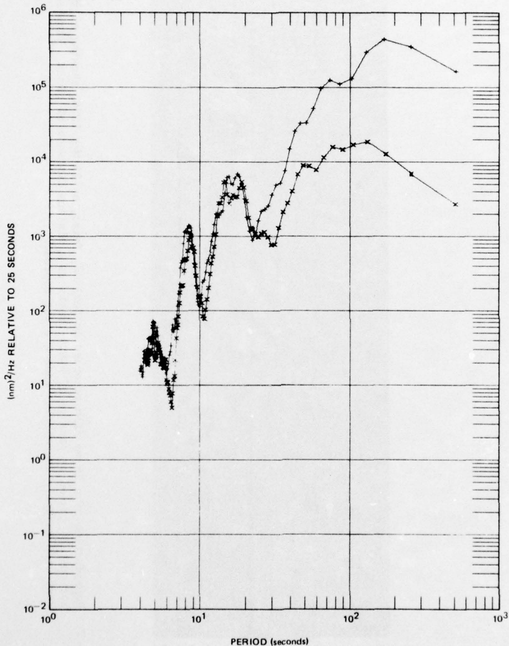
Figure 8. Power spectra of the background noise recorded by the long-period horizontal north (LPN) seismograph showing a significant decrease in level with decreased cultural activity during the night. Not corrected for instrument response
