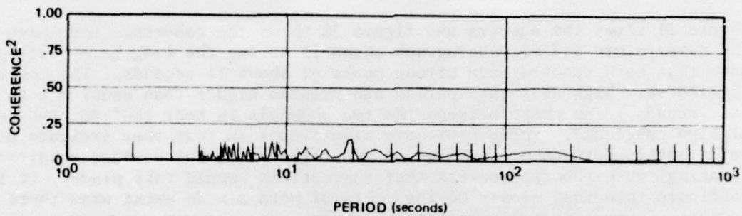
Figure 30a. Coherence squared between LPN and the temperature (Delta T) channel when heat was being dissipated in heater No. 2
