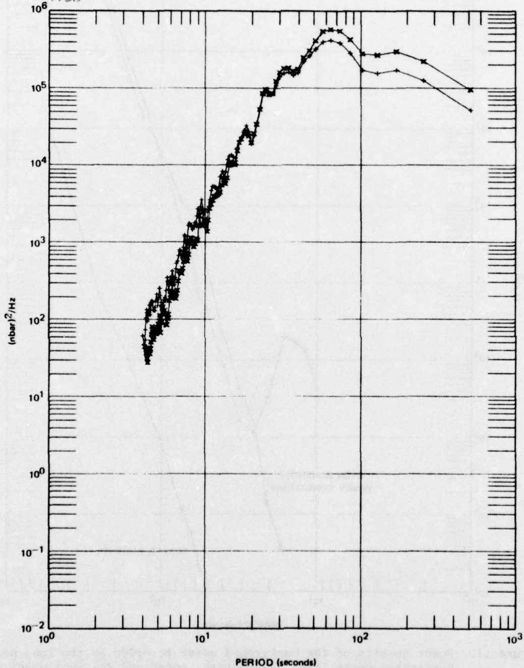
Figure 12. Power spectra of internal pressure noise in the sealed bore-hole as sensed by MKBTOP at the top of the well and by MKBBOT at 60 m depth. Not corrected for instrument response
