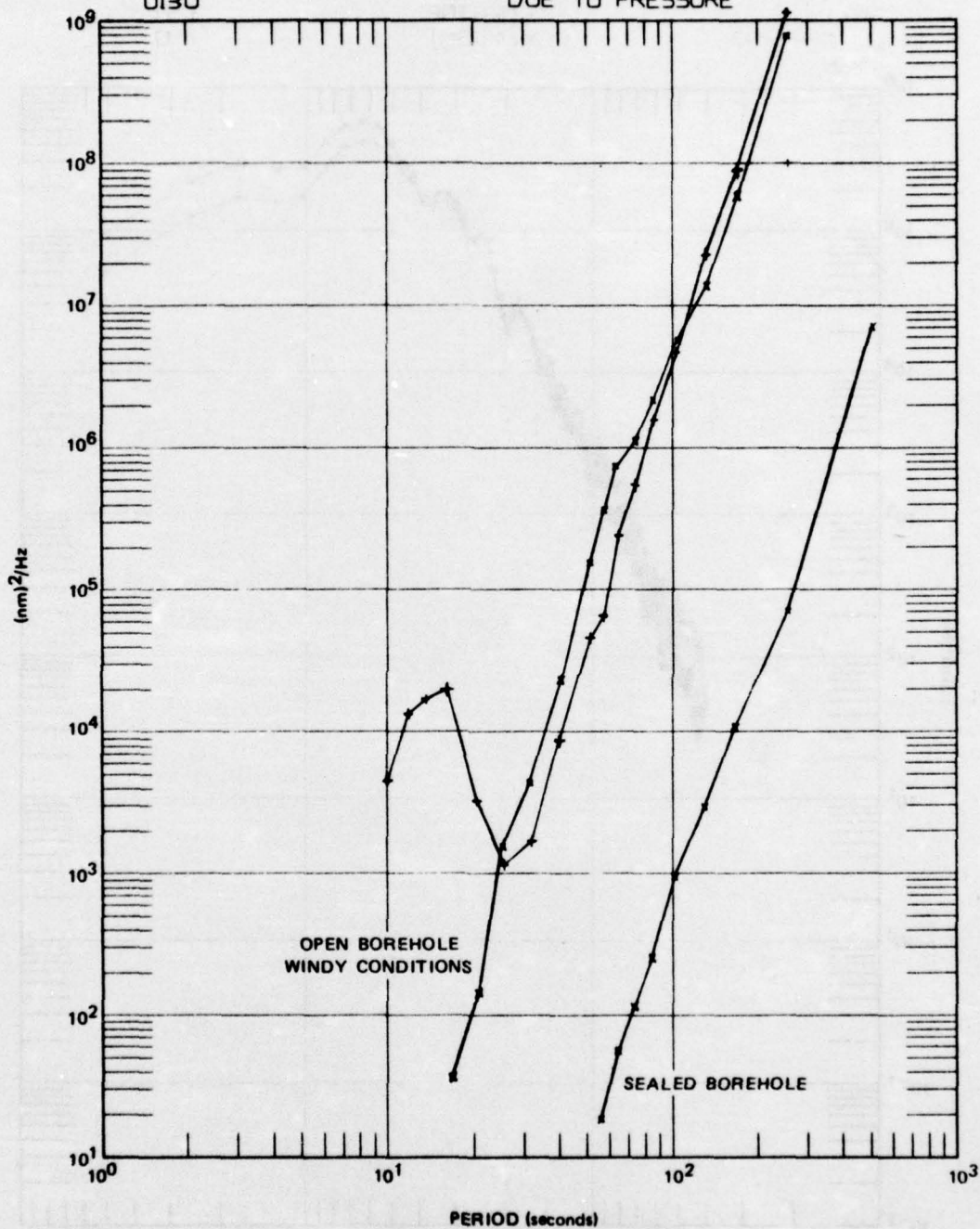
Figure 11. Power spectra of the background noise recorded by the long-period horizontal north (LPN) seismograph, corrected for instrument response. Also shown is the theoretically predicted noise contribution due to borehole pressure changes
