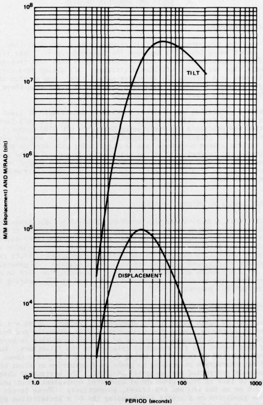
Figure 5. Response of horizontal KS seismographs to displacement and tilt
