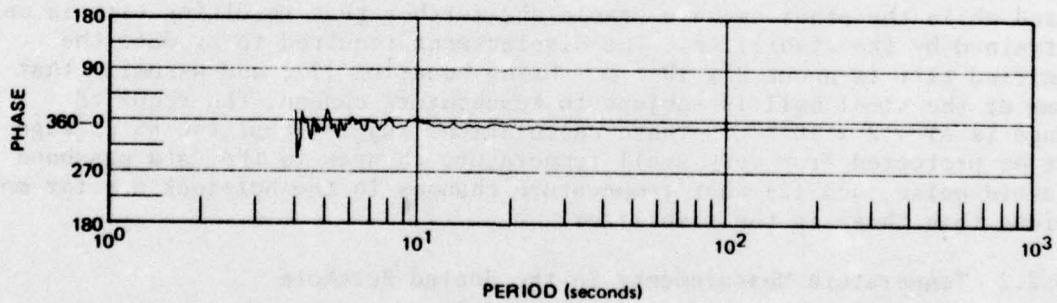
Figure 13. Coherence squared (a) and phase (b) between MKBTOP and MKBBOT when the instruments were separated by 60 m
