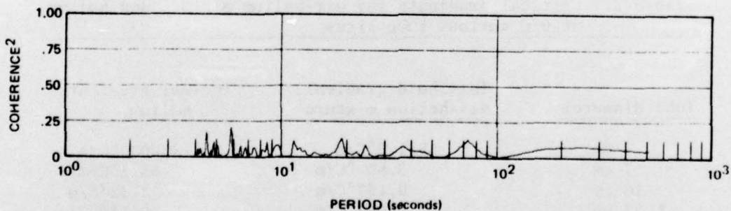
Figure 30b. Coherence squared between LPN and the microbarograph when heat was being dissipated in heater No. 2
