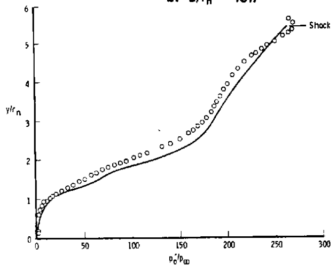
Figure 13. Blunt biconic lee-side pitot pressure profiles.
