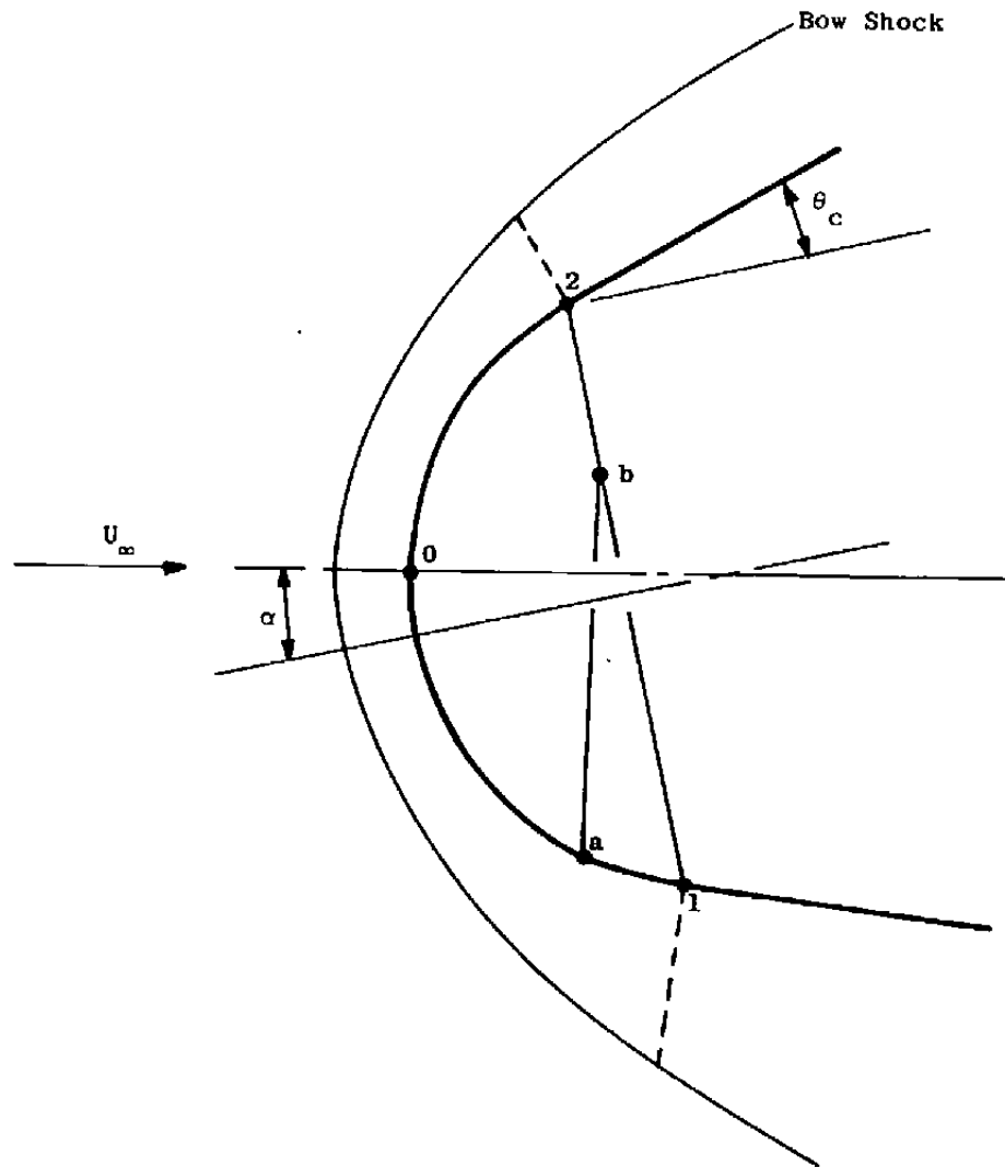
Figure 2. Treatment of nose cap flow to yield initial HVSL starting data.
