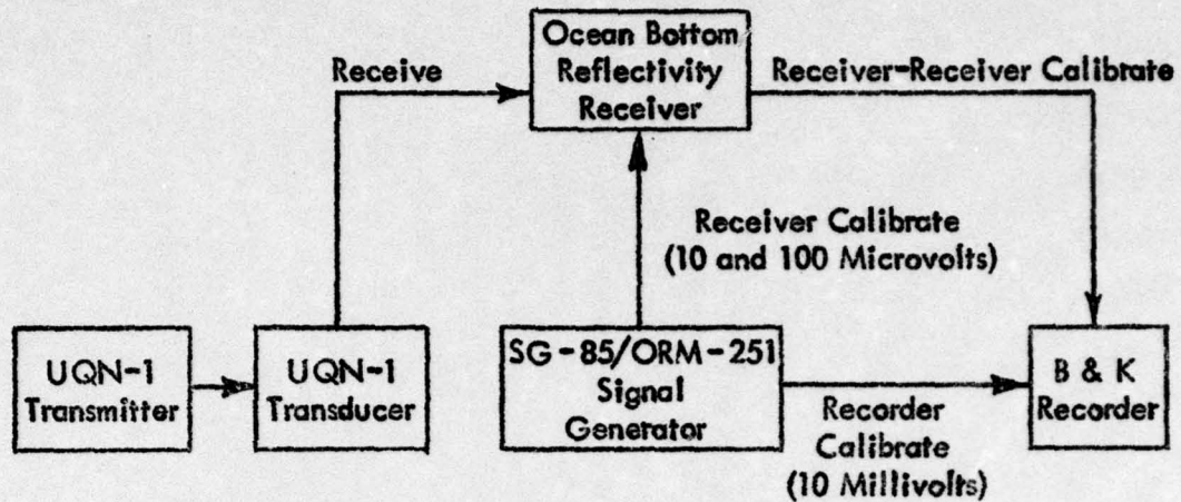
FIGURE 3 BLOCK DIAGRAM OF MODIFIED REMPAC SYSTEM
