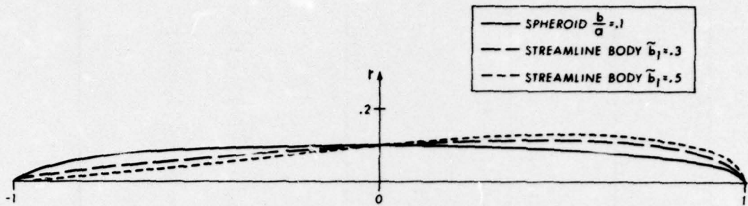
Fig. 2 - Meridian Profiles
