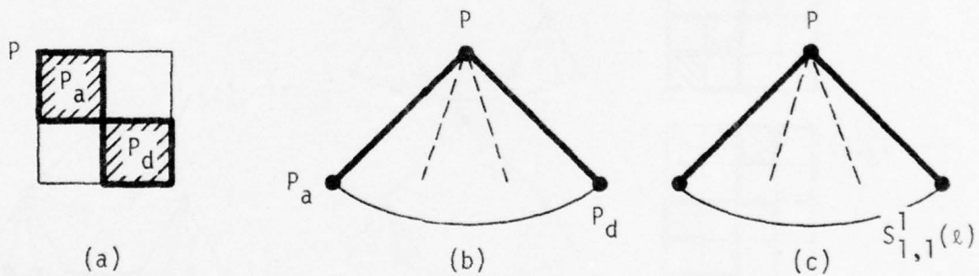
Fig. 3.14: Left-diagonal Symmetry Class at Level 1. (a) The Paired Grid-points (Shaded Squares); (b) The Corresponding Paired Nodes of the Tree (Solid Lines); (c) The \ell -class.
