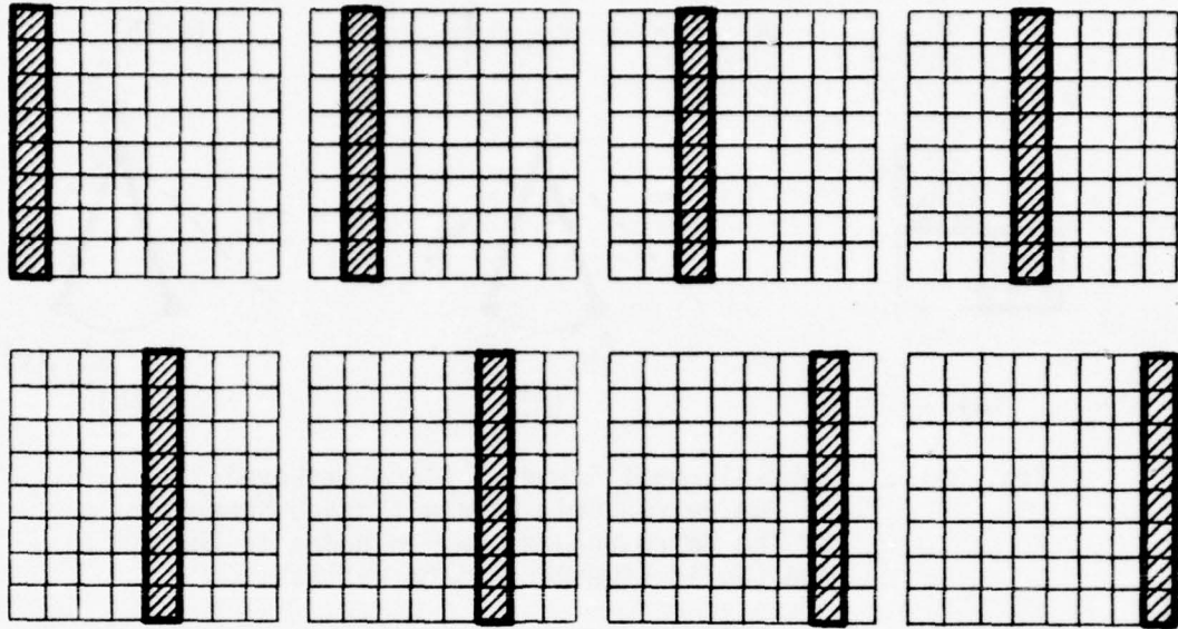
Fig. 3.10: Vertical Symmetry Classes at Level 3. The Shaded Squares Identify the Eight Different Sets.
