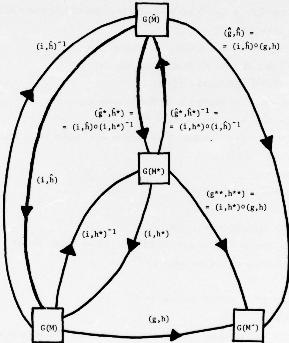
Figure 1.7.3: Relations among the Maps of the Minimal Standard Cover Concept.
