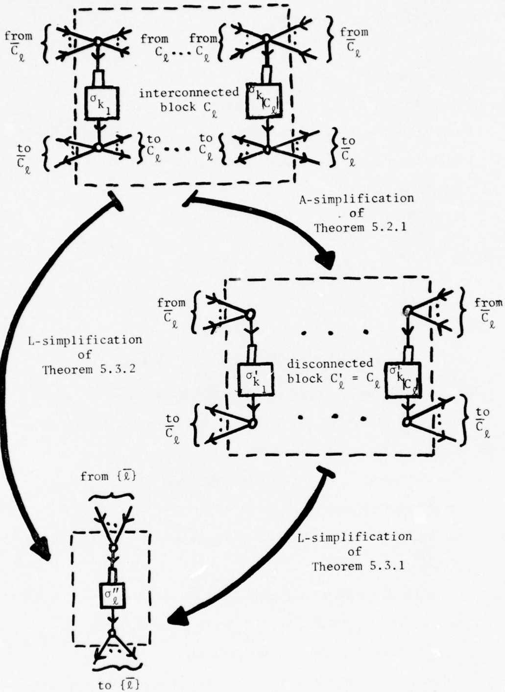
Figure 5.3.1: A Decomposition of the L-Simplification of Theorem 5.3.2 When Operating on a Typical Block C_l .
