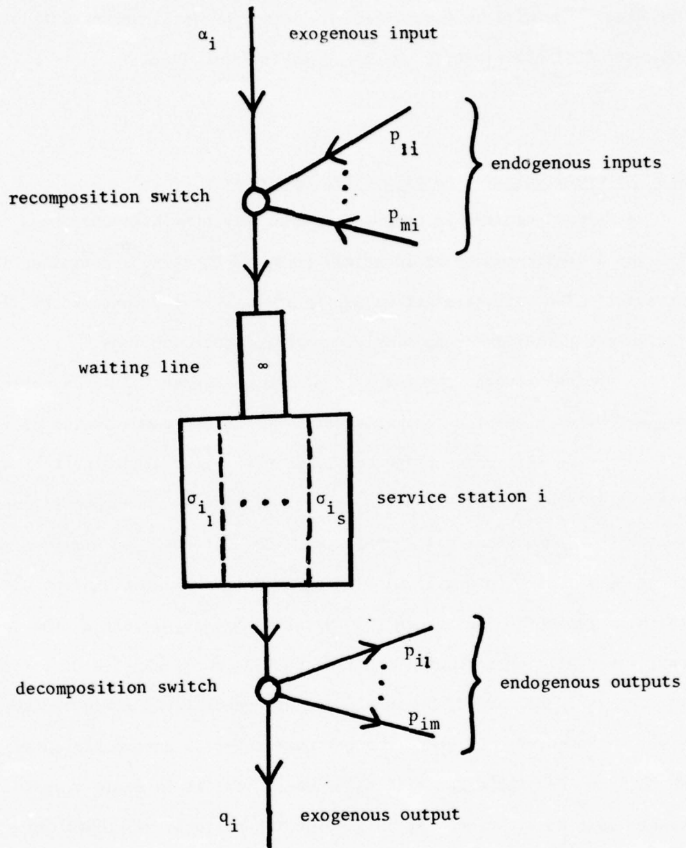
Figure 4.1.1: Typical Node i in a Jackson Network with Multiple Server Nodes.
