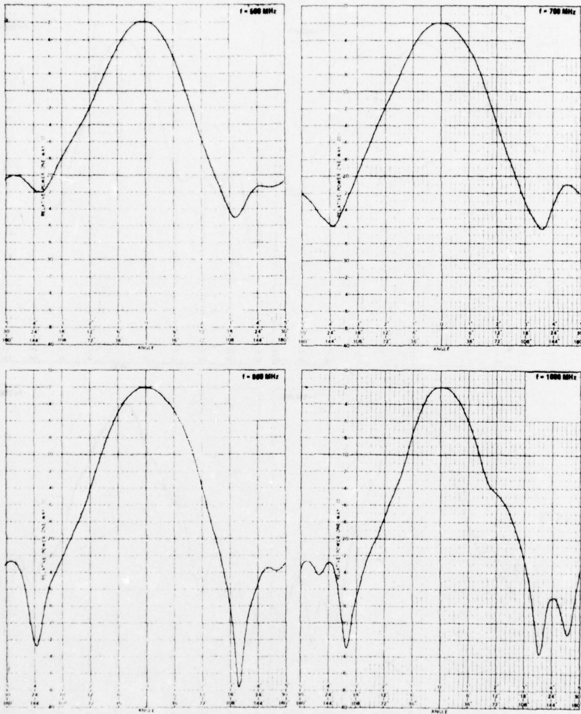
Figure 35. E0 Patterns for 8-1/2 Inch Hooded Antenna, One Meter Spacing, 500-1000 MHz.
