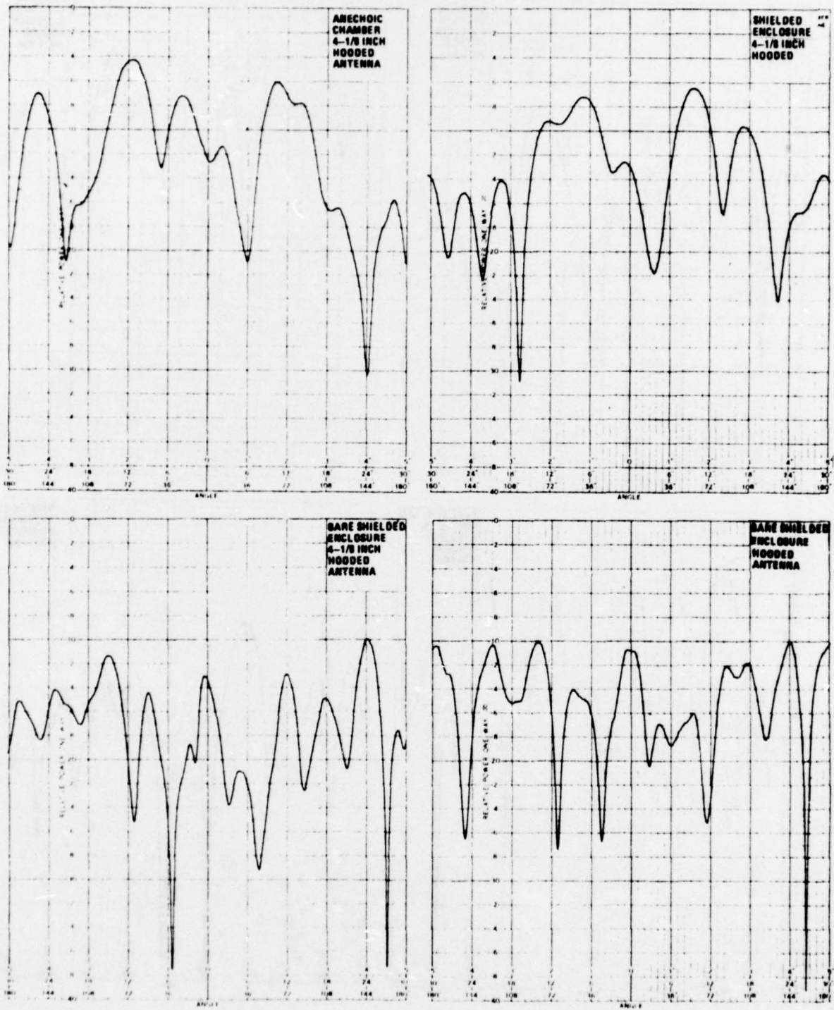
Figure 31. Simulated Equipment Patterns for Various Test Configurations, 800 MHz.
