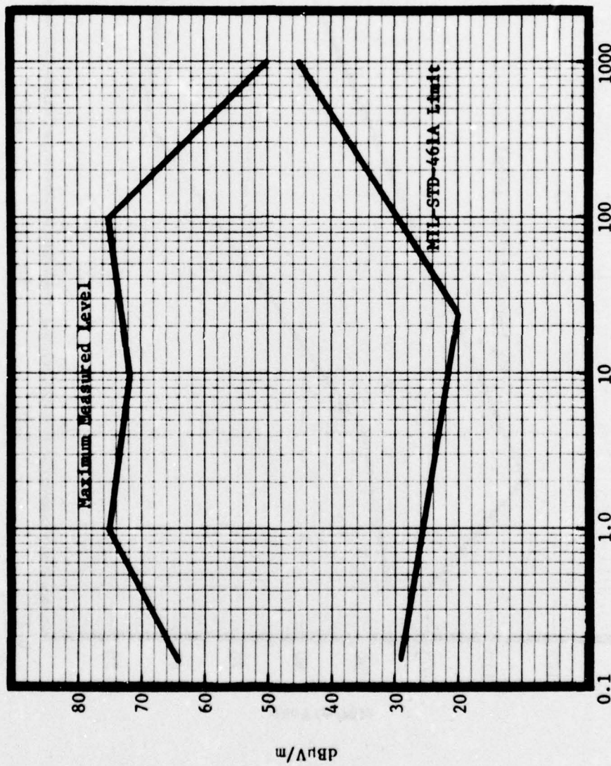
Figure 50. Narrowband Emission Levels Measured in ARTCC Facilities.
