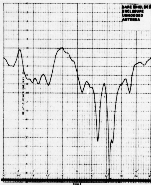
Figure 29. Dipole Patterns for Various Test Configurations, 1000 MHz.
