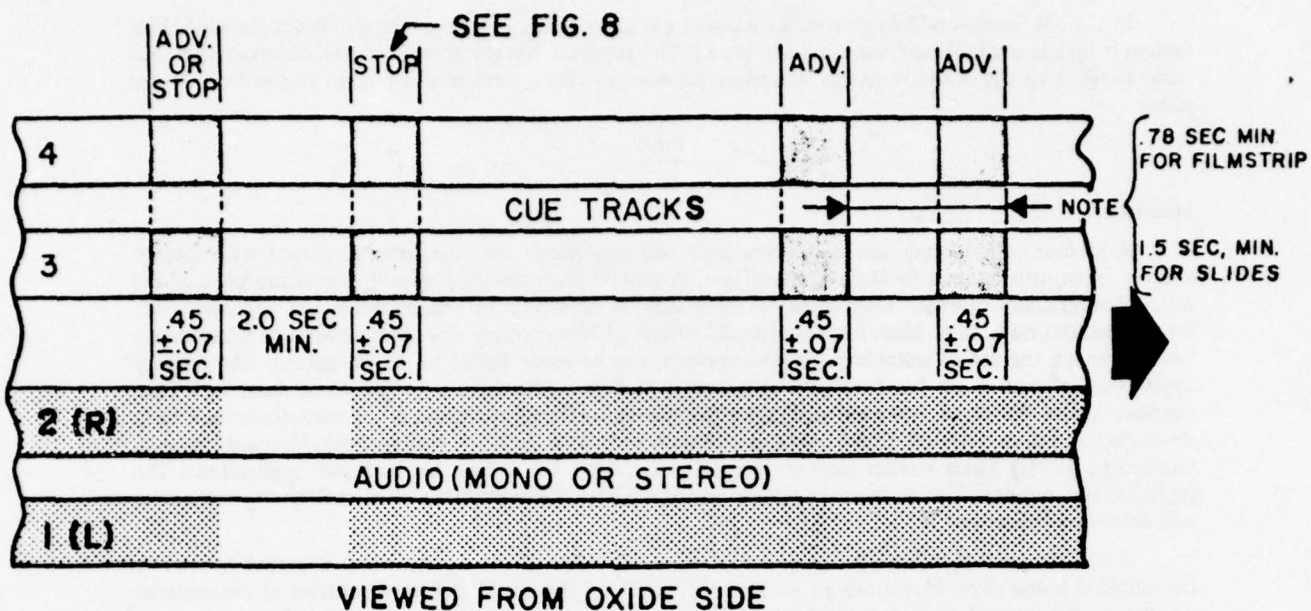
Figure 9. Cue duration and spacing, separate track system, slide and filmstrip (taken from PH 7.4 proposal, 1974).
