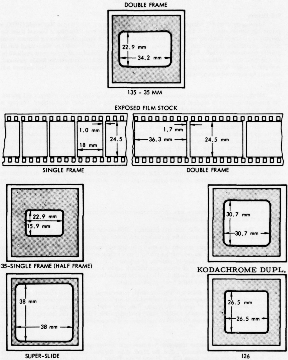
Figure 1. 2-inch slide formats (taken from Sullivan and Smith, 1974).
