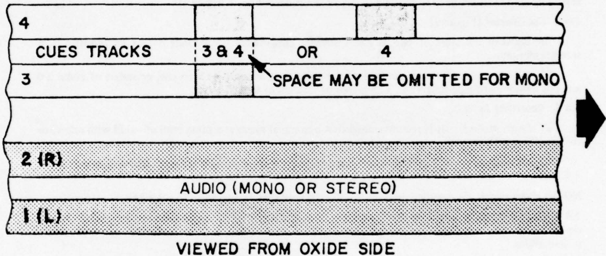
Figure 8. Track utilization separate track system (taken from PH 7.4 proposal, 1974).
