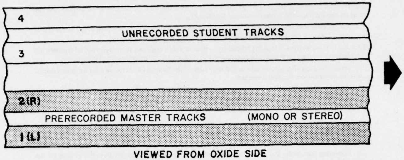
Figure 3. Track utilization, learning laboratories (taken from PH 7.4 proposal, 1974).
