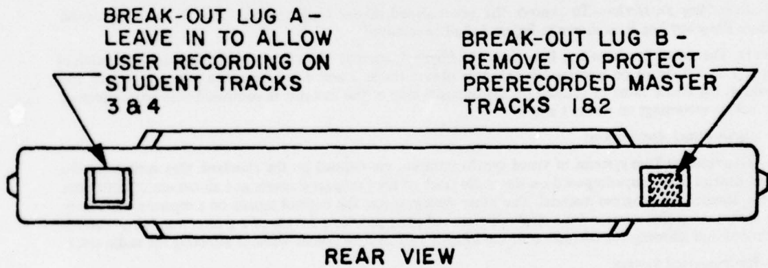
Figure 4. Recording protection, learning laboratories (taken from PH 7.4 proposal, 1974).
