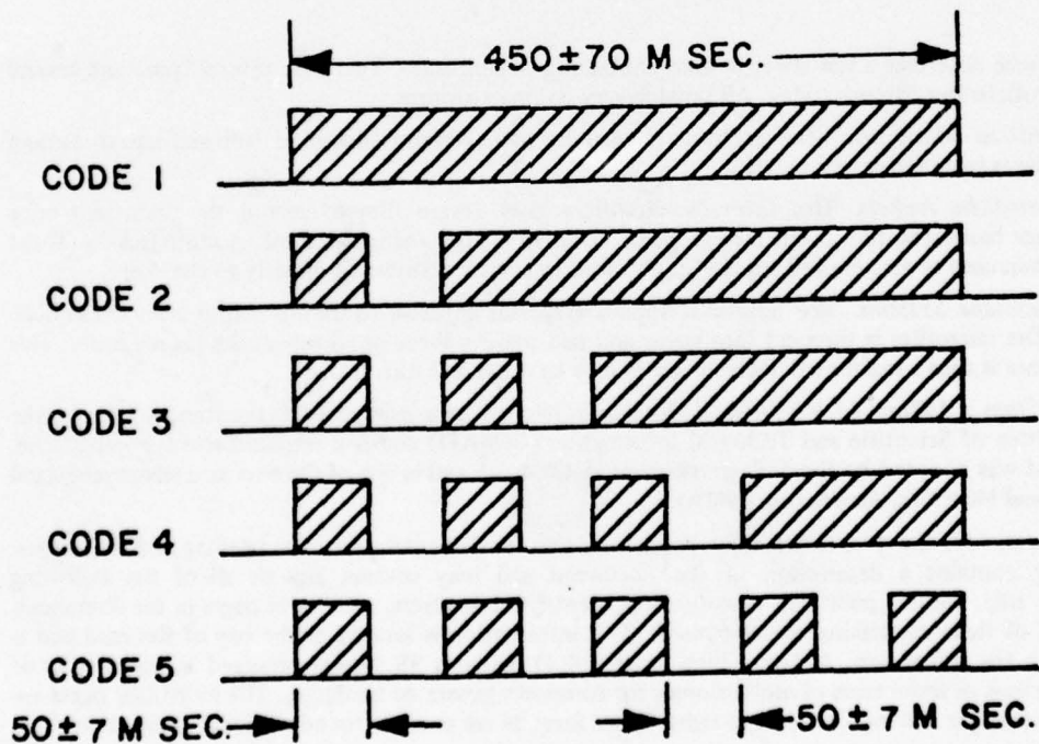
Figure 10. Correct answer coding for stop cue (taken from PH 7.4 proposal, 1974).
