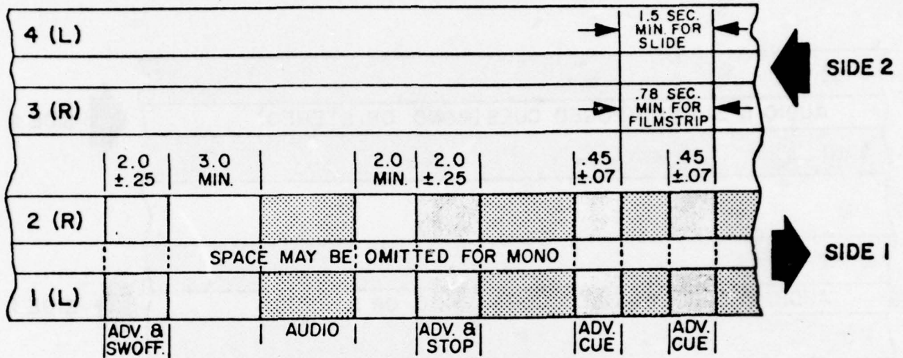
VIEWED FROM OXIDE SIDE
