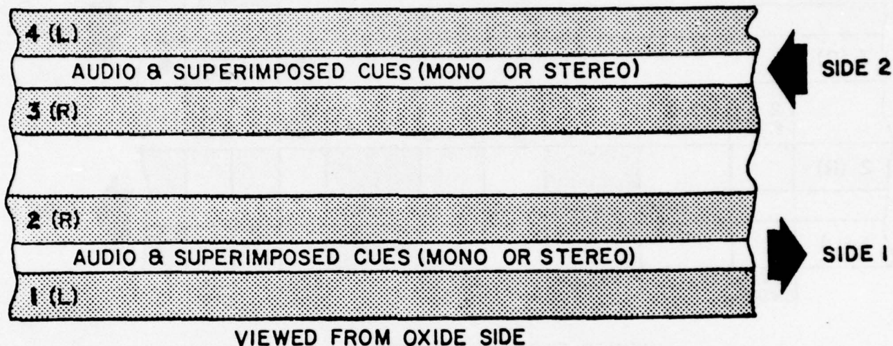
Figure 5. Track utilization, superimposed system (taken from PH 7.4 proposal, 1974).
