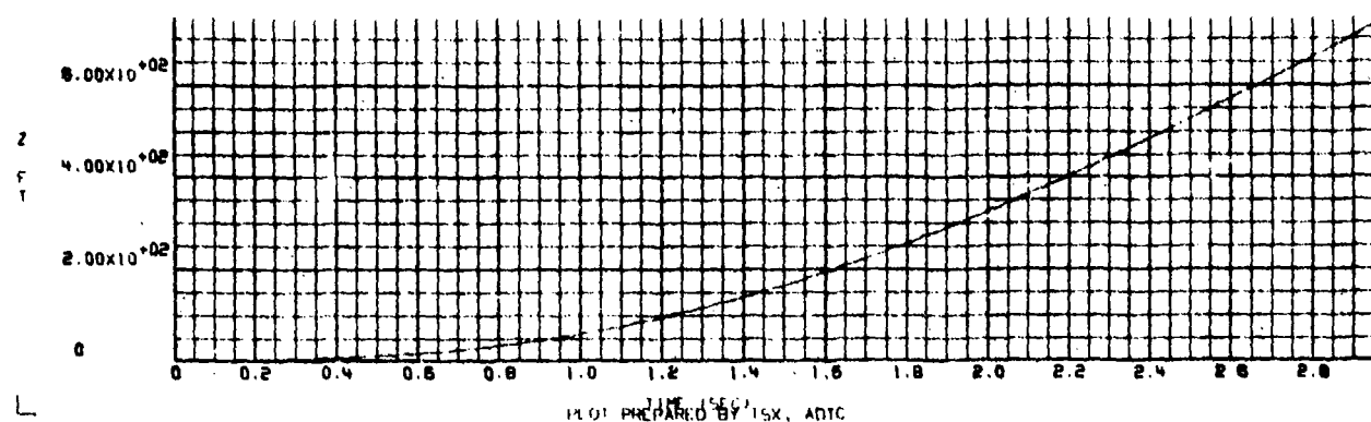
Figure C-3. X, Y, and Z Position Versus Time for a Flow Field Intensity of 1 (as measured in the wind tunnel)
