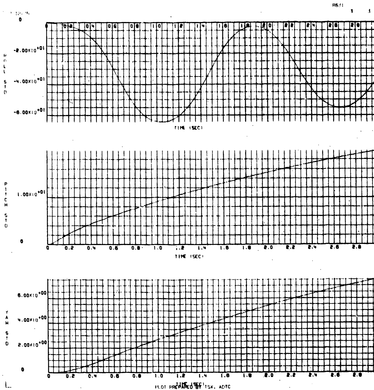
Figure E-2. \phi , \theta , and \psi Rotation Versus Time for a Flow Field Intensity of 1/2
