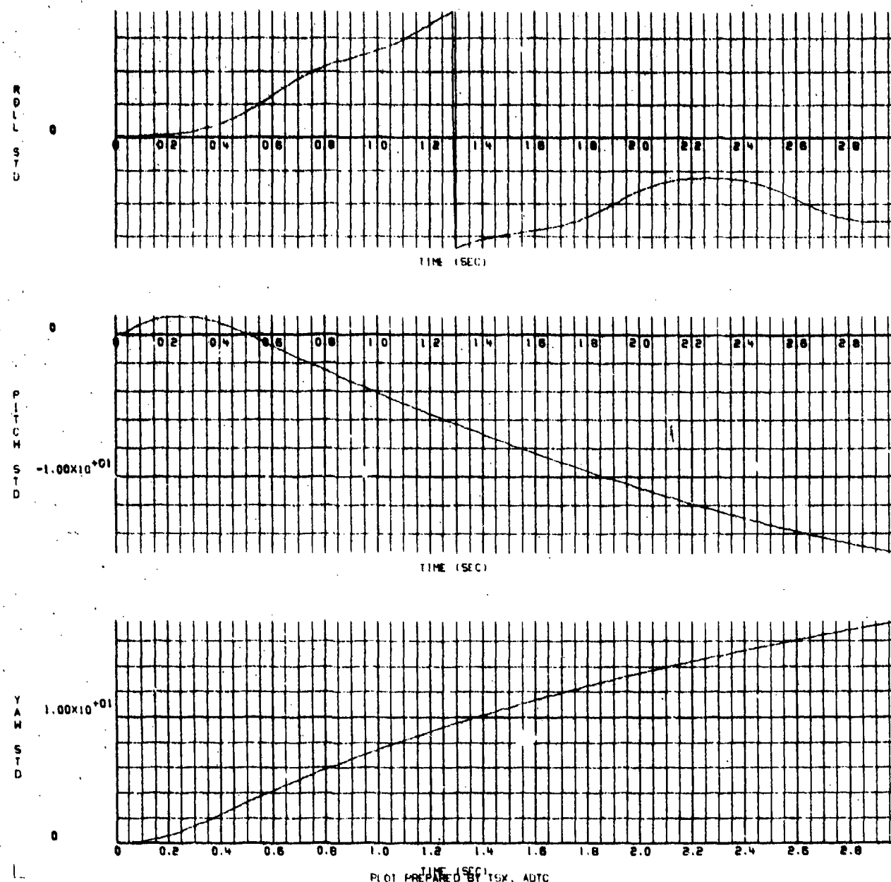
Figure H-4. \phi , \theta , and \psi Rotation Versus Time for a Flow Field Intensity of 1 (unchanged from the wind tunnel measured values)
