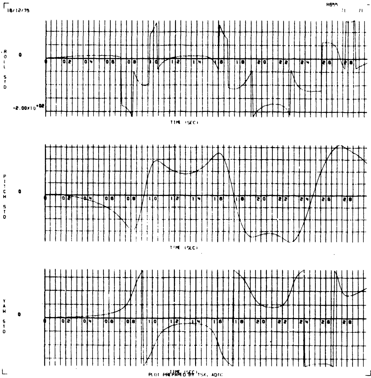
Figure X-6. \phi , \theta , and \psi Rotation Versus Time for a Flow Field Intensity of 2
