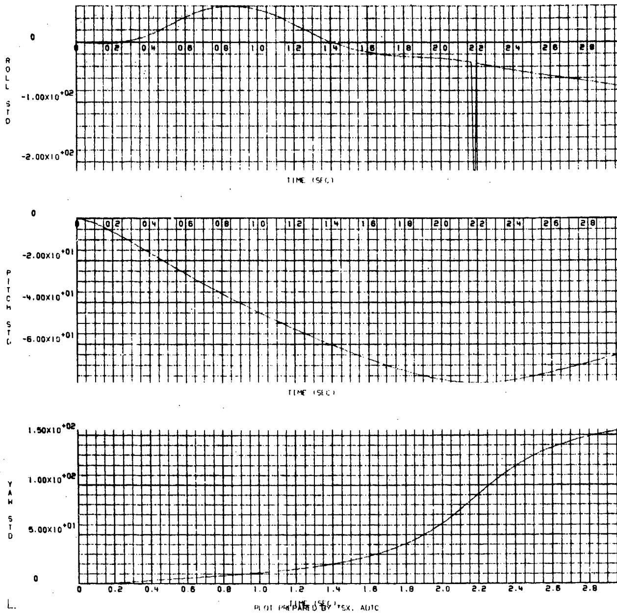
Figure B-6. \phi , \theta , and \psi Rotation Versus Time for a Flow Field Intensity of 2
