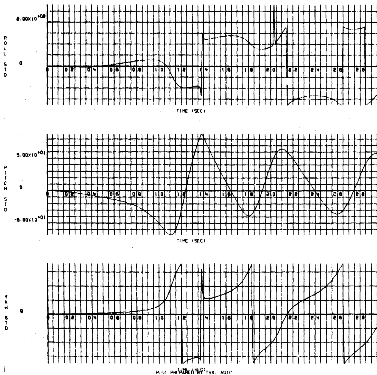
Figure N-4. \phi , \theta , and \psi Rotation Versus Time for a Flow Field Intensity of 1 (unchanged from the wind tunnel measured values)
