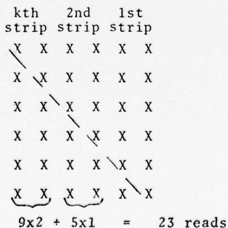
Figure 1. Counting reads in a factorization
