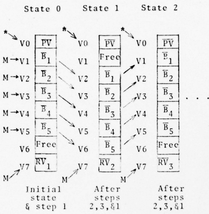
Figure 6a. Data flow in external block processing
