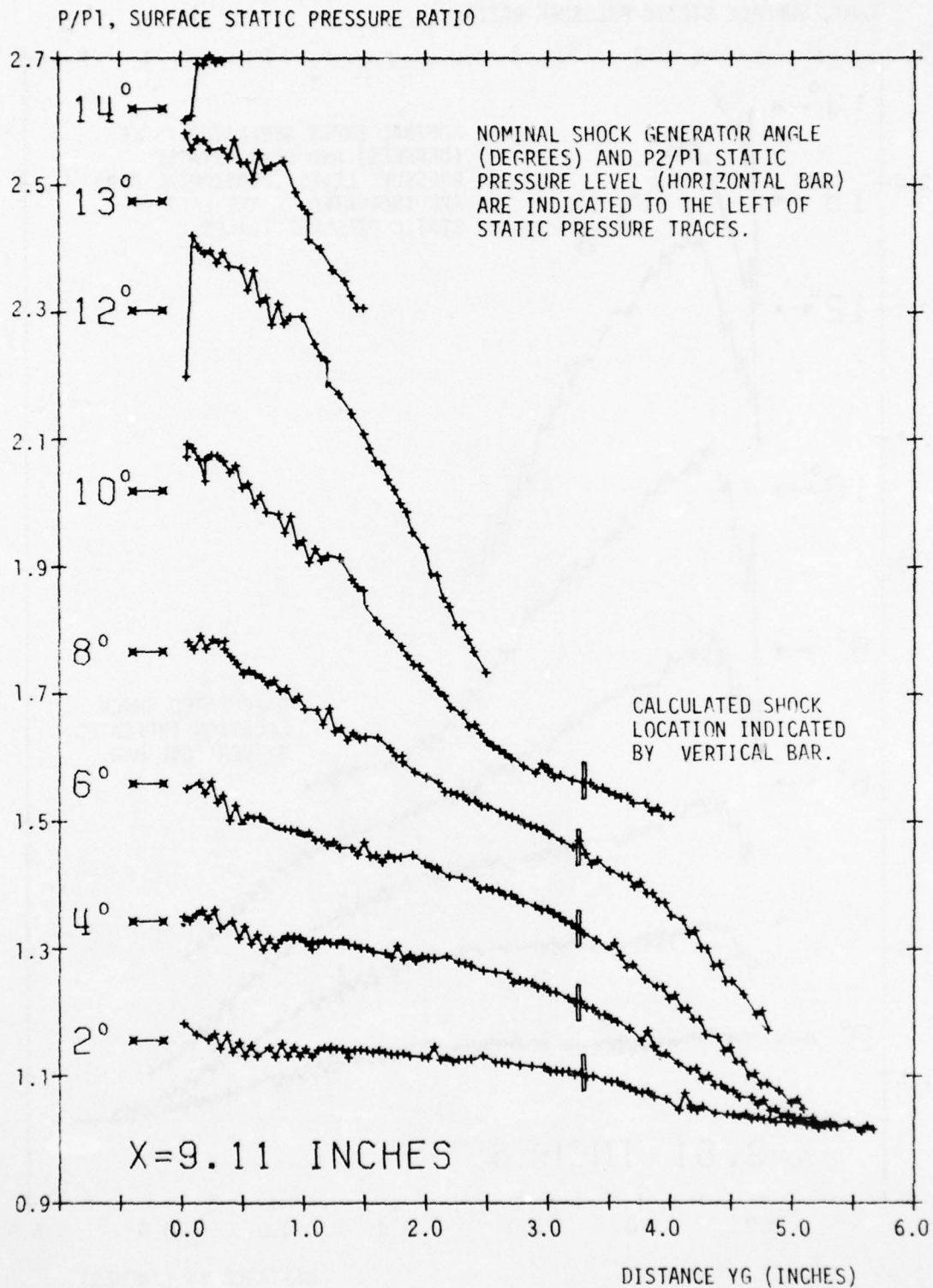
Figure A-8: Surface Static Pressure, X ≈ 9.1 inches.
