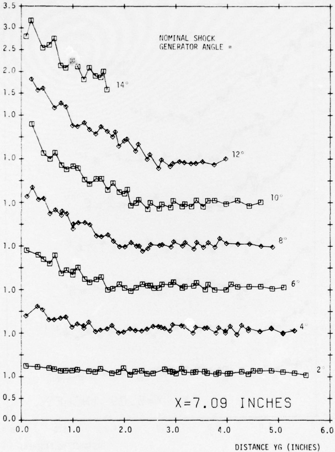
Figure C-3: Surface Heat Transfer, X = 7.1 inches.
