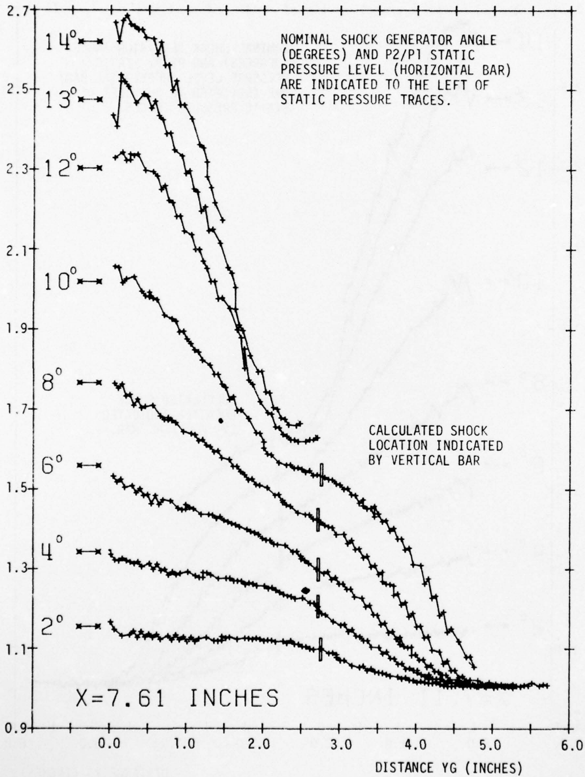
Figure A-5: Surface Static Pressure, X = 7.6 inches.
