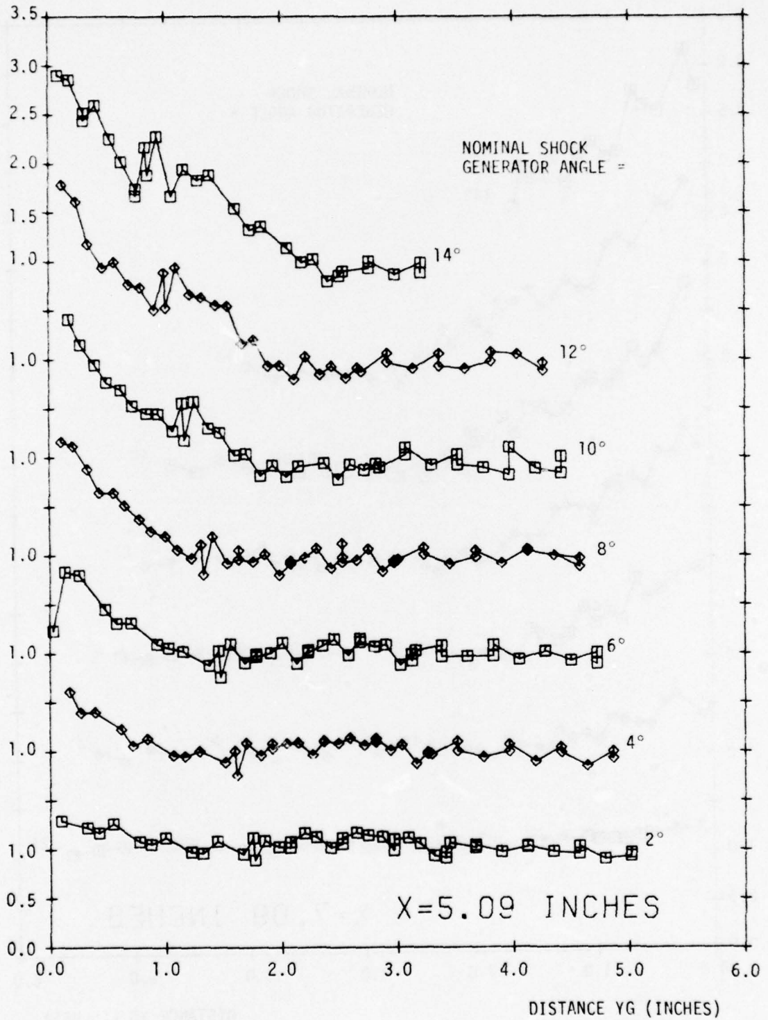
Figure C-2: Surface Heat Transfer, X = 5.1 inches.
