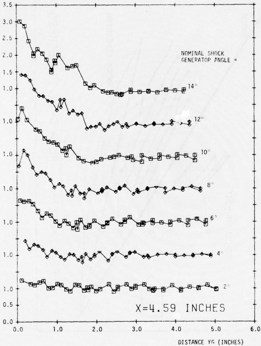
Figure C-1: Surface Heat Transfer, X = 4.6 inches.
