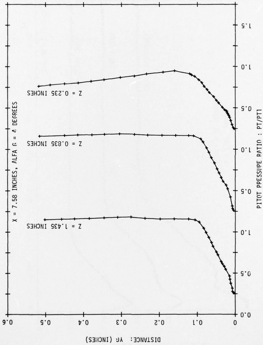
Figure I-1: Pitot Pressure Surveys, X = 7.6 inches, \alpha_G = 4^\circ .
