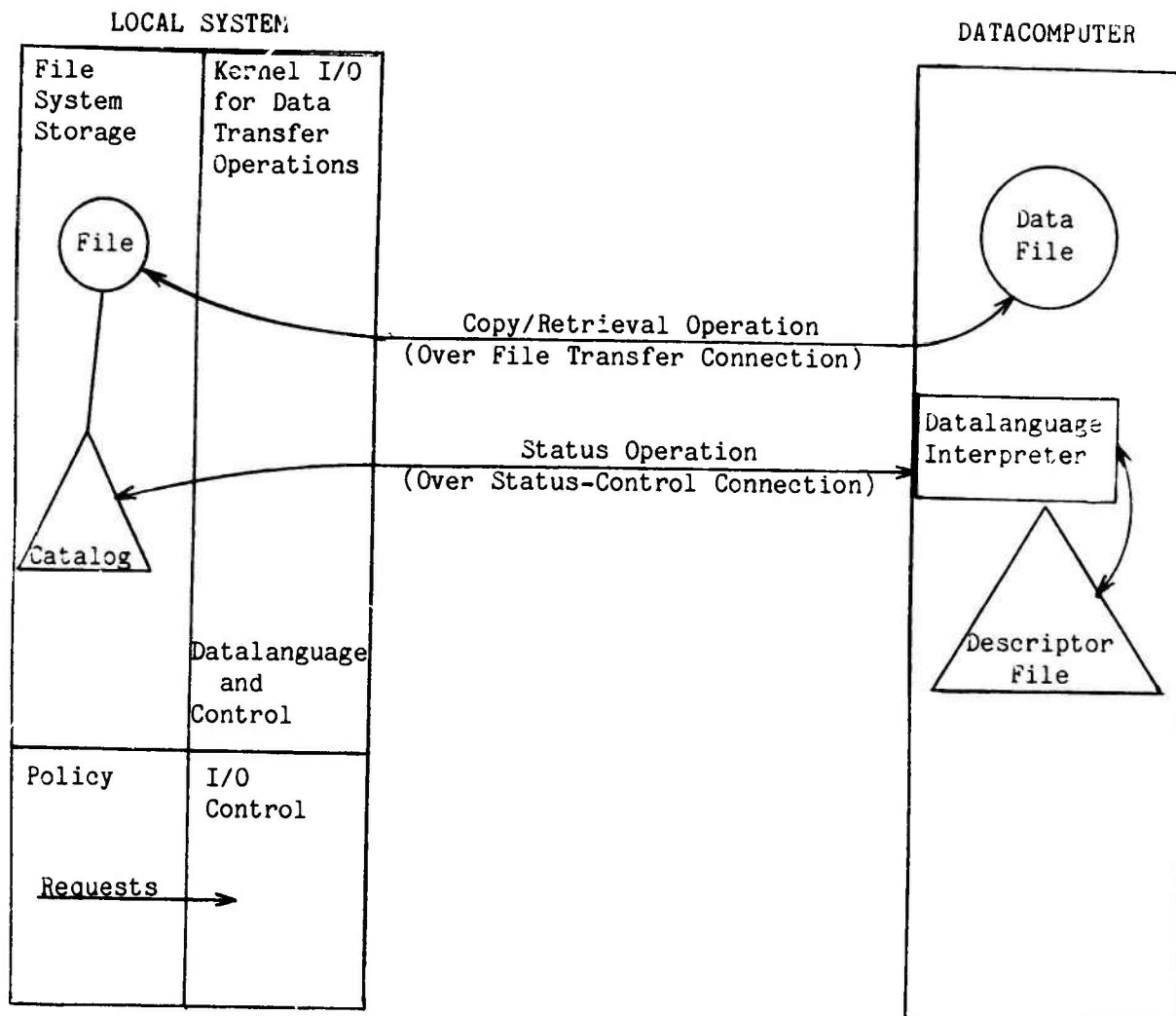
Figure 4.5 I/O Control of Data Transfers
