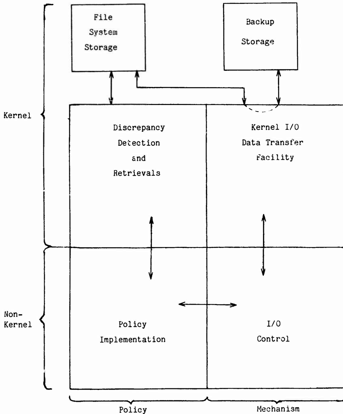
Figure 4.1 Interacting Components in the Backup System Design
