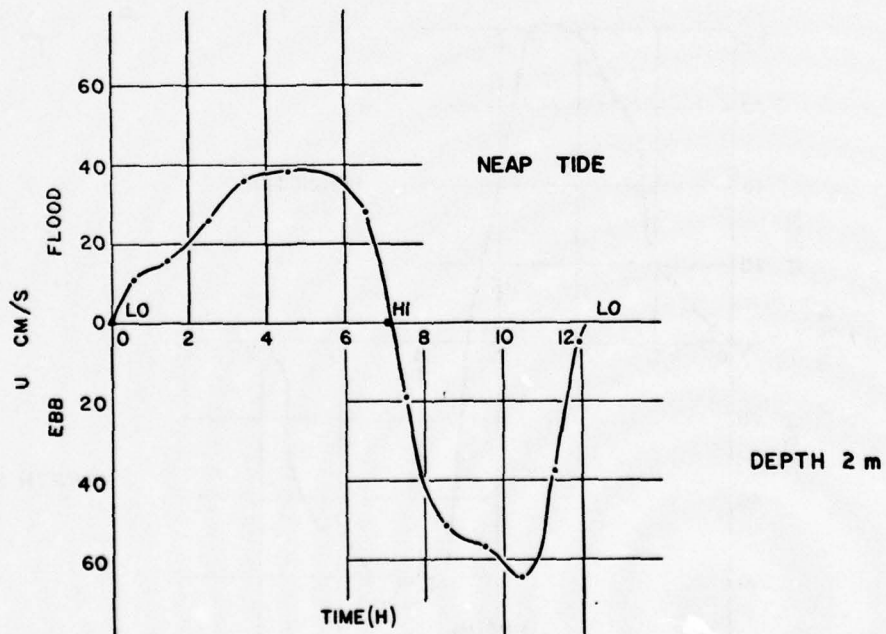
Figure C-4. Tidal current velocity, station IN-2, 18 July 1972.
