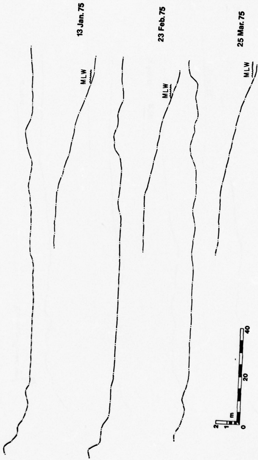
Figure B-16. Station NI-10, 13 January to 25 March 1975.
