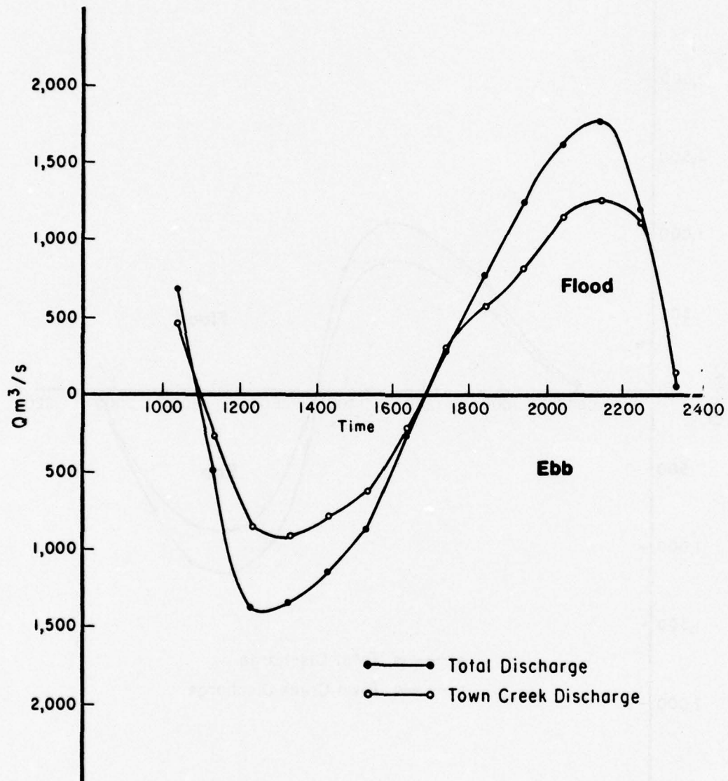
Figure D-5. North Inlet discharge, 15 September 1974.
