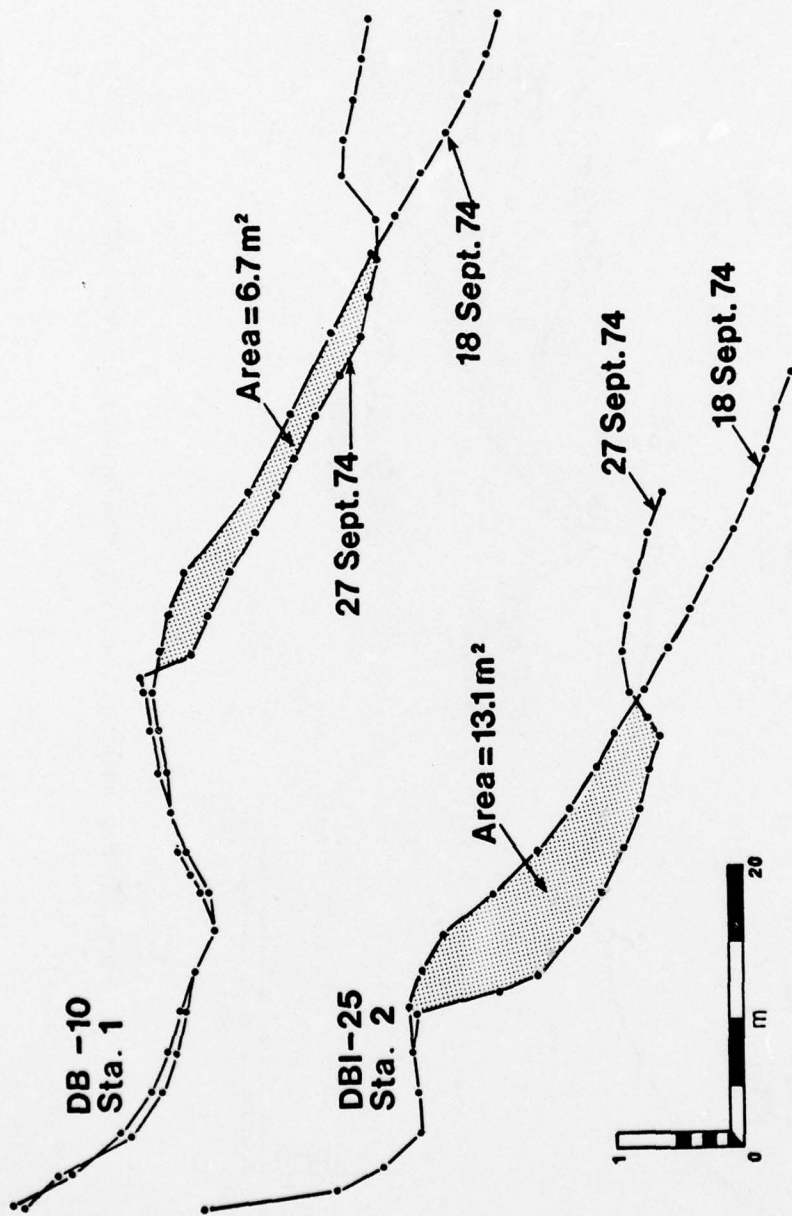
Figure 36. Debidue Island beach erosion, September 1974.
