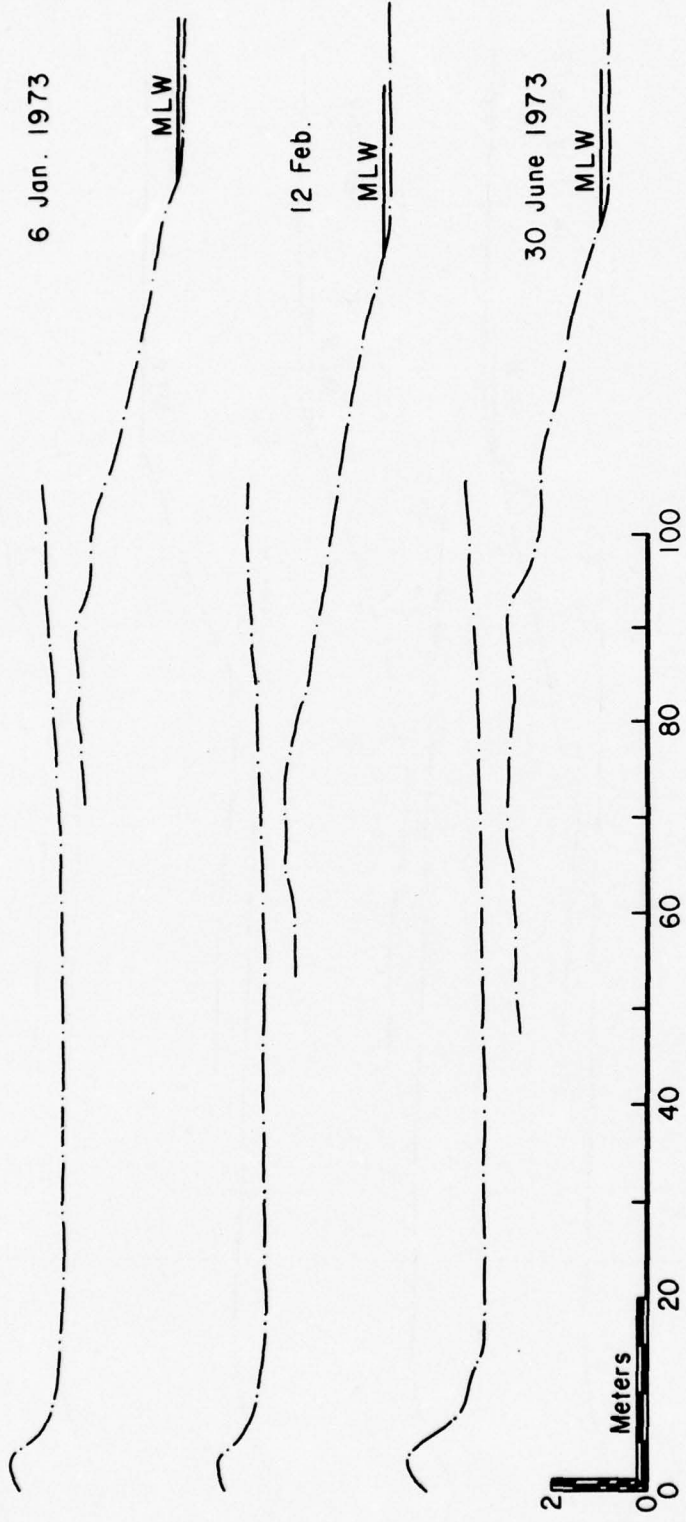
Figure A-9. Station NL-10, 6 January to 30 June 1973.
