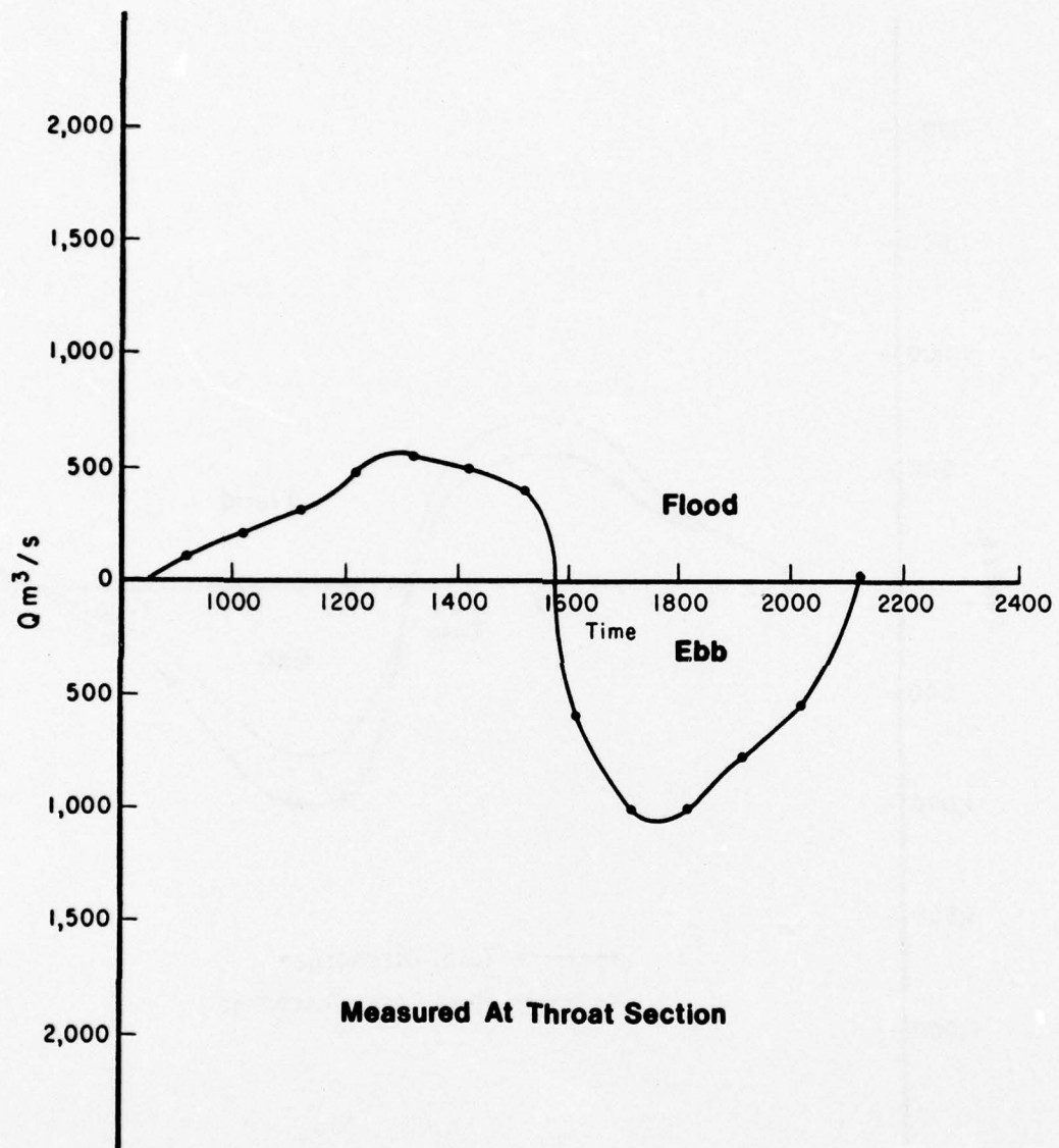
Figure D-14. North Inlet discharge, 21 March 1975.
