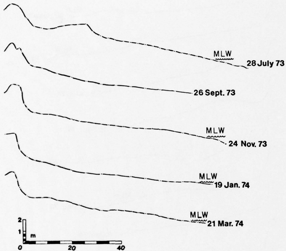
Figure B-9. Station DBI-25, 28 July 1974 to 21 March 1974.
