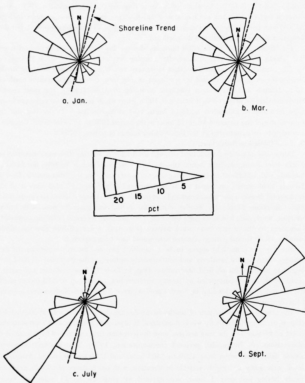
Figure 4. Quarterly wind directional frequency, offshore South Carolina (based on U.S. Naval Weather Service Command, 1970).
