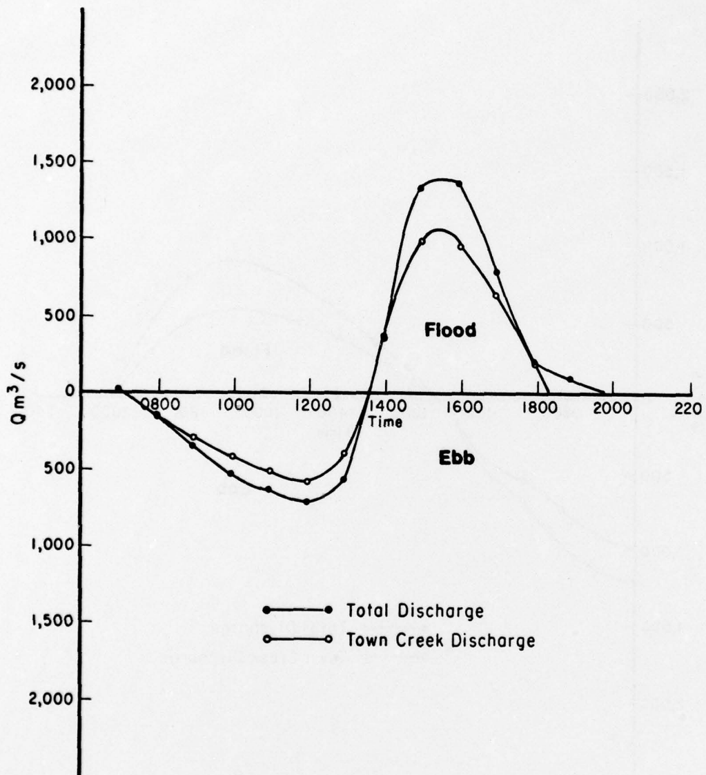
Figure D-9. North Inlet discharge, 4 January 1975.
