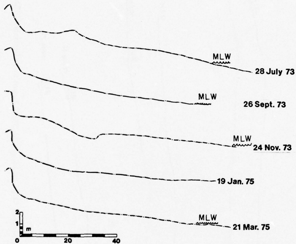
Figure B-6. Station DBI-20, 28 July 1973 to 21 March 1974.
