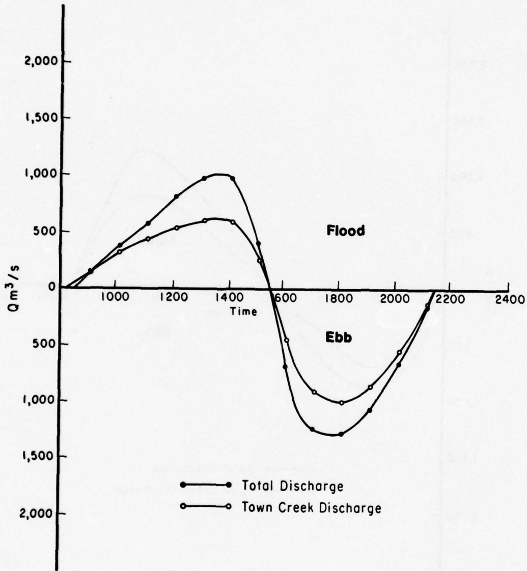
Figure D-6. North Inlet discharge, 21 September 1974.
