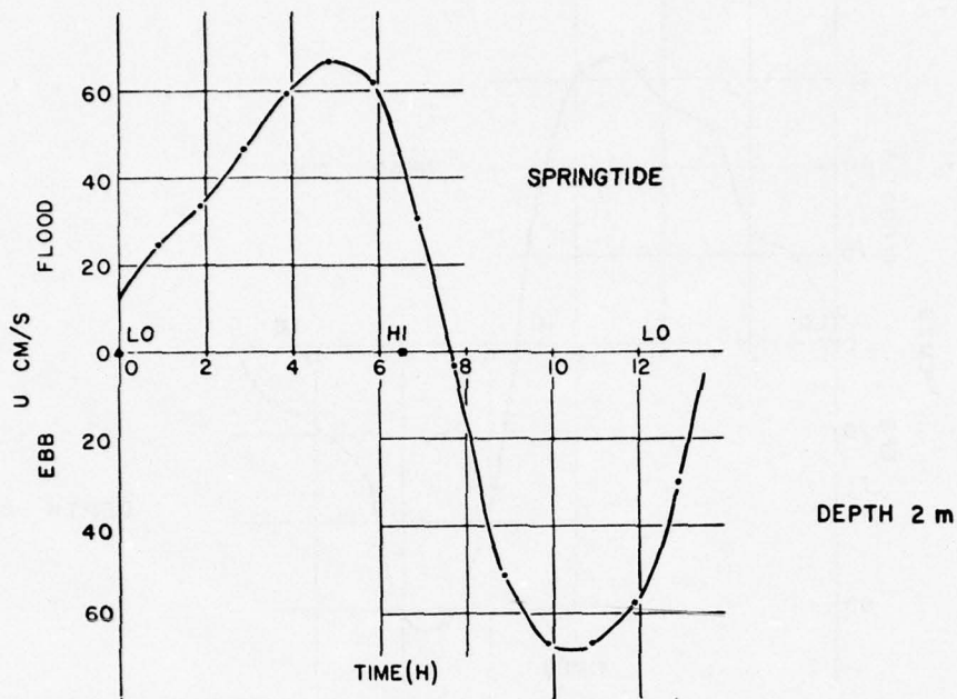
Figure C-11. Tidal current velocity, station TC-4, 6 August 1972.
