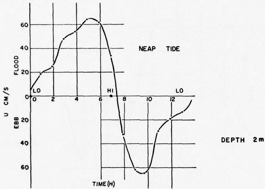
Figure C-13. Tidal current velocity, station JC-2, 20 July 1972.
