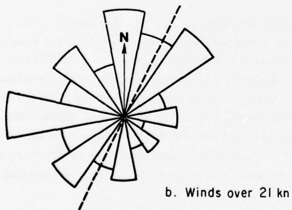
Figure 3. Annual wind directional frequency, offshore South Carolina (based on U.S. Naval Weather Service Command, 1970).
