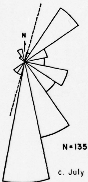
Figure 6. Observed wind directional distribution, North Inlet.
