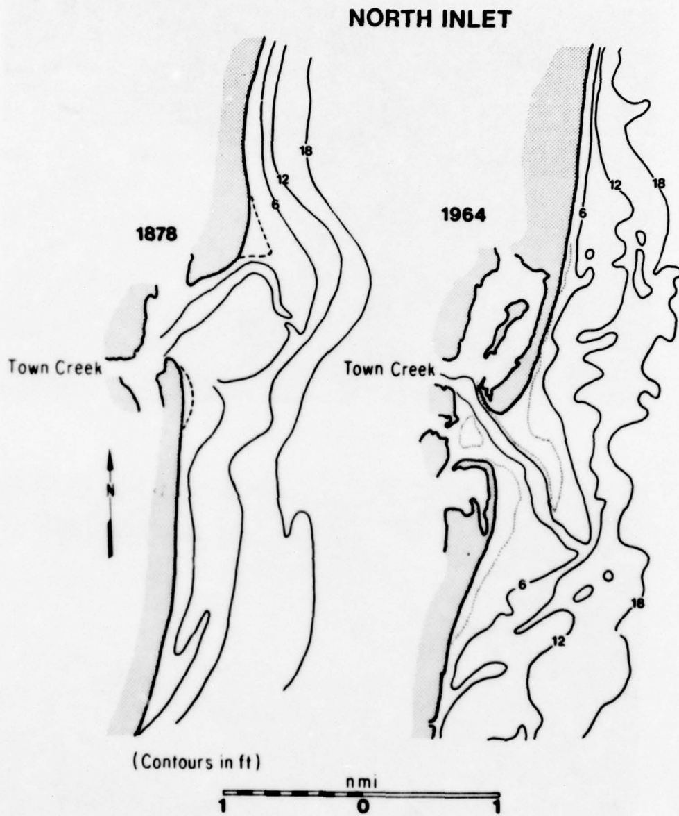
Figure 43. North Inlet offshore bathymetry, 1878 and 1964.
