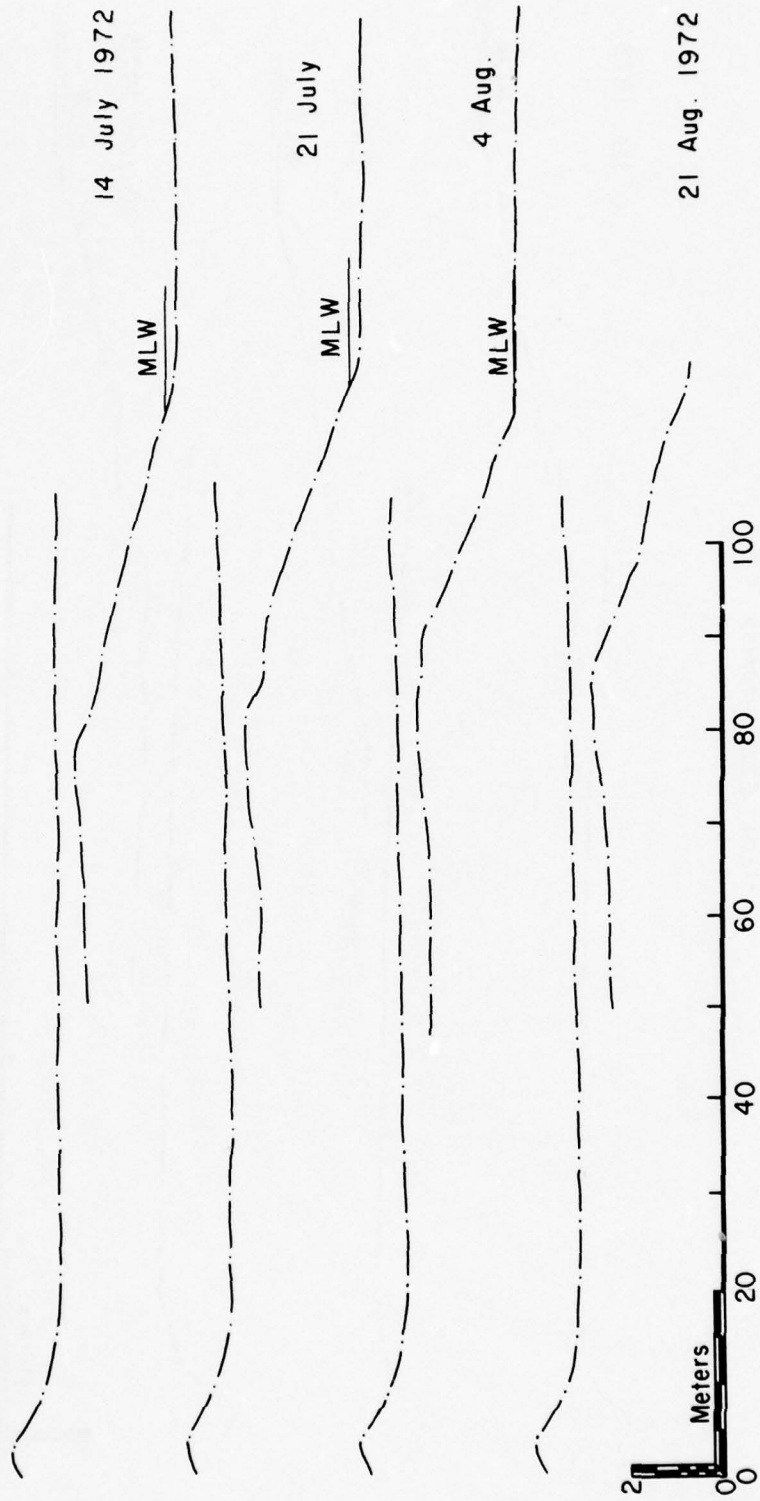
Figure A-8. Station NI-10, 14 July to 21 August 1972.
