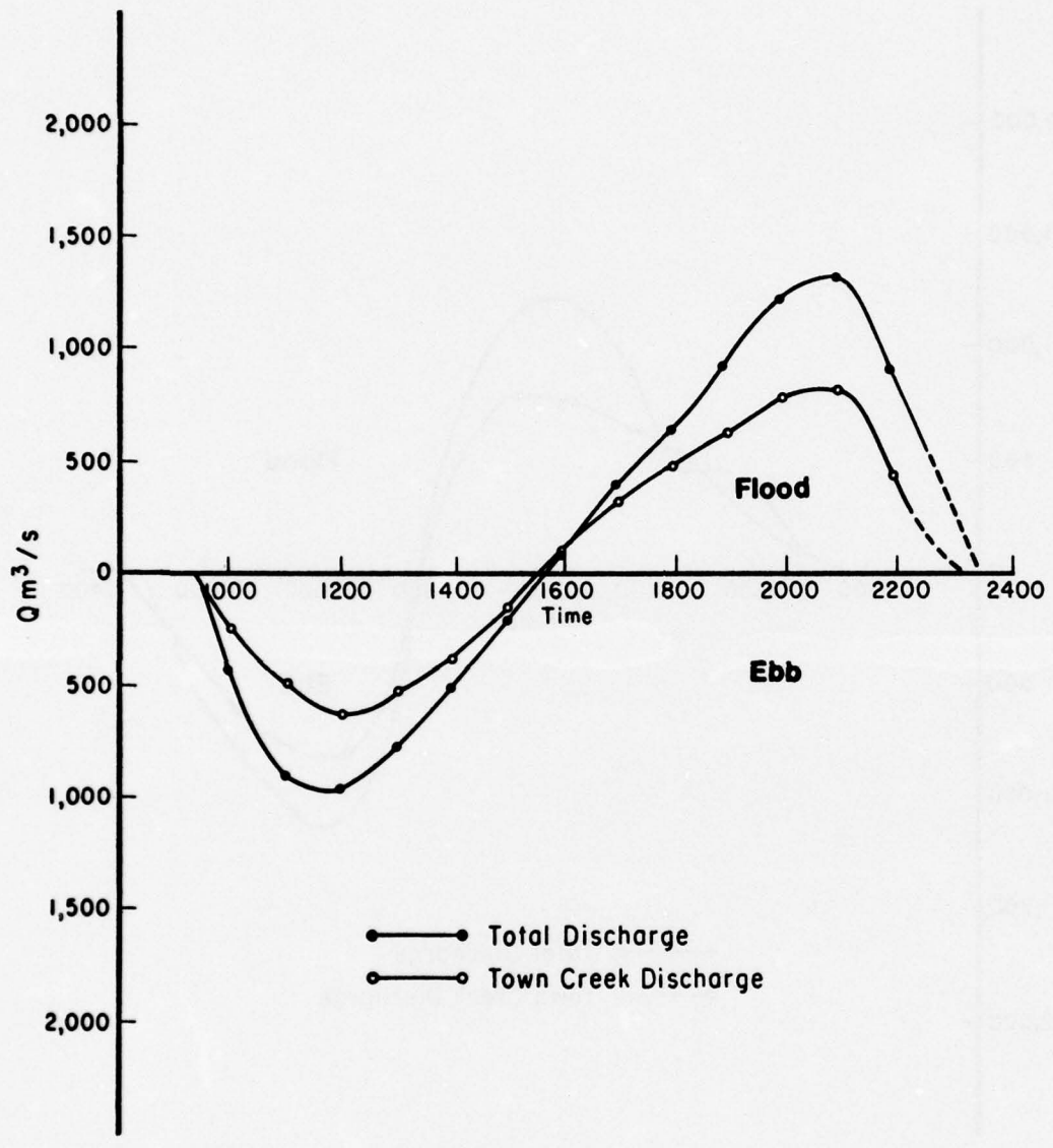
Figure D-3. North Inlet discharge, 1 August 1974.
