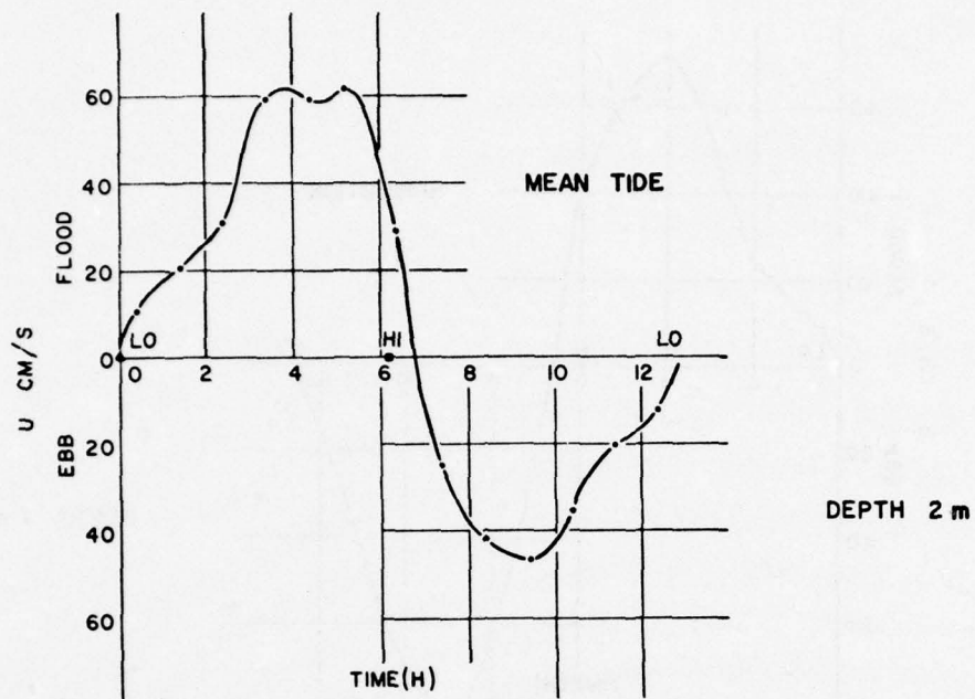
Figure C-3. Tidal current velocity, station IN-2, 25 July 1972.
