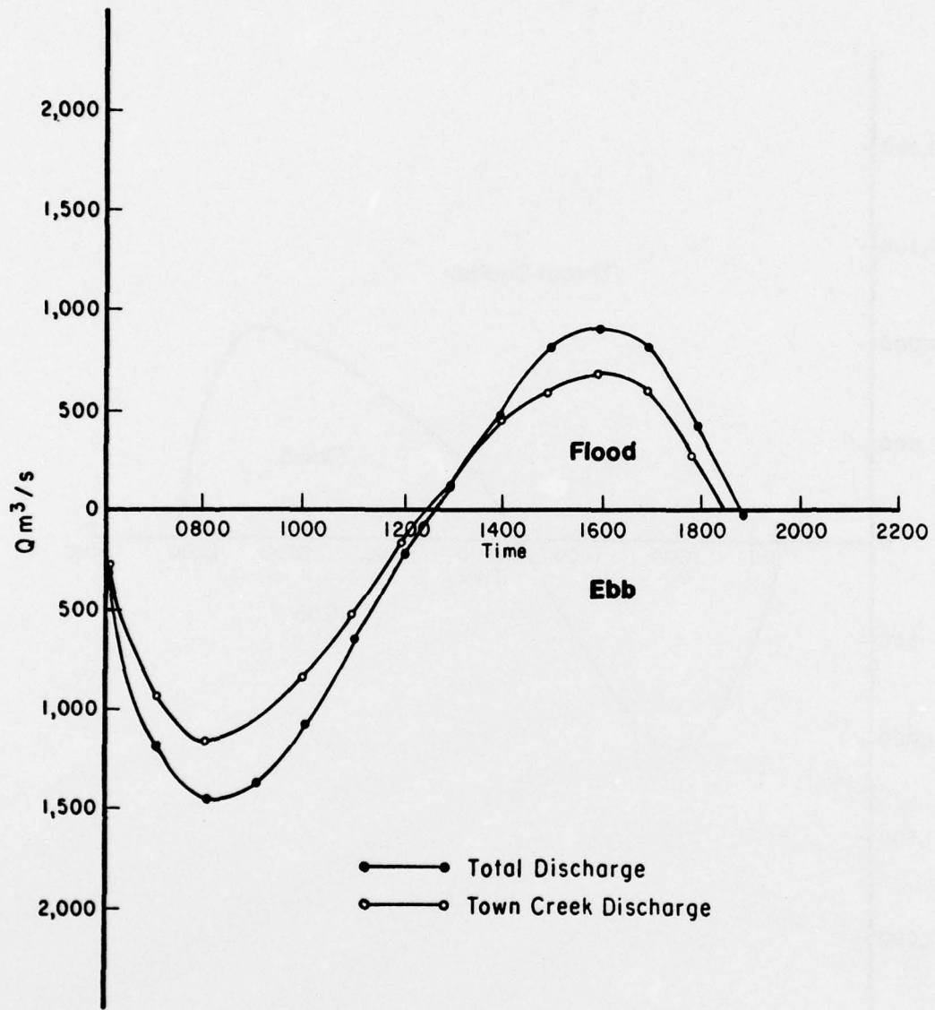
Figure D-16. North Inlet discharge, 24 March 1975.
