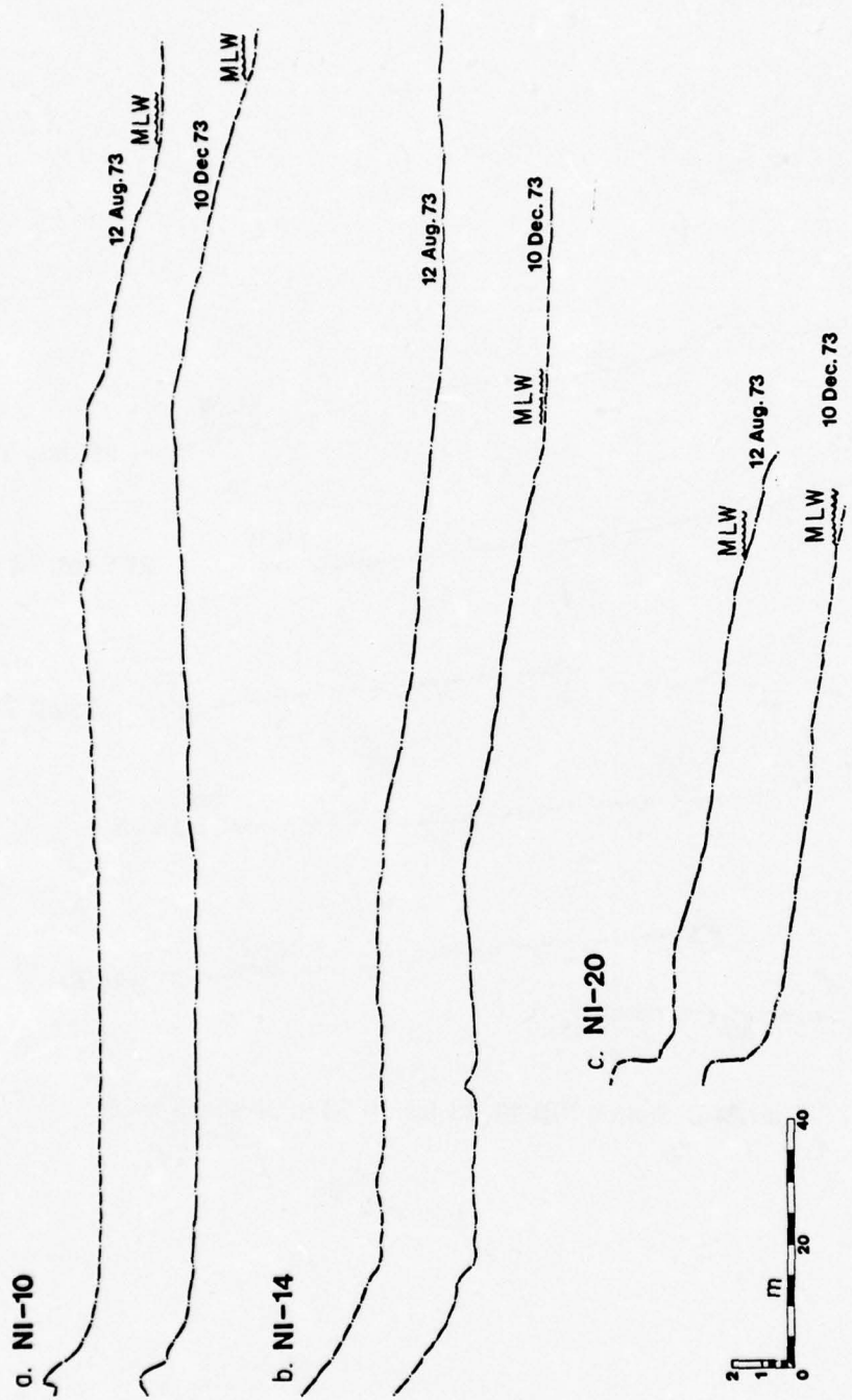
Figure B-7. Stations NI-10, NI-14, and NI-20, 12 August to 10 December 1973.
