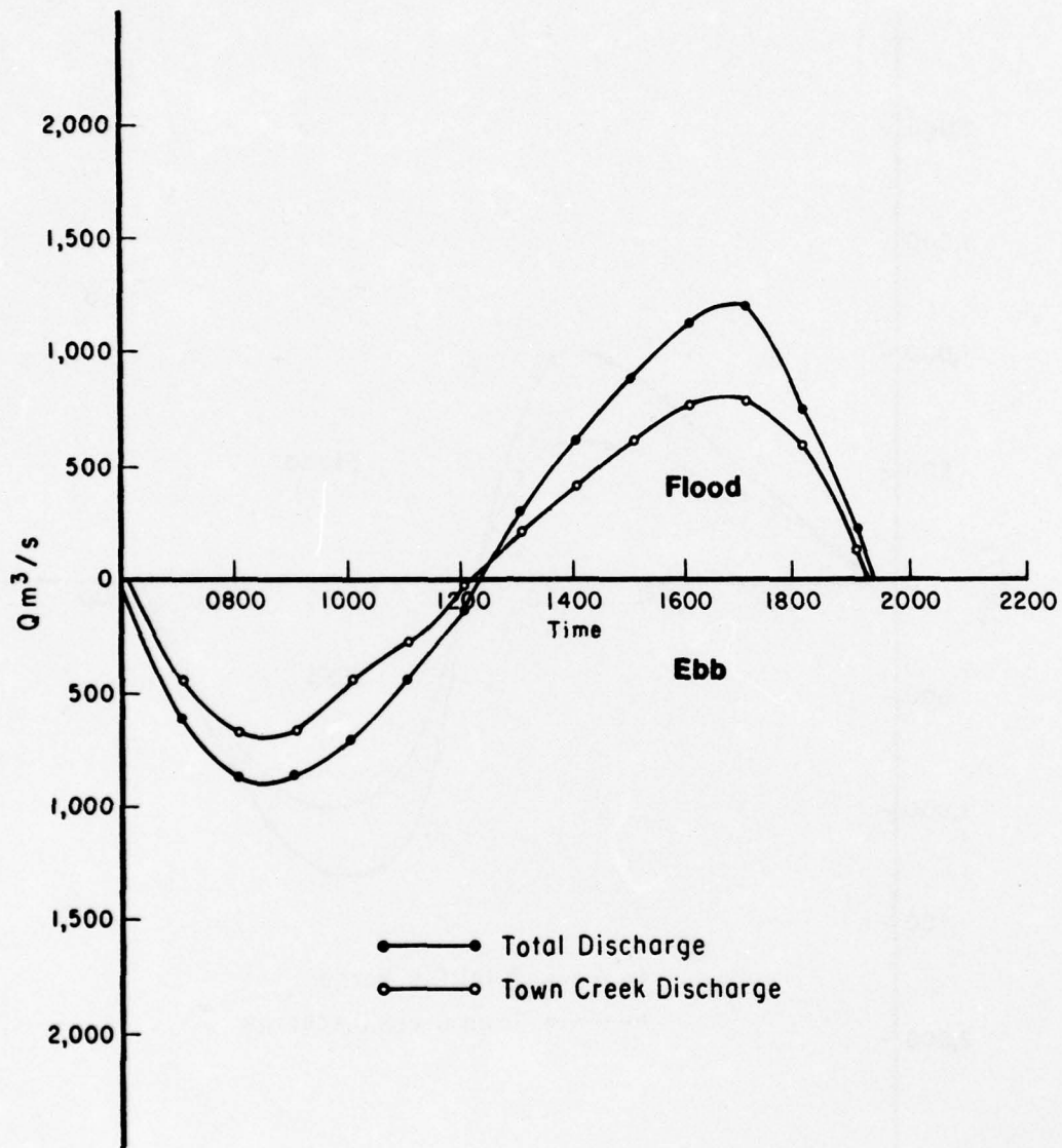
Figure D-7. North Inlet discharge, 27 September 1974.
