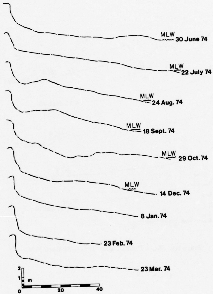
Figure B-8. Station DBI-20, 30 June 1974 to 23 March 1975.
