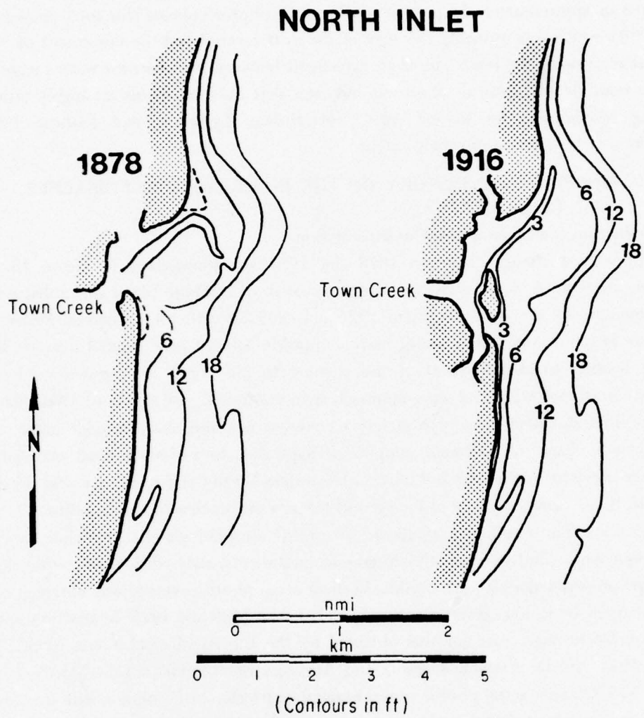
Figure 18. Early shoreline changes (after USC&GS).
