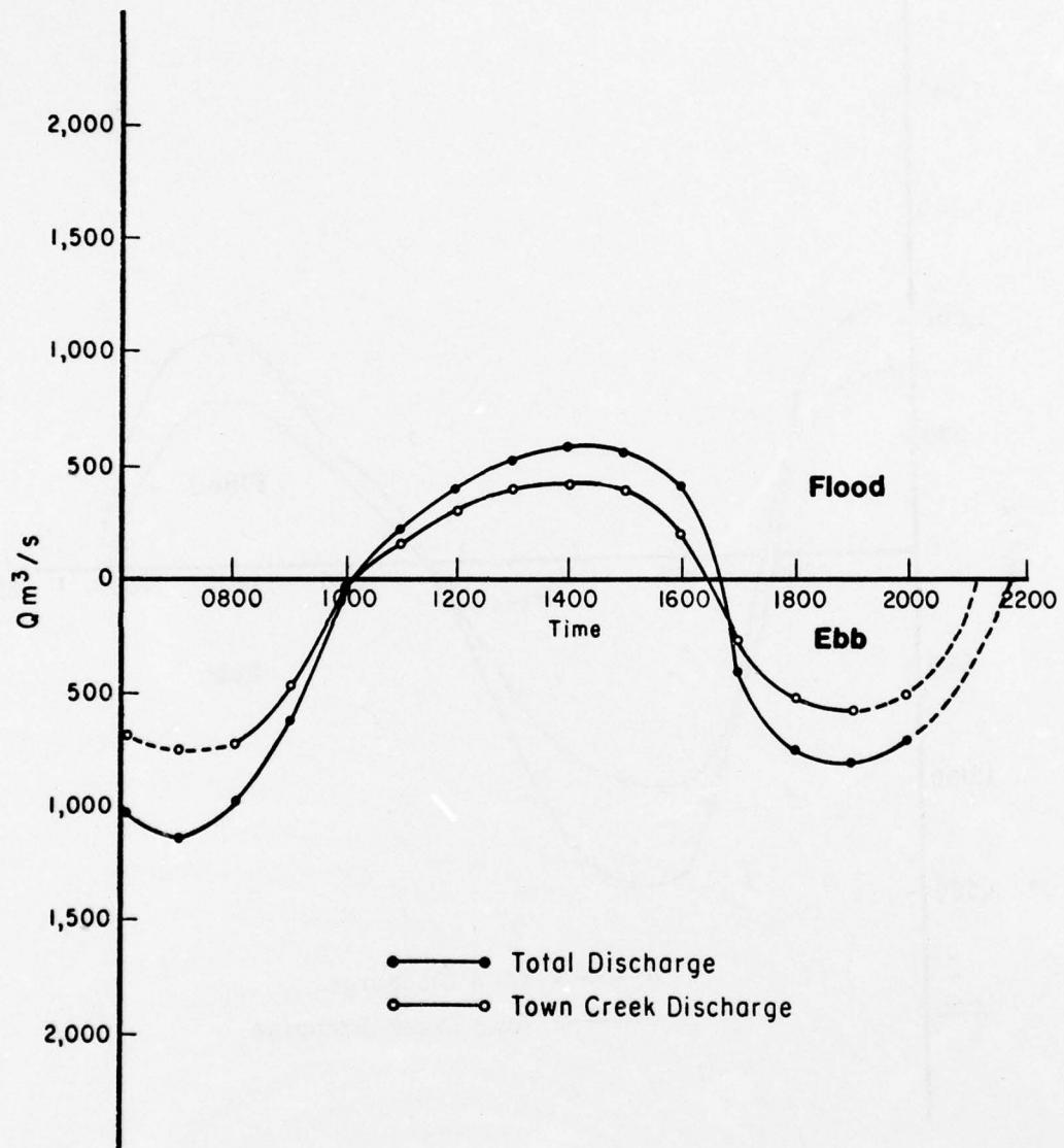
Figure D-10. North Inlet discharge, 7 January 1975.
