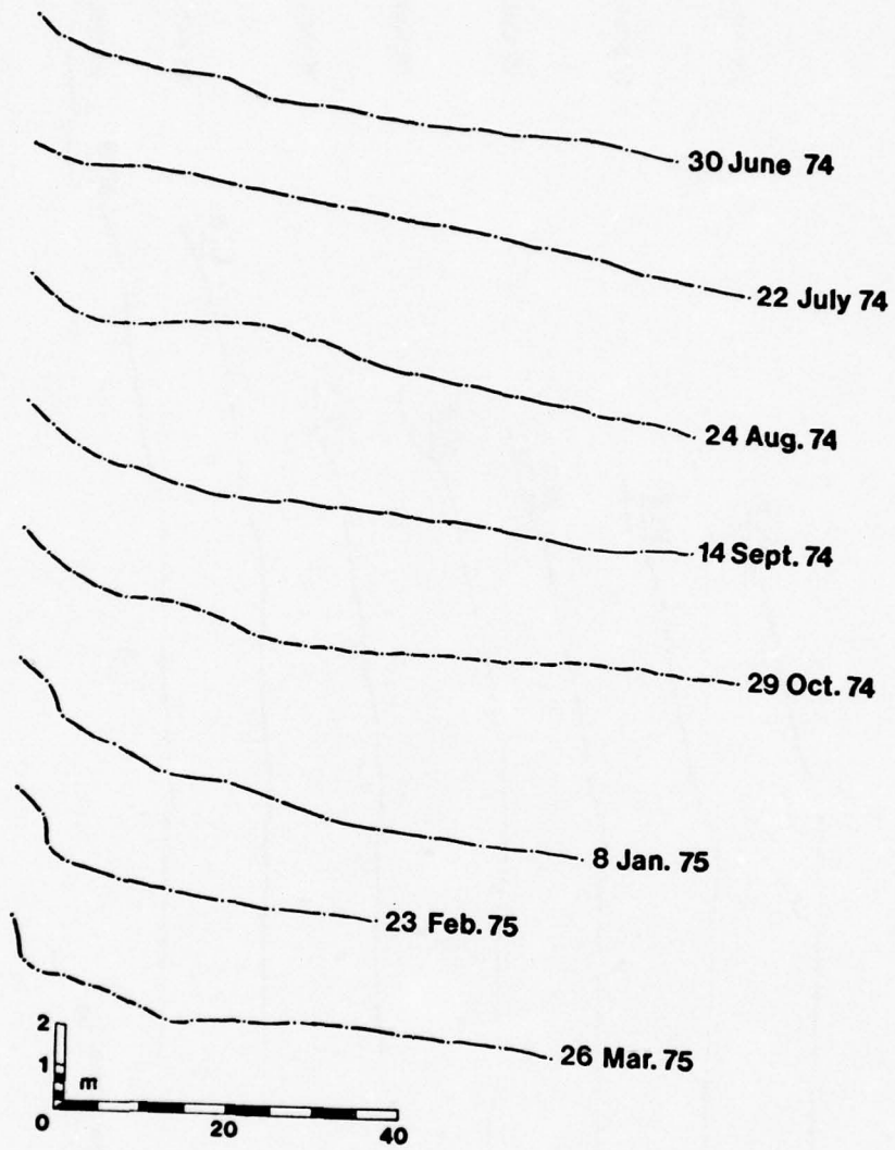
Figure B-12. Station DBI-30, 30 June 1974 to 26 March 1975.
