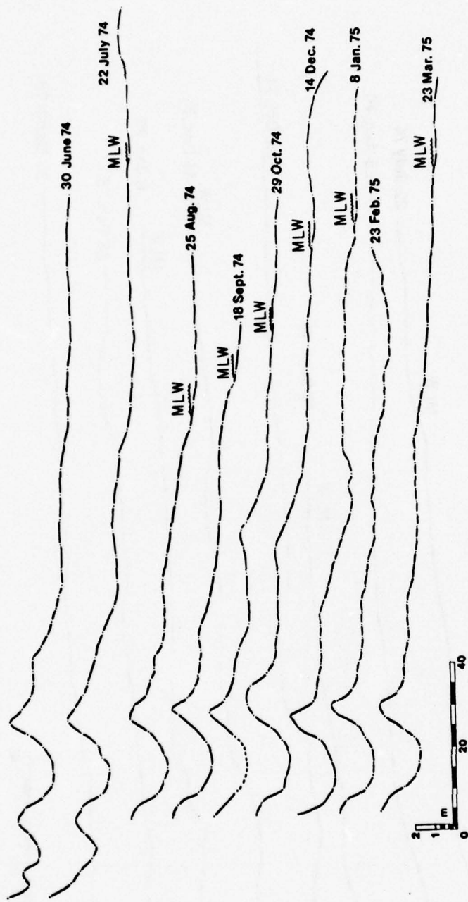
Figure B-2. Station DBI-6, 30 June 1974 to 23 March 1975.
