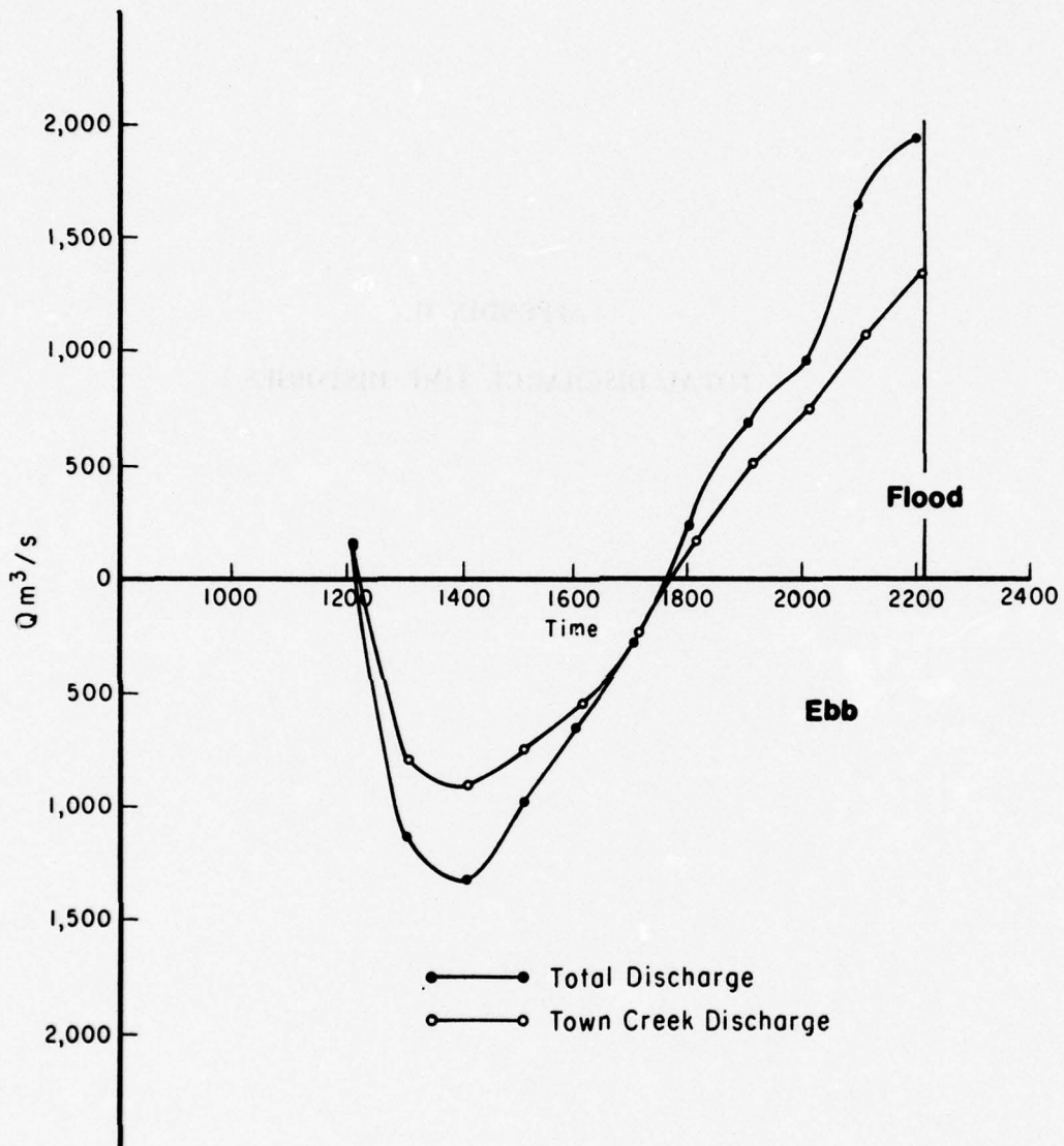
Figure D-1. North Inlet discharge, 20 July 1974.
