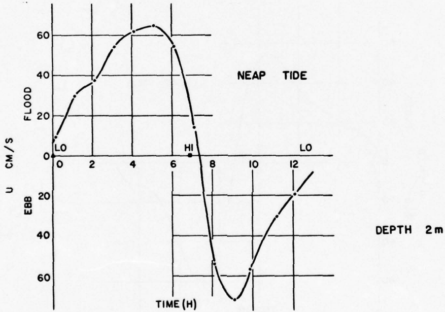
Figure C-14. Tidal current velocity, station JC-3, 20 July 1972.
