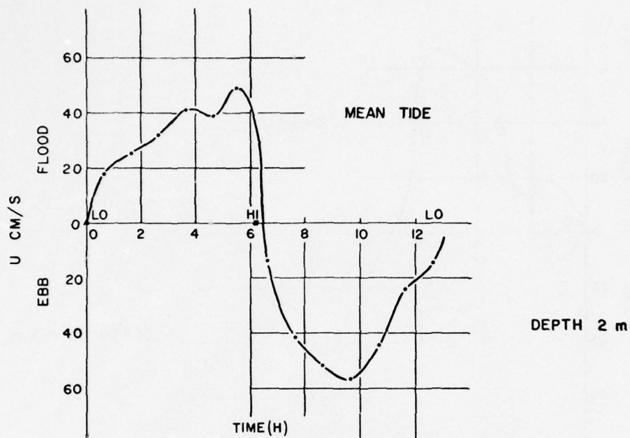
Figure C-7. Tidal current velocity, station TC-1, 25 July 1972.
