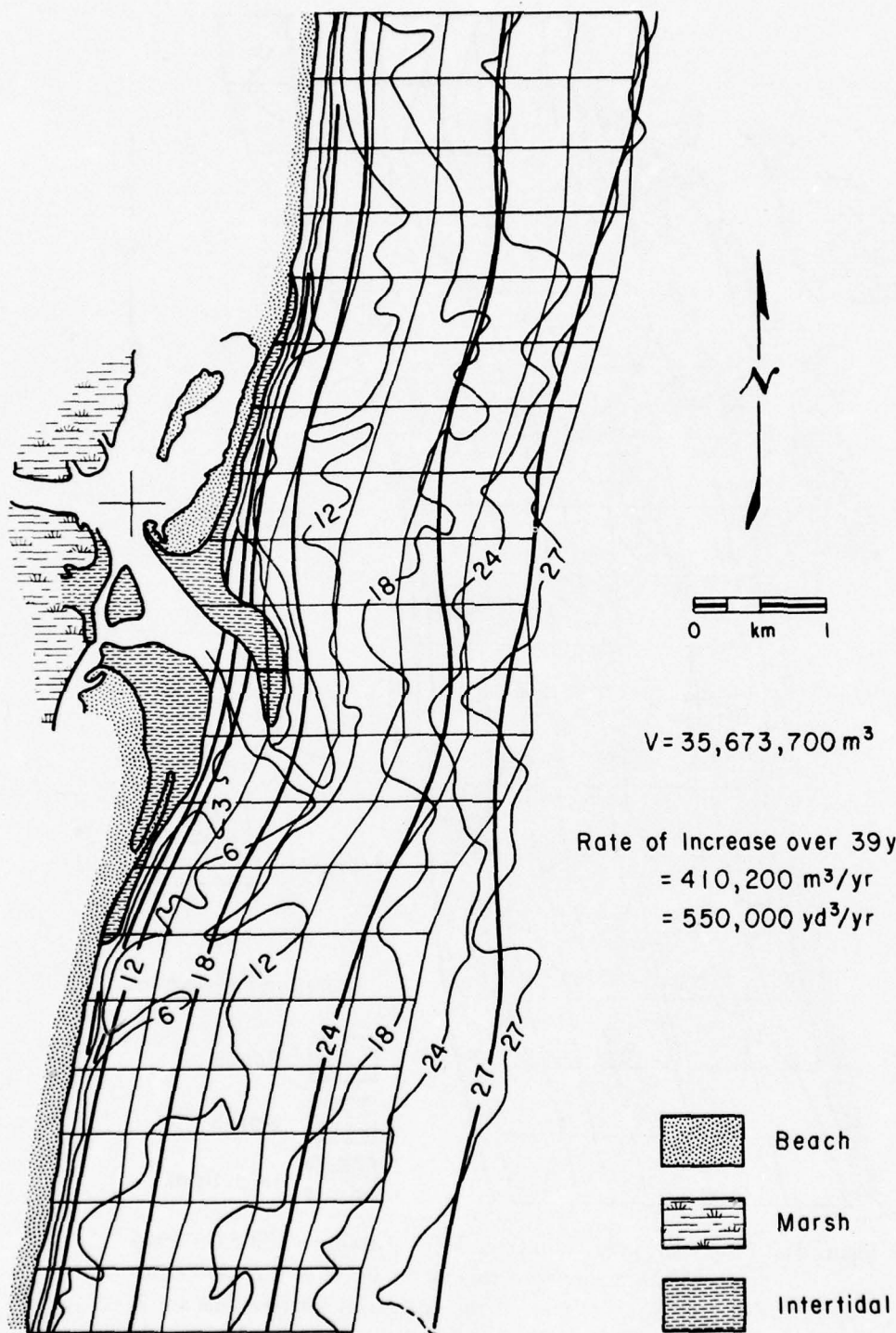
Figure 17. Ebb tidal delta volume in 1964 (based on USC&GS 1964 survey).
