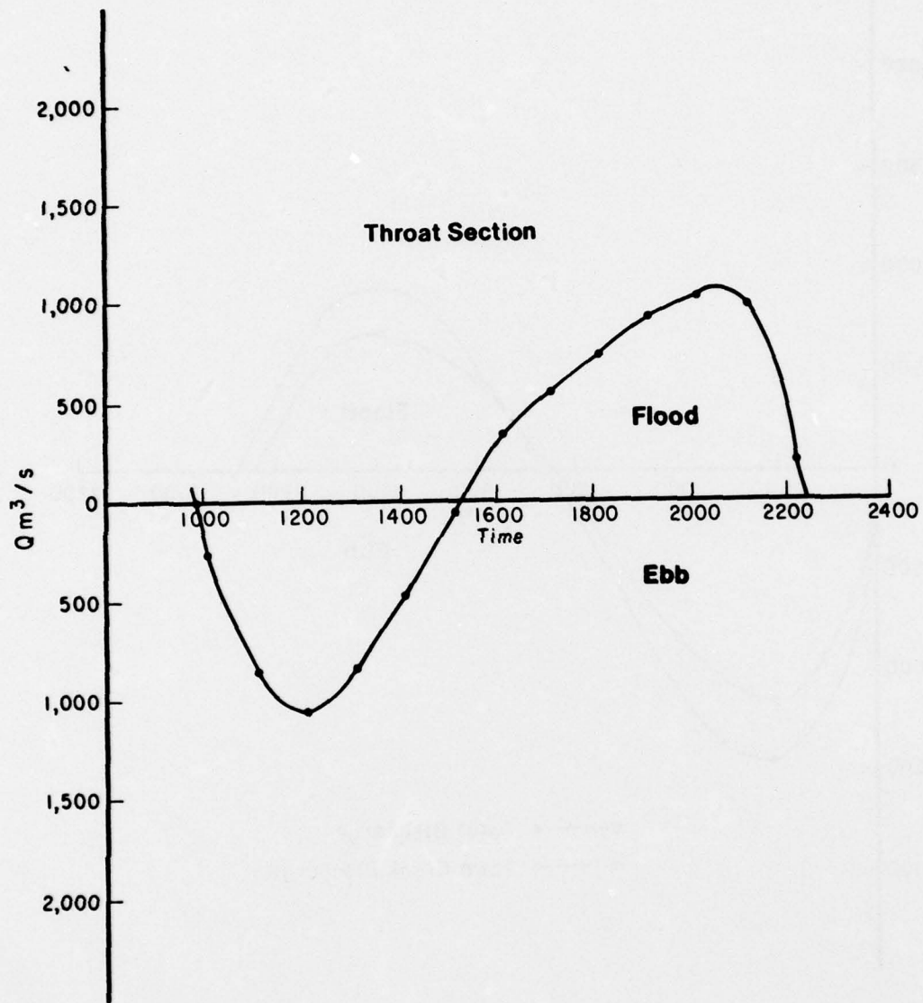
Figure D-17. North Inlet discharge, 26 April 1975.
