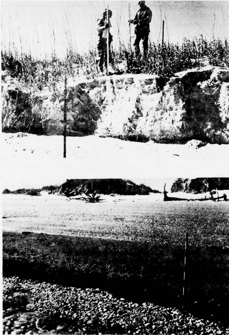
Figure 35. Foredune ridge scarp (upper photo) and peat exposure (lower photo) at profile NI-20. Length of scale is 1 meter.
