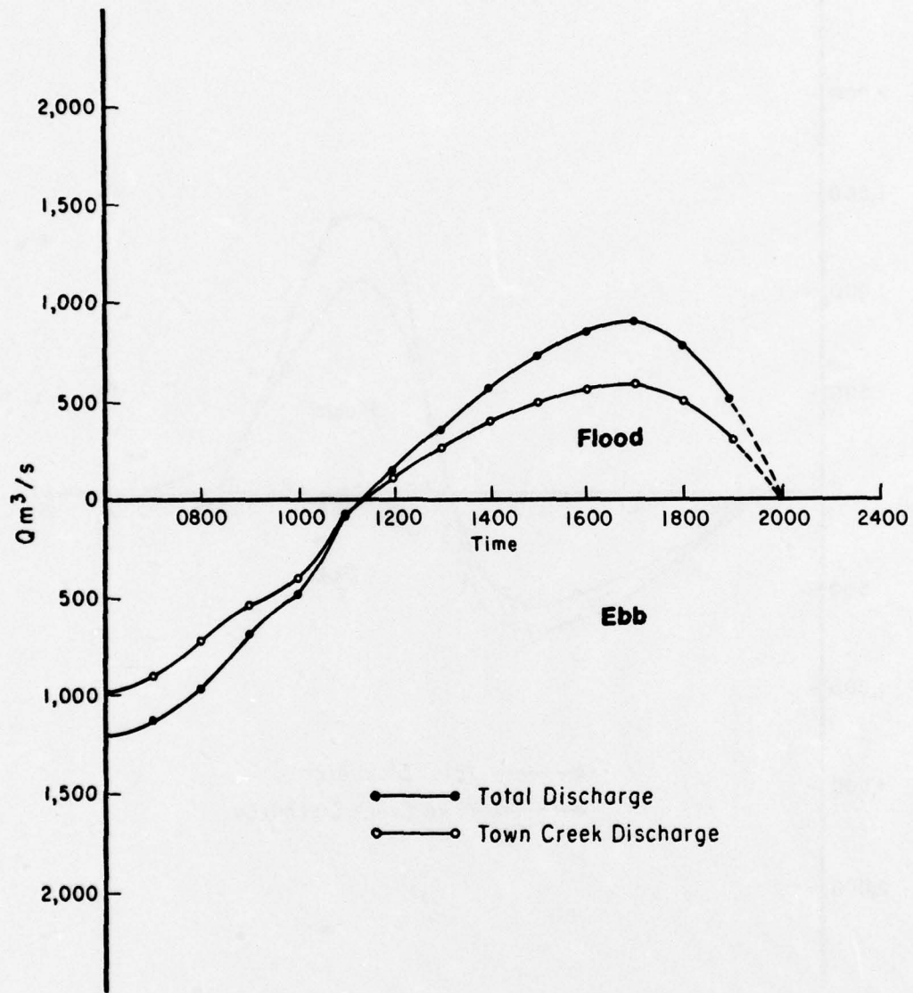
Figure D-8. North Inlet discharge, 27 October 1974.
