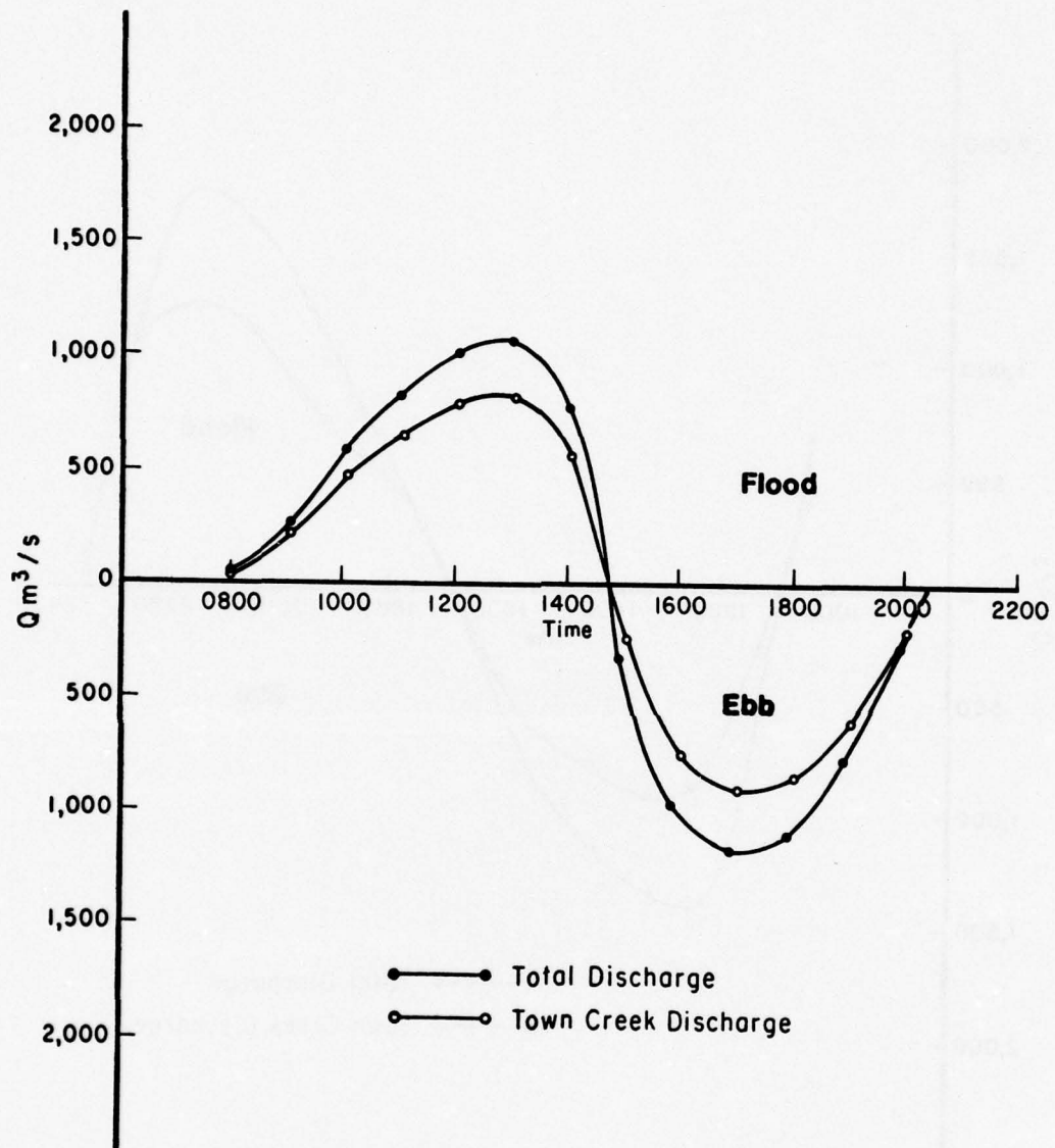
Figure D-4. North Inlet discharge, 24 August 1974.
