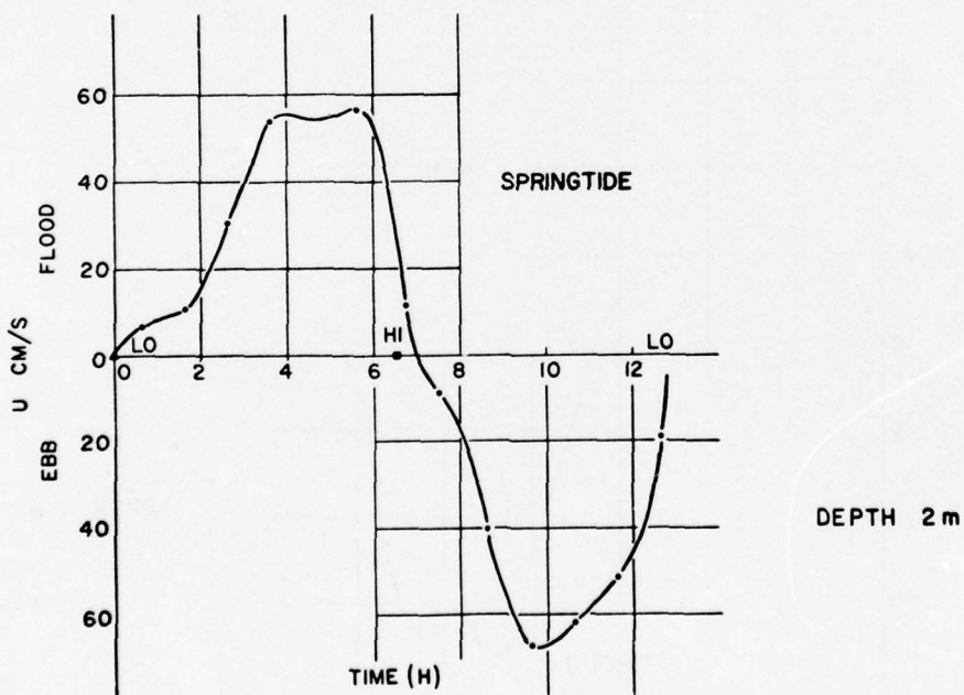
Figure C-10. Tidal current velocity, station TC-3, 6 August 1972.
