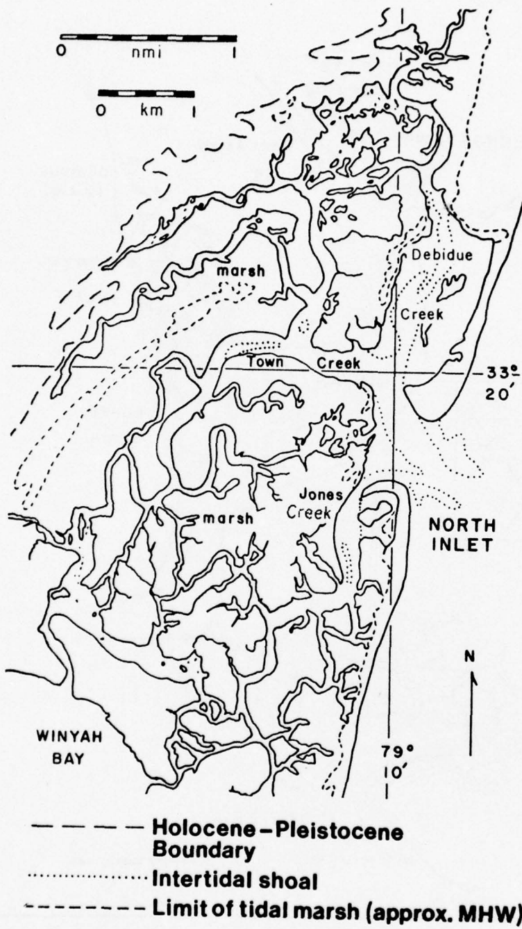
Figure 2. Detail of North Inlet bay area (based on NOS chart 11532).
