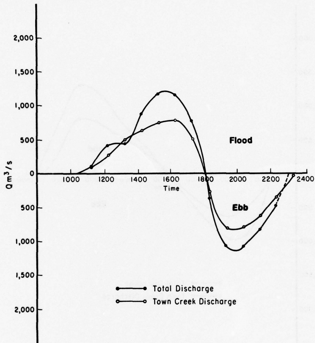
Figure D-2. North Inlet discharge, 26 July 1974.
