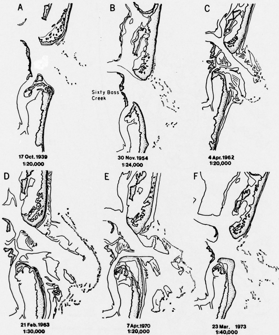
Figure 20. Historical changes at North Inlet. Sketches are based on vertical aerial photos. Beach areas interpreted to be above MHW are enclosed by heavier lines and are stippled. Pattern of short, parallel line segments indicates areas of breaking waves. On high tide photos (A, B, F), pattern gives the approximate location of shoals. Original photo scale indicated.
