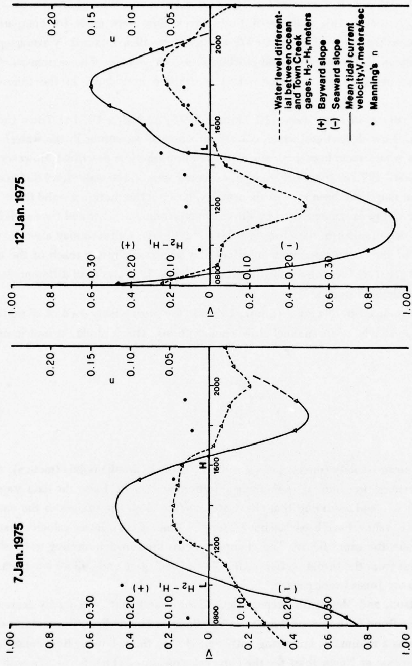
Figure 54. Time histories of tidal differential, currents, and Manning's n at Town Creek, 7 and 12 January 1975.
