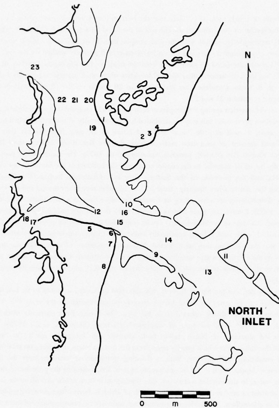
Figure 9. Sediment sample station locations, midtide level beach (1 to 8), intertidal shoal (9 to 12), and subtidal (13 to 23).
