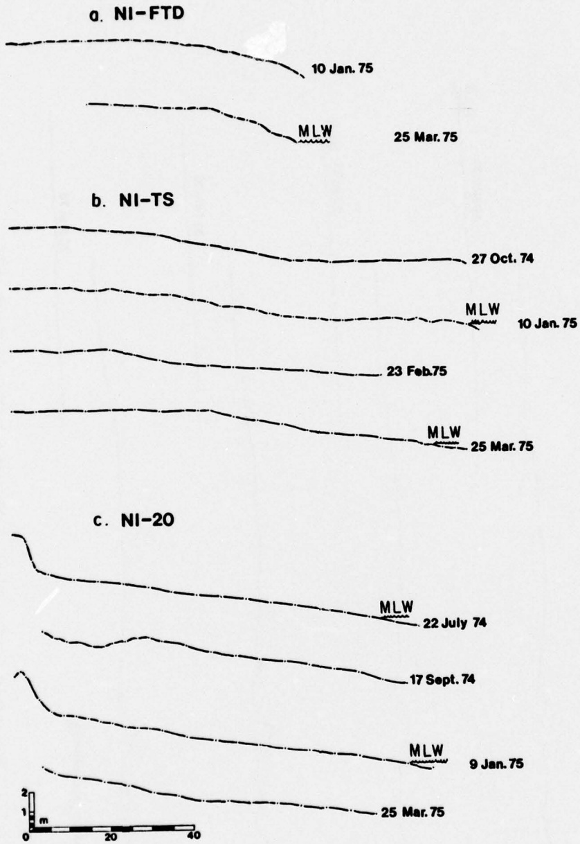
Figure B-19. Stations NI-FTD (10 January to 25 March 1975), NI-TS (27 October 1974 to 25 March 1975), and NI-20 (22 July 1974 to 25 March 1975).
