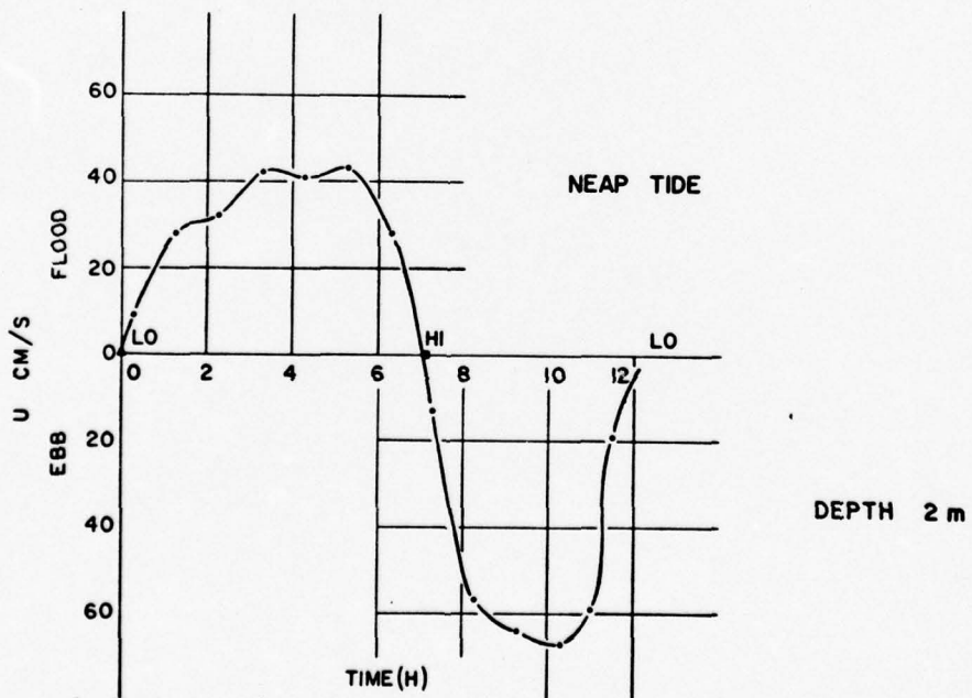
Figure C-2. Tidal current velocity, station IN-1, 18 July 1972.
