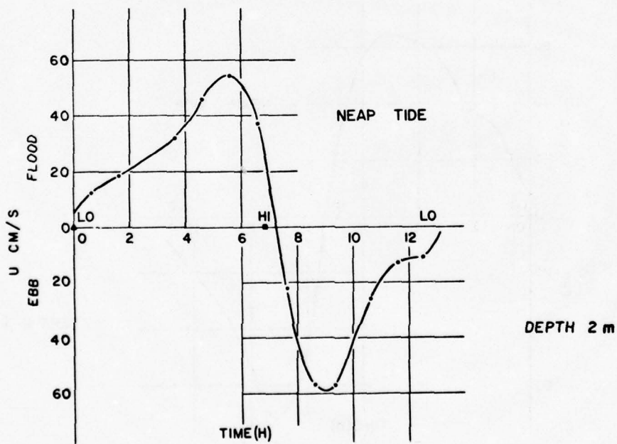
Figure C-12. Tidal current velocity, station JC-1, 20 July 1972.
