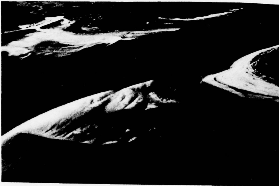
Figure 29. Inner channel-margin linear bar, July 1974.
