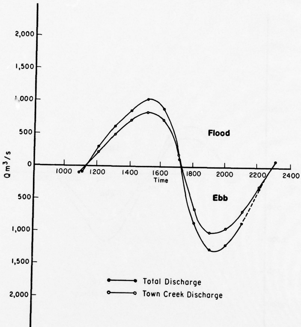
Figure D-12. North Inlet discharge, 22 February 1975.
