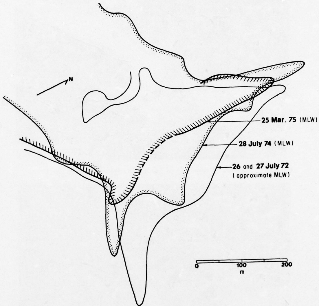
Figure 40. North Inlet flood tidal delta planforms.
