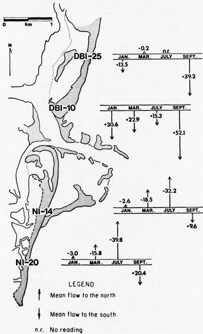
Figure 11. Resultant longshore current vectors (centimeters per second).
