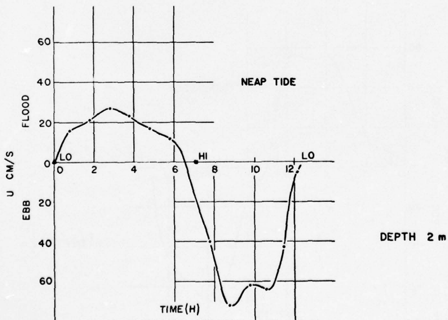
Figure C-8. Tidal current velocity, station TC-1, 18 July 1972.
