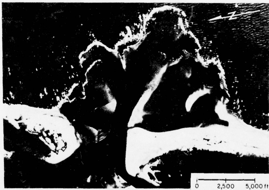
Figure 39. Vertical view of North Inlet, March 1975 (NOAA).
