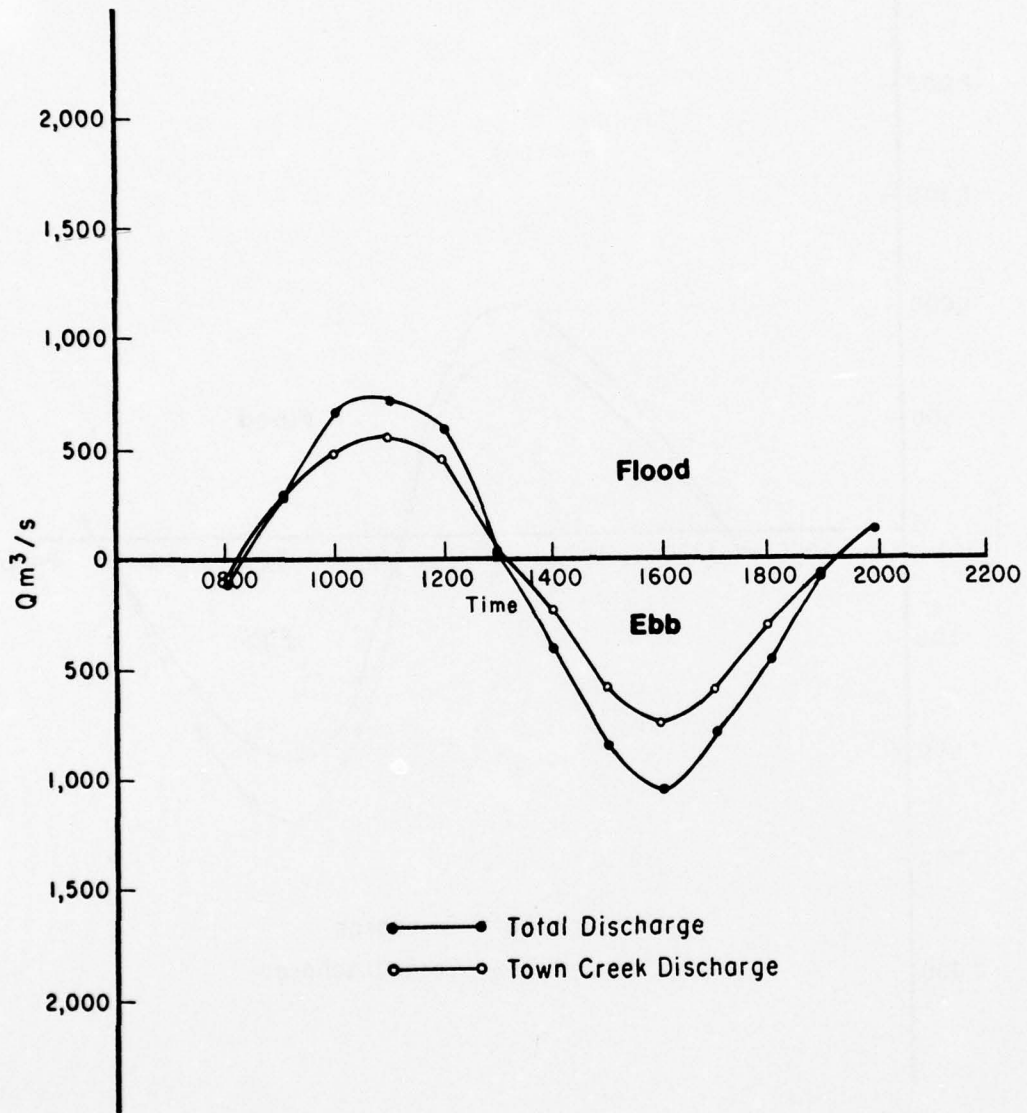
Figure D-13. North Inlet discharge, 19 March 1975.
