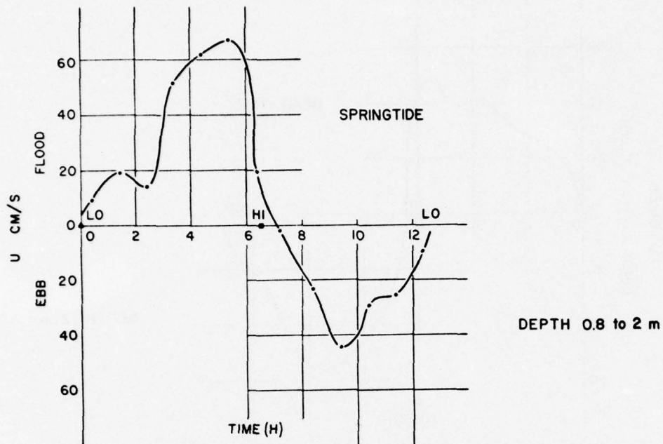
Figure C-9. Tidal current velocity, station TC-2, 6 August 1972.
