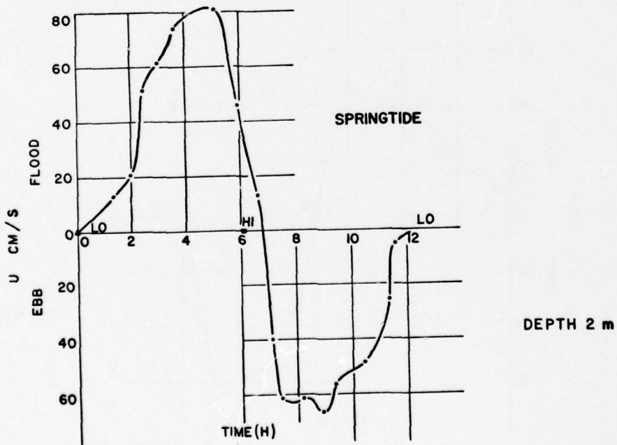
Figure C-6. Tidal current velocity, station IN-6, 5 May 1973.
