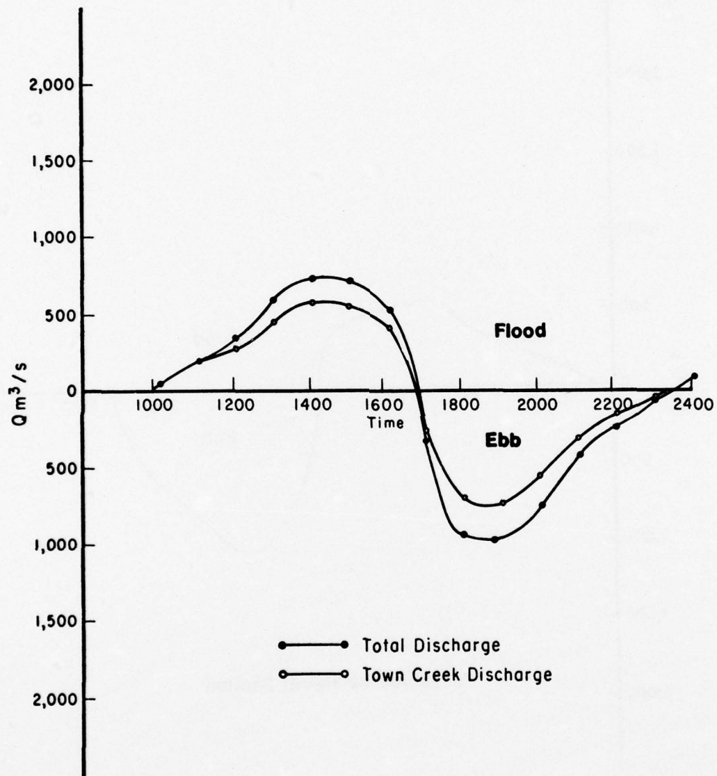
Figure D-15. North Inlet discharge, 22 March 1975.
