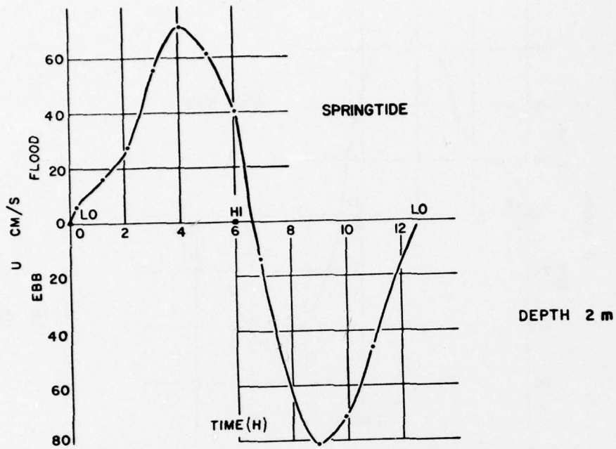
Figure C-5. Tidal current velocity, station IN-6, 14 April 1973.
