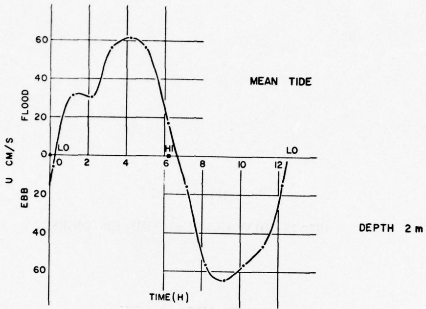
Figure C-1. Tidal current velocity, station IN-1, 25 July 1972.
