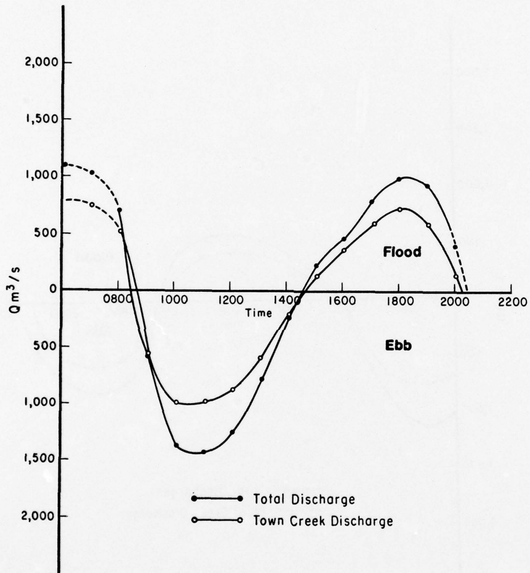
Figure D-11. North Inlet discharge, 12 January 1975.
