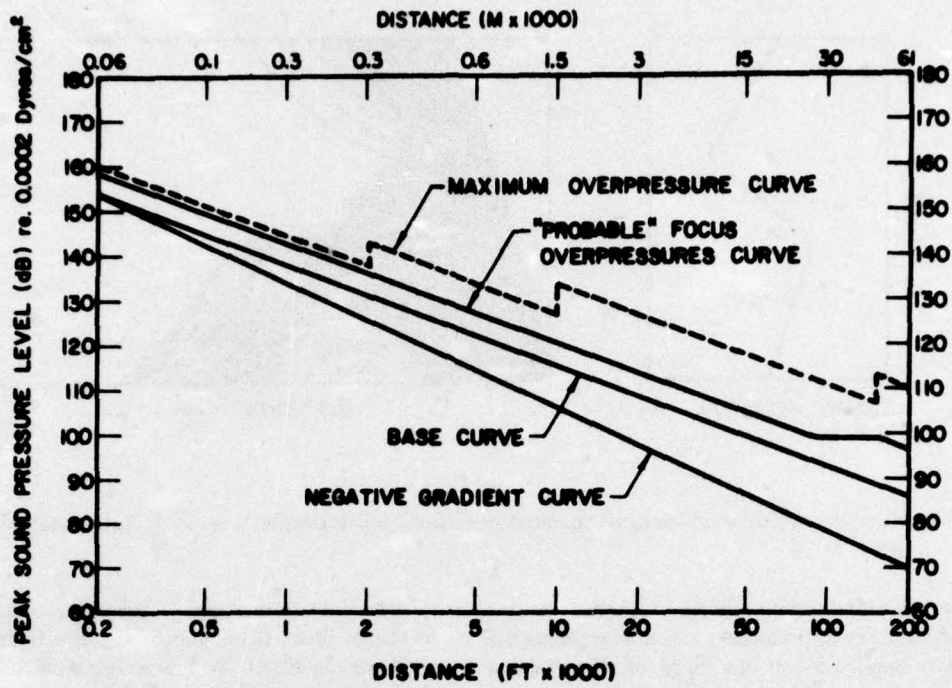
Figure 17. Theoretical amplitude versus distance prediction curves from CERL Technical Report E-17.
