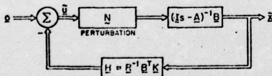
Fig. 2 Perturbed LQSF Regulator ( \Sigma )
