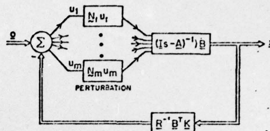
Fig. 3 LQSF Regulator with Non-interacting Perturbations in Each Control Loop
