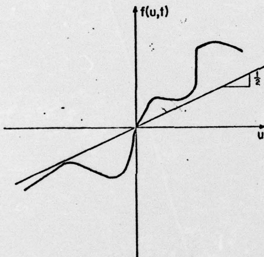
Fig. 1 Non-destabilizing Nonlinear Feedback Gain
