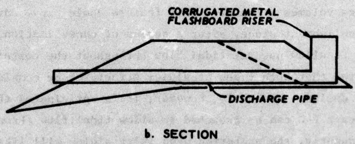
Figure 14. Plan and section views of drop inlet sluice (pipe and riser)
