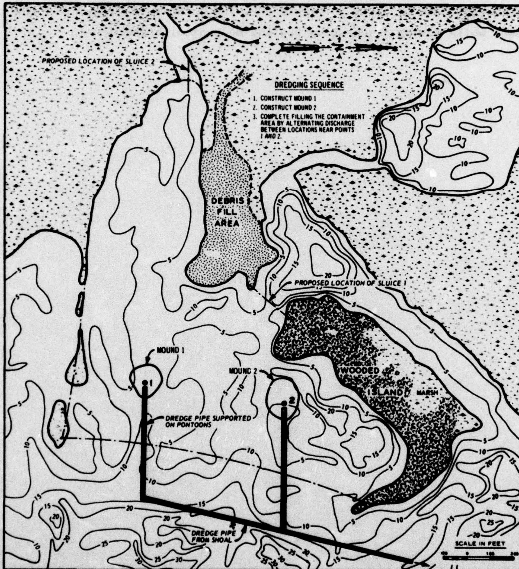
Figure 20. Dredged material placement scheme
