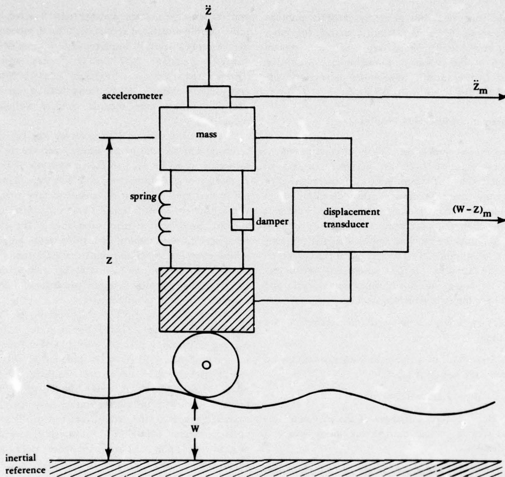
Figure 5. Profilometer sensor subsystem [18].
