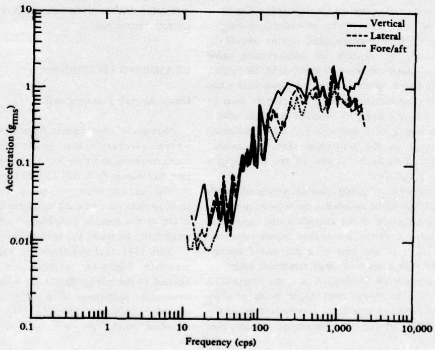
Figure 4. Acceleration envelope for KC-135 aircraft [11].
