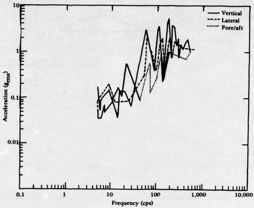
Figure 3. Acceleration envelope for C-130 aircraft [11].
