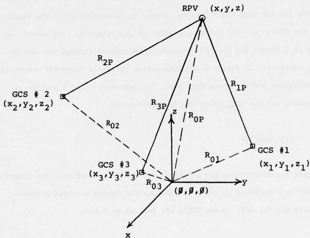
Figure A-1 Geometry of RPV Position By Trilateration
