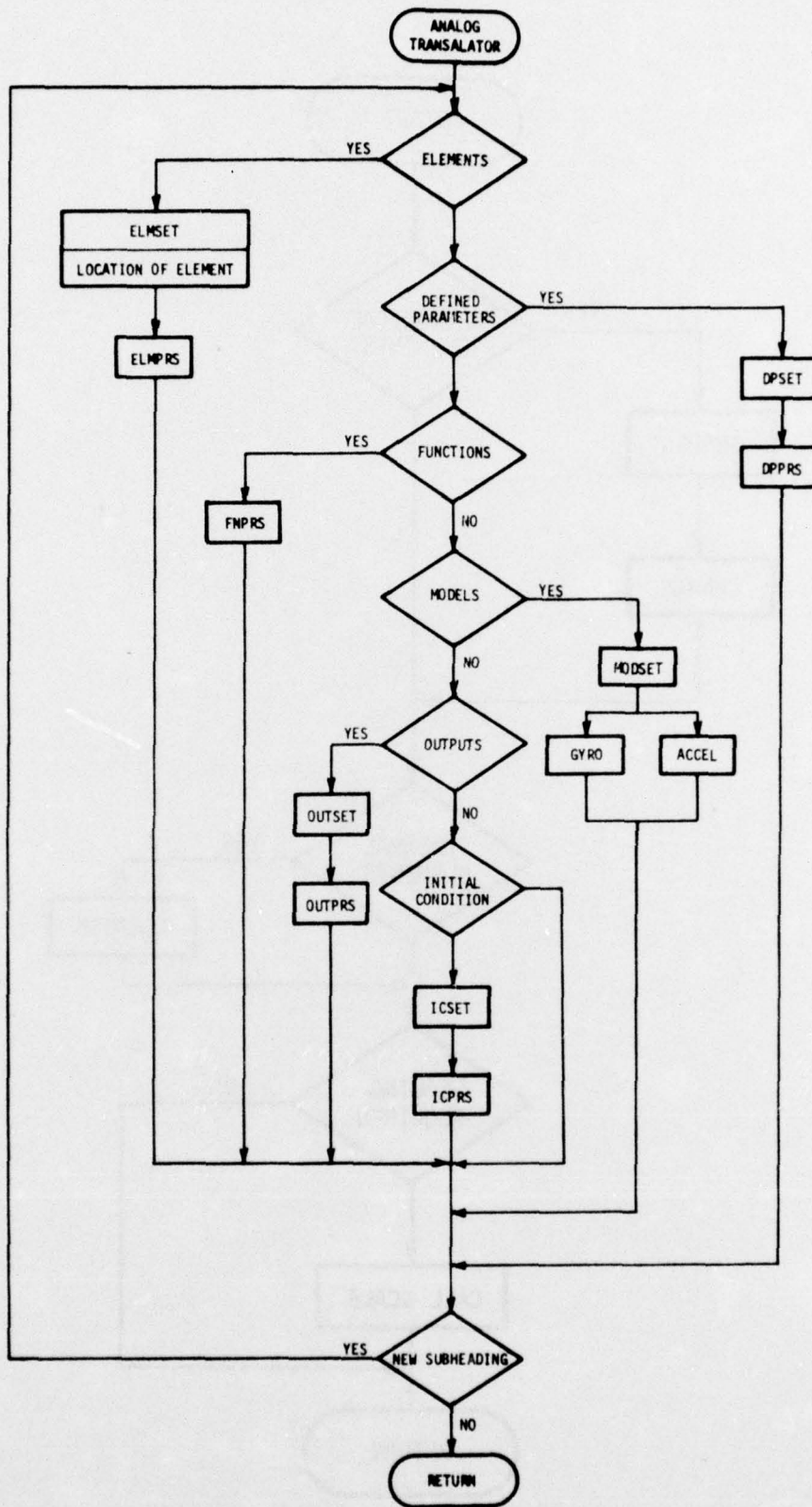
Figure 24. Function Subheading Processor
