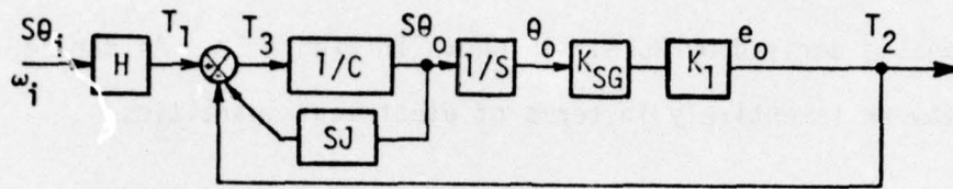
Figure 13. Block Diagram of Rate Gyro
