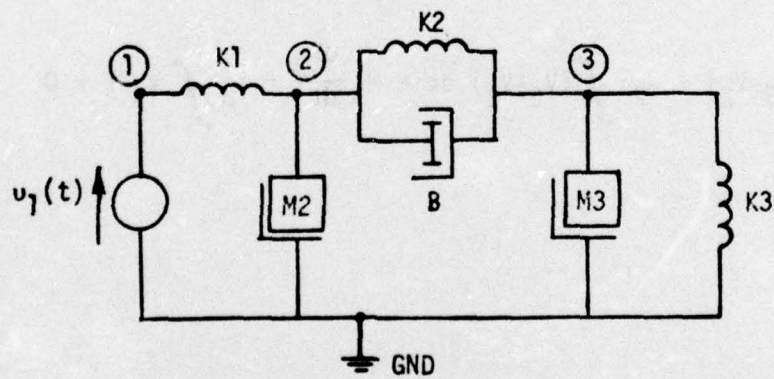
Figure 5. Mechanical Network Equivalent
