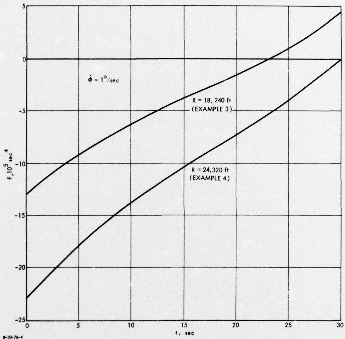
FIGURE 2. Collision Threat Criterion Polynomial F = f(t)
