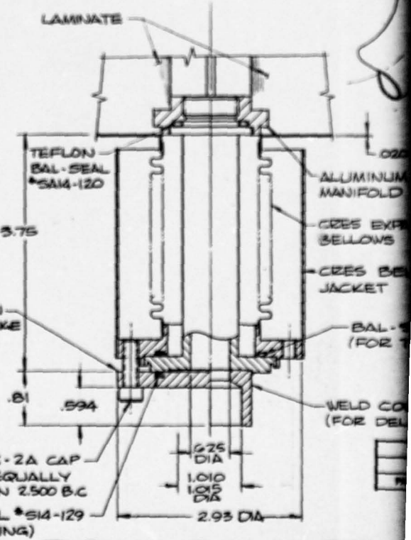
TYPICAL FLANGE DETAIL SCALE: 1/1
