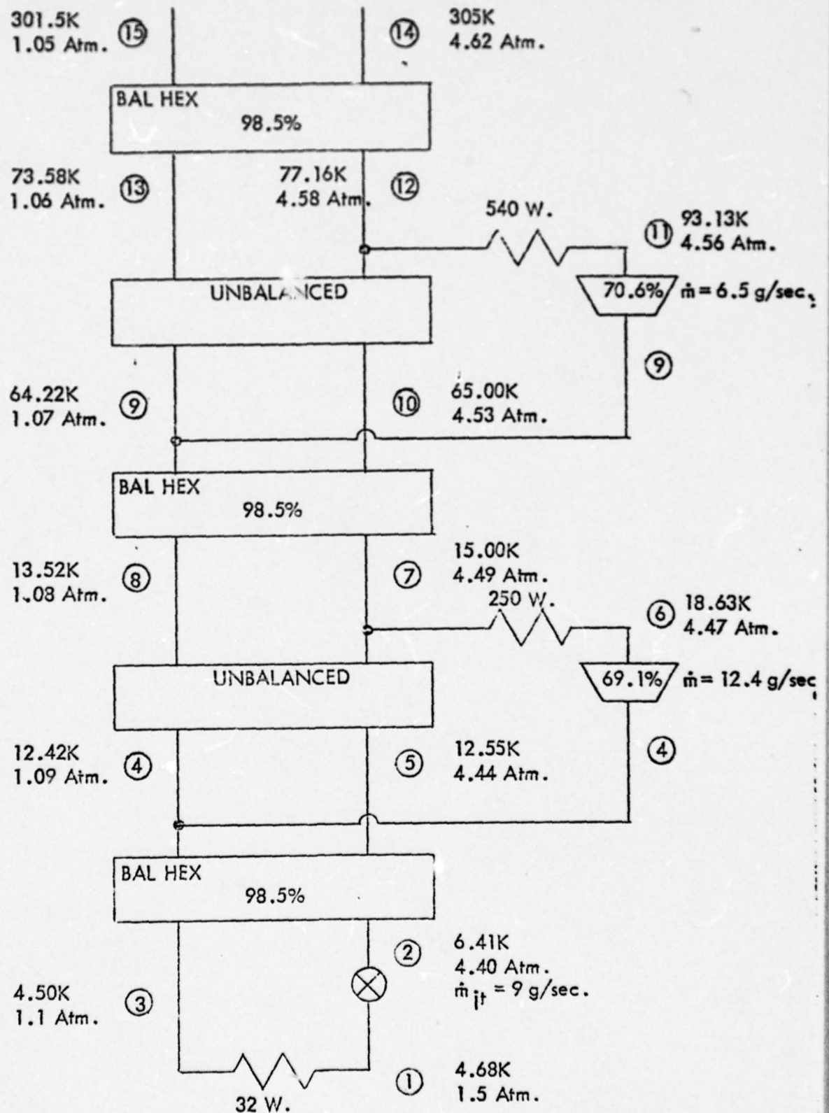
Figure 2-4 - Heat Exchanger Thermodynamic State Schematic
