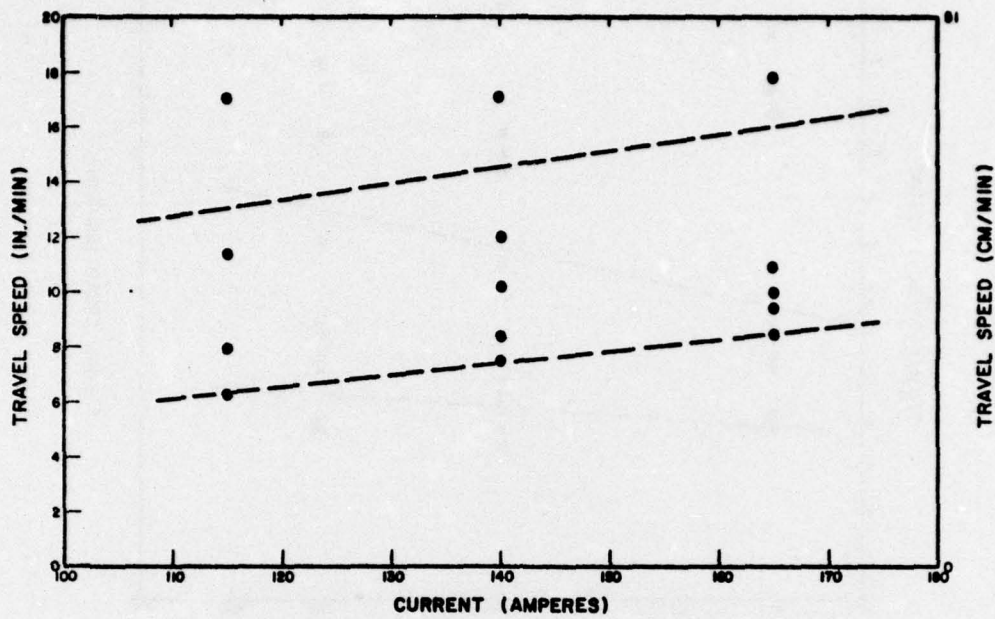
Figure 7. Graph of travel speed versus current for 1/8-in. (3.2 mm) diameter E11018 SMAW electrode. Dashed lines show travel speed limits as determined by amount of undercut and bead shape.
