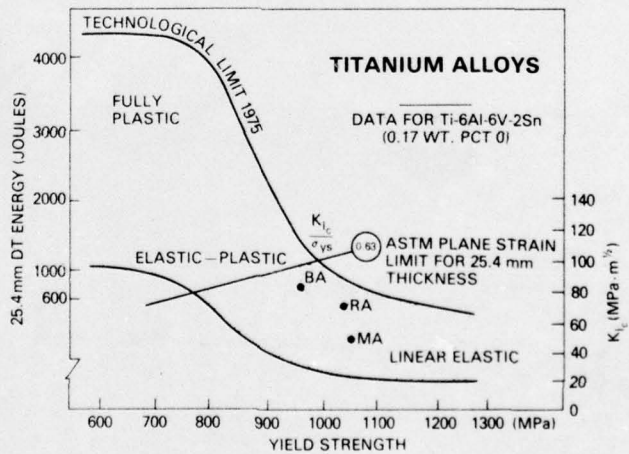
Fig. 7—Influence of heat treatment on fracture toughness and strength level of Ti-6Al-6V-2Sn
