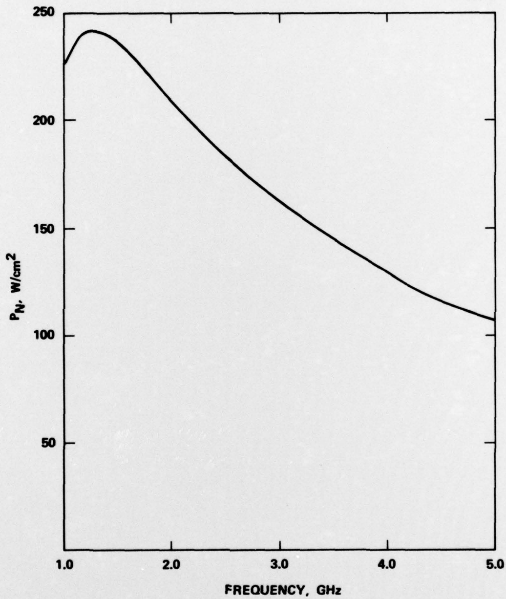
Figure 5 Output power density versus frequency.
