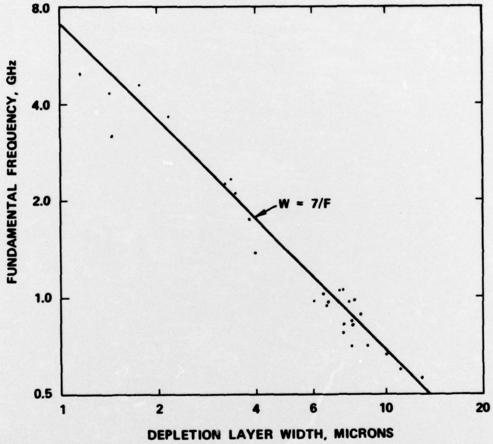
Figure 3 Fundamental frequency versus depletion layer width.
