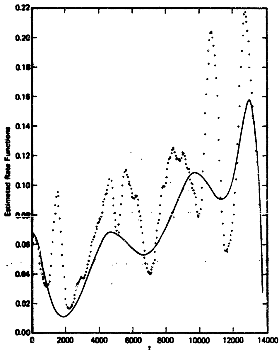
Figure 9. Estimates of the rate function for time period L (low activity). Solid curve is the NHPP estimate \hat{\lambda}(t; \hat{\alpha}) using exponential polynomial (degree 8). Dotted curve is the estimate \hat{\lambda}(t; n, t_0) using a kernel-type density estimator. Sample size n = 1258 , band-width b(n) = 1.25/n^{1/2} . Triangular window.
