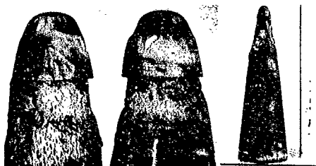
Figure 2-33. Post Test of Porous Tungsten Nosetip No. 5 Tested for 4 Seconds
