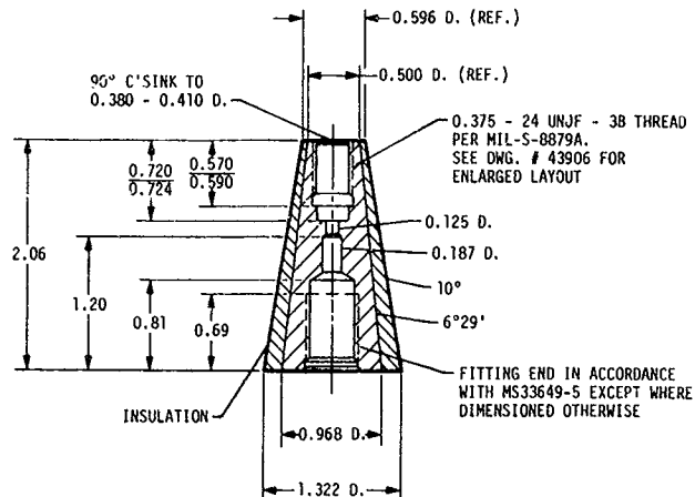
Figure 2-13. Model Adapter Forward Body
