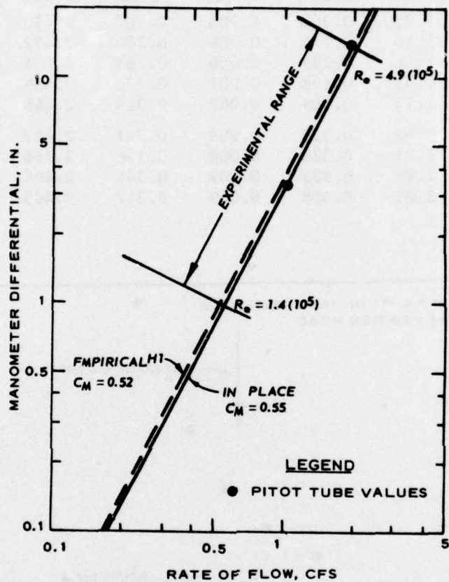
Figure 4. Bend meter calibration in which L_c is the crest length (2.500 ft for the test facility). A series of observations, tests H1-H14, were performed in order to determine C as a function of H_e ; the data and calculations are tabulated below, and the results are summarized in Figure 5.
