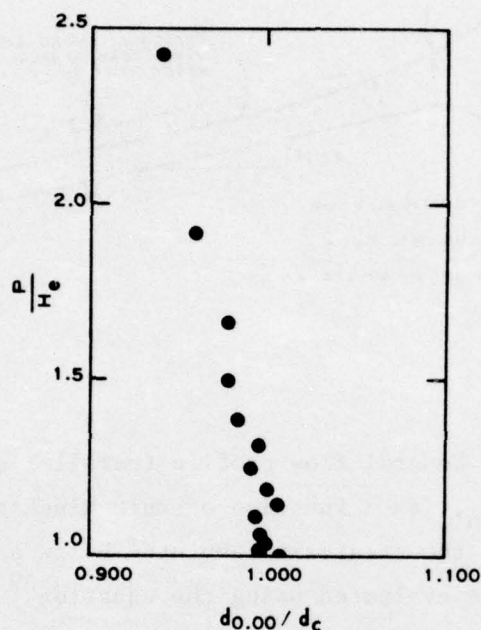
Figure 7. Depth at the spillway crest (parallel sidewalls)
