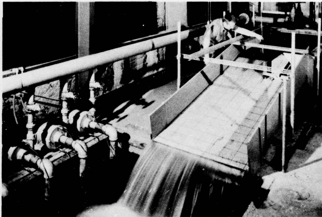
Figure 2. Experimental facility
