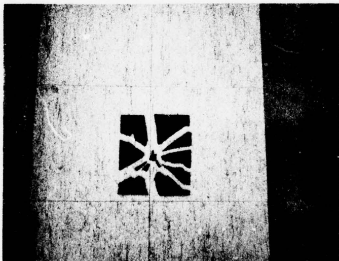
Figure 2. Specimen V2 after impact test.
