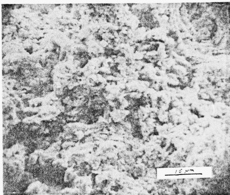
Figure 89. Active material in the outer layers of the plate. Note the enlargement of the agglomerate of PbO_2 . Lead-calcium PbCA#1, 20 cycles, 1200X.
