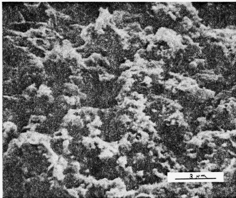
Figure 94. Active material at the interface with the grid. Note the ordered arrangement and development of voids beginning to form in this active material. Lead-calcium PbCA#1, 40 cycles, 2500X.
