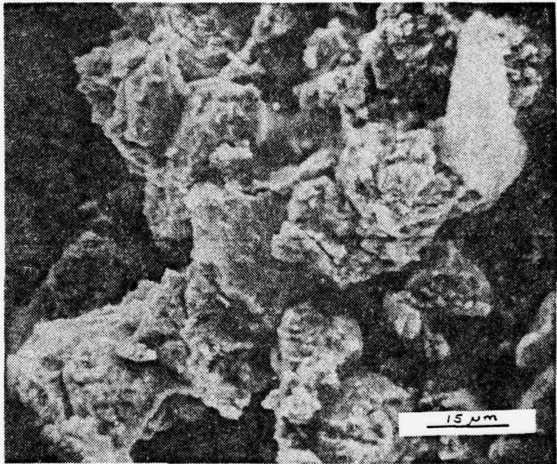
Figure 57. Enlarged coralloid near the grid. Lead-antimony battery PbSb#1, 45 cycles, 1100X.
