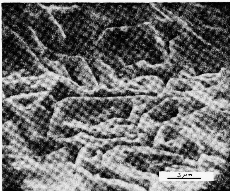
Figure 81. Partially transformed lead-sulfate at the grid surface. The spiny needle-like crystals are in evidence around those crystals. Lead-calcium PbCA#1, 10 cycles, 5500X.
