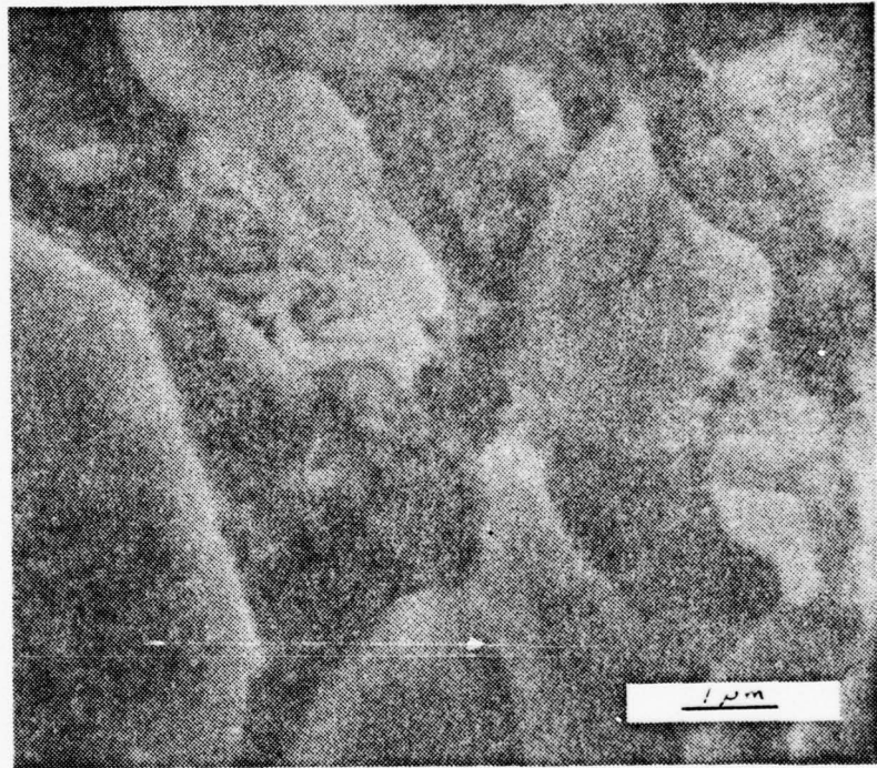
Figure 95. Area between lead-sulfate crystals near the grid. Note the dendritic crystals in these areas. Lead-calcium PbCA#1, 40 cycles, 12700X.
