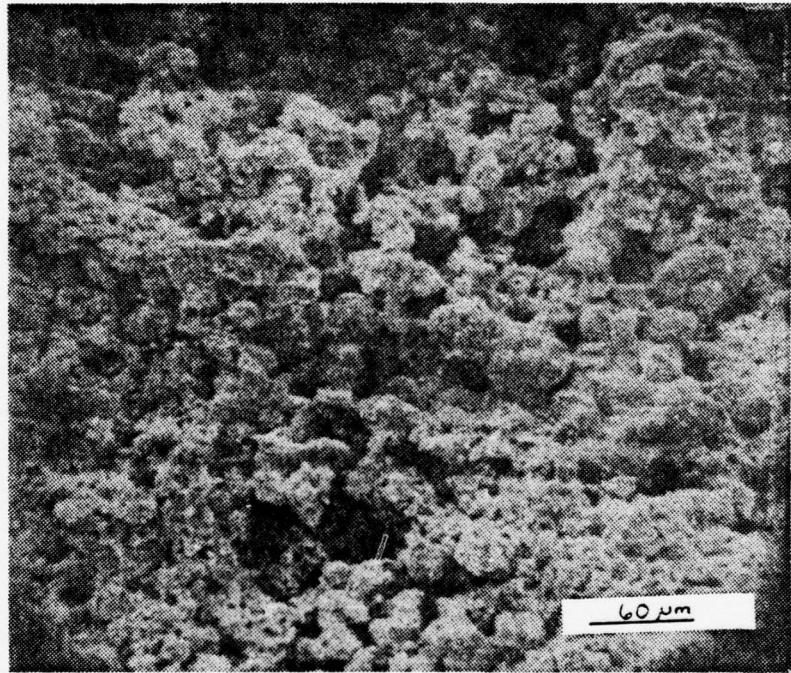
Figure 65. Active material at the center of the pellet in the transition to the coralloid structure. Lead-antimony battery PbSb#2, 50 cycles, 240X.
