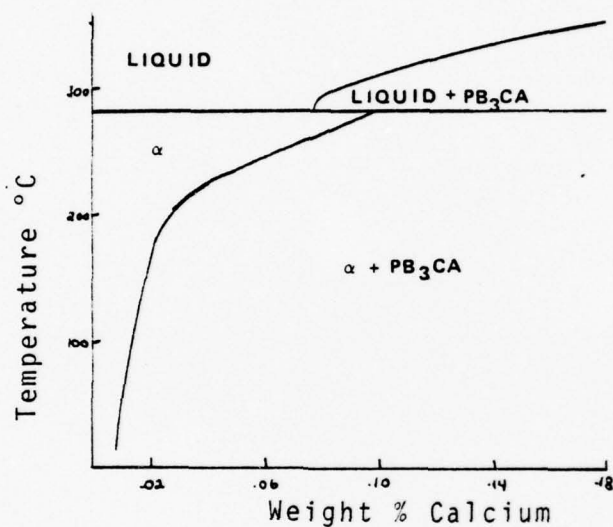
Figure 6. The Lead-Calcium Phase Diagram
