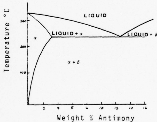
The Lead-Antimony Phase Diagram
