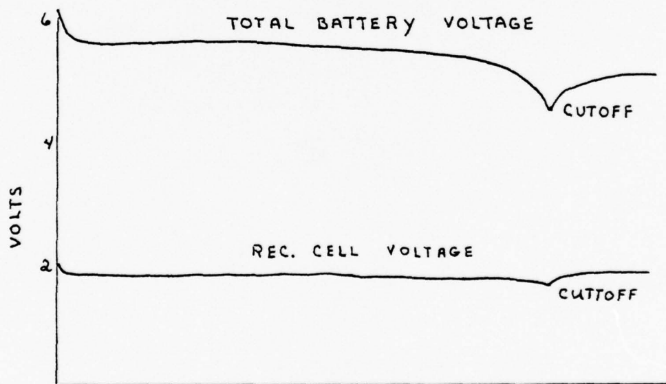
TIME NONLIMITING CELL DISCHARGE CURVES
