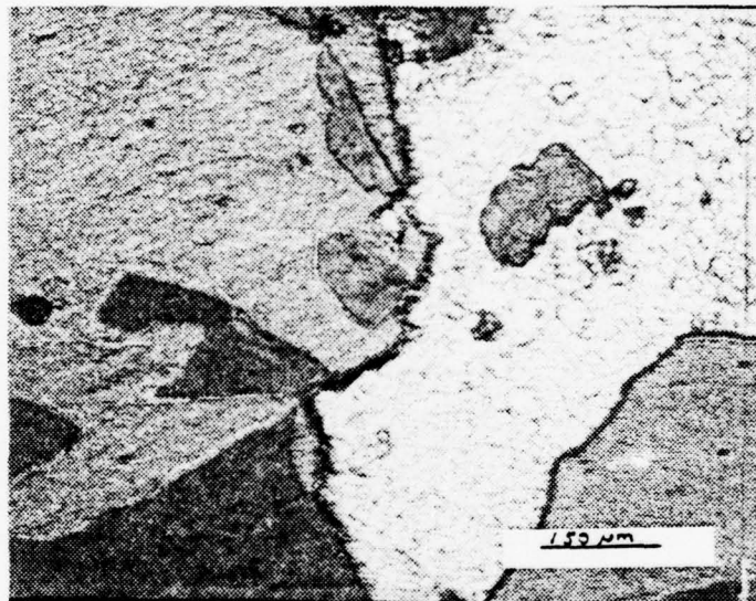
Figure 7. Microstructure of the lead-calcium grid material from a submarine type battery plate.
