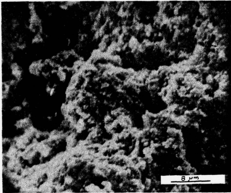
Figure 49. Active material near the center of the pellet with the first stages of void development within the active material. Lead-antimony battery 20 cycles, 2400X.
