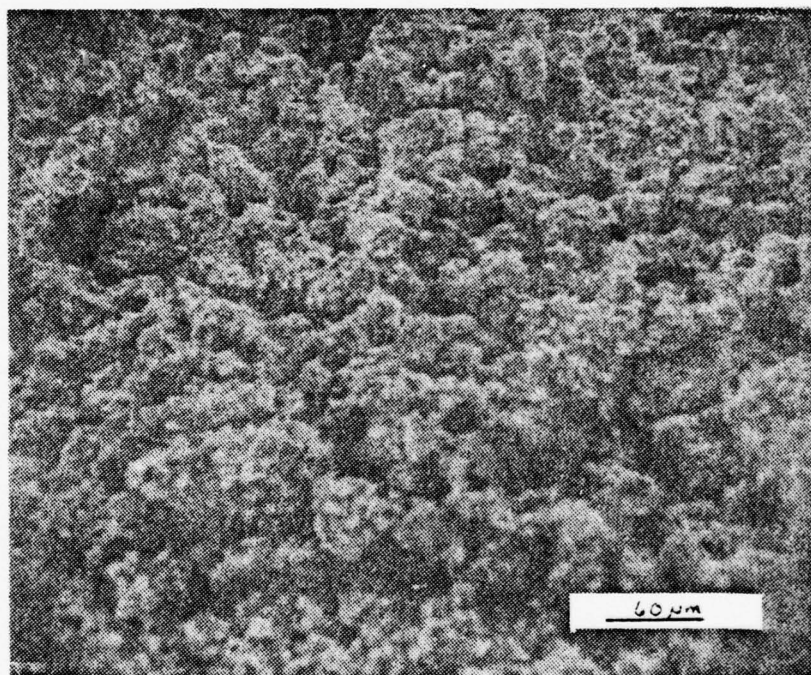
Figure 93. Early development of the coraloid near the surface of the plate in the active material. Lead-calcium PbCA#1, 40 cycles, 240X.
