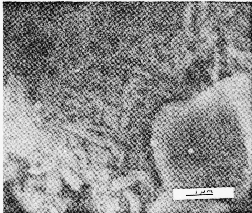
Figure 96. Area between lead-sulfate crystals near the grid. The dentic crystals are seen as increasing in number as cycling proceeds. Lead-calcium PbCA#1, 60 cycles, 12500X.
