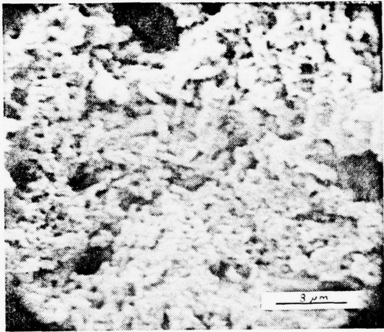
Figure 102. Active material at center of plate with little evidence of lead-sulfate being present. Lead-calcium PbCA#1, 60 cycles, 2500X.
