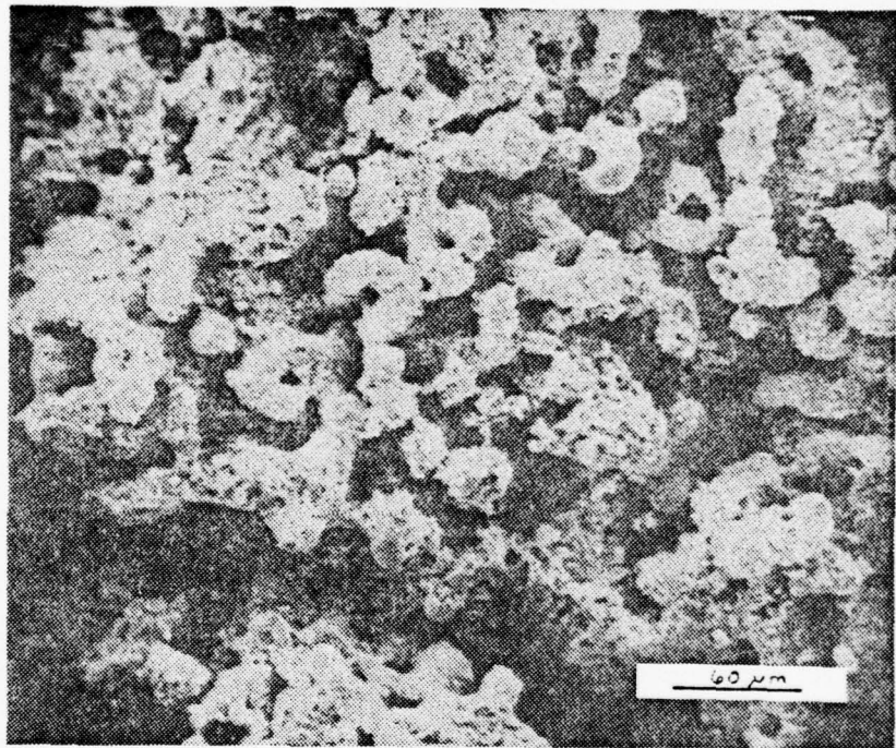
Figure 98. Coralloid structure within the active material near the surface of the photo. Lead-calcium PbCA#1, 50 cycles, 260X.
