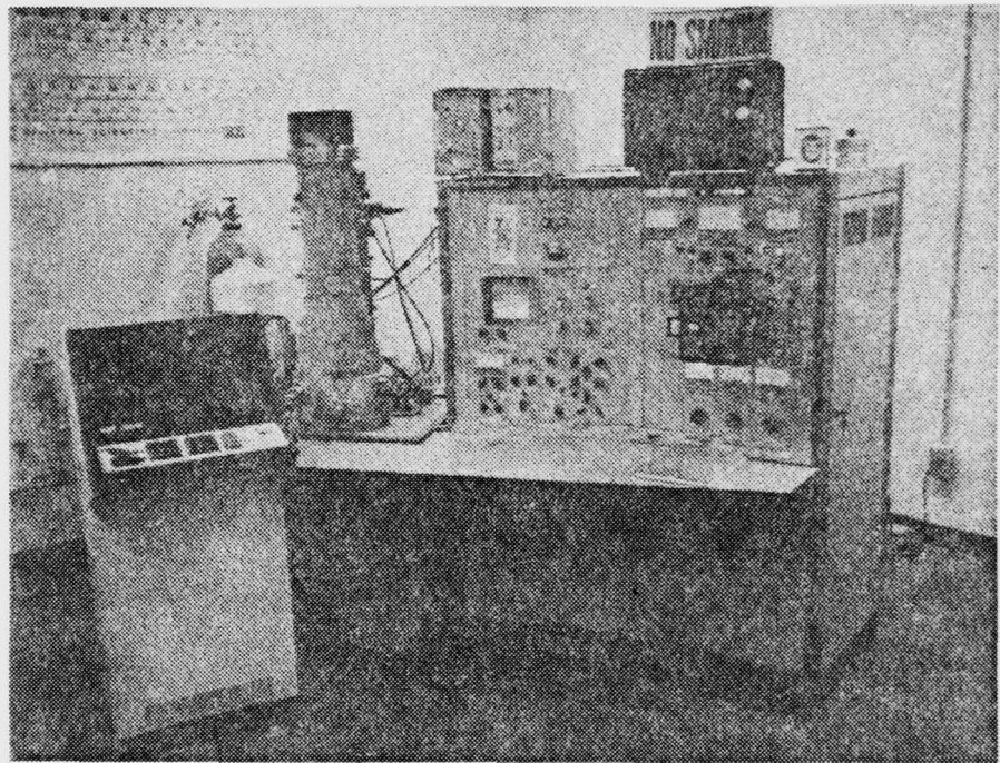
Figure 28. Cambridge Mode S4-10 scanning electron microscope (SEM).
