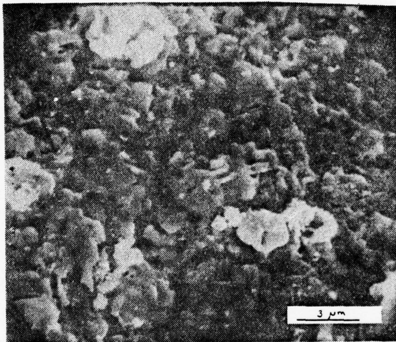
Figure 74. The clear grid surface observed by the separation of the active material from the grid. Lead-calcium PbCA#1, 0 cycles, 6000X.
