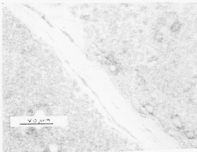
Figure 43. Optical photomicrograph of the corrosion layer of a zero cycle lead-antimony type positive plate 400X.
