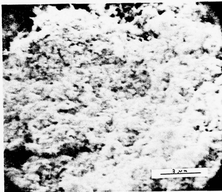
Figure 84. Active material of the outer layers of the positive plate. Lead-calcium PbCA#1, 10 cycles, 2450X.
