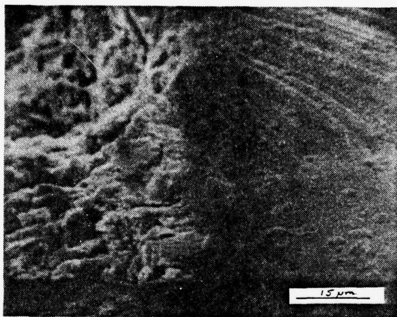
Figure 63. Interface of grid-corrosion layer - active material. The corrosion layer measures about 27 \mu\text{m} thick. Note lack of liquid-like entrapment of active material interface. Lead-antimony battery PbSb#2, 50 cycles, 1400X.
