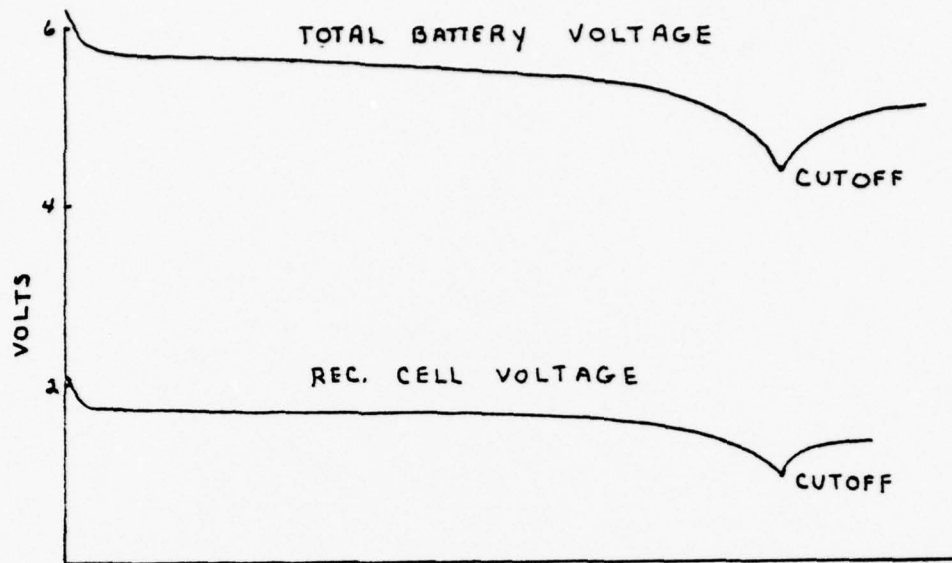
TIME LIMITING CELL DISCHARGE CURVES
