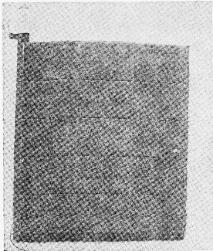
Figure 37. Positive plate of a lead-antimony grid battery at 40 cycles. The first signs of a change in the structure of the plate have occurred.
