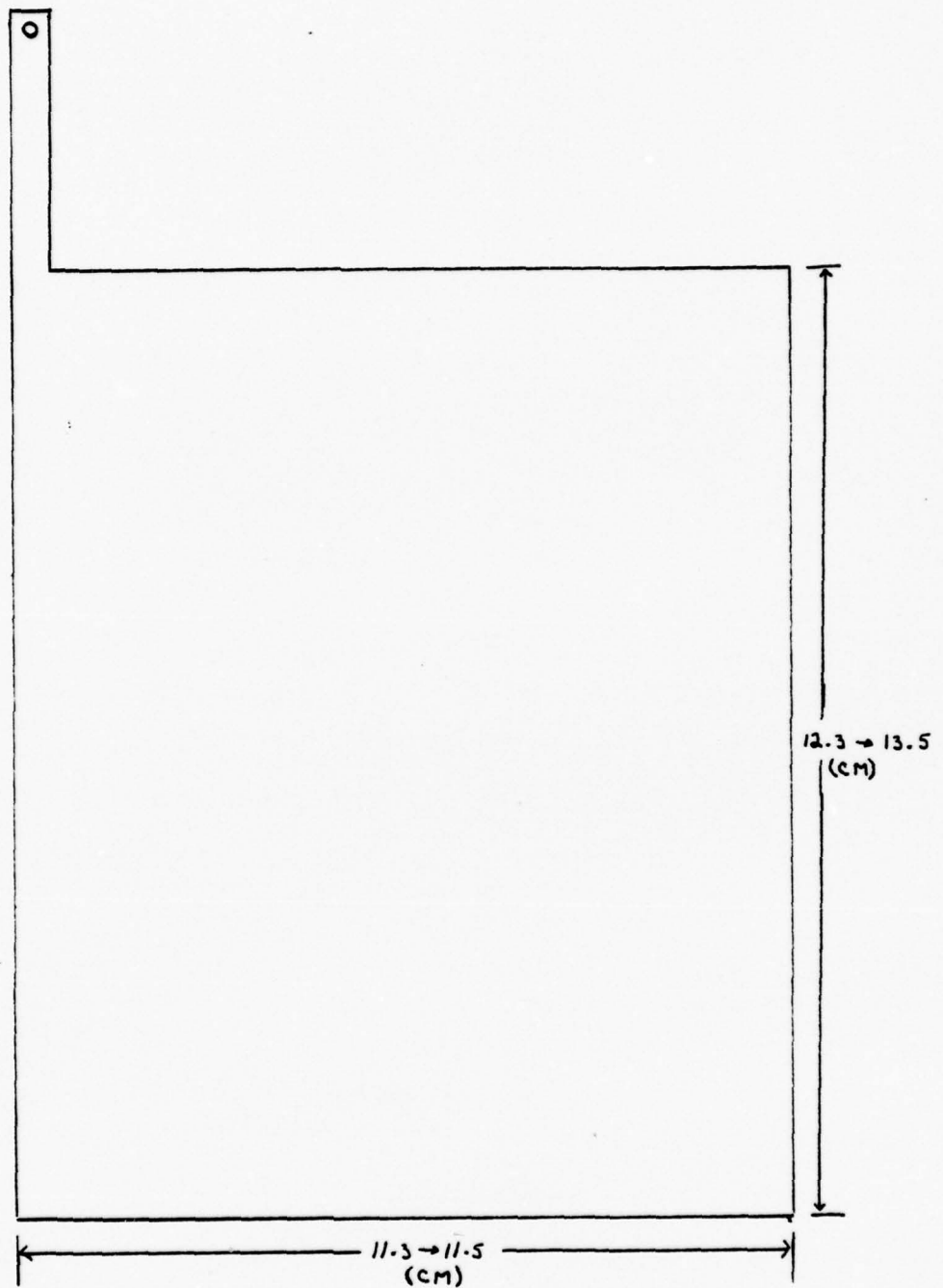
TYPICAL TEST PLATE FIGURE 13
