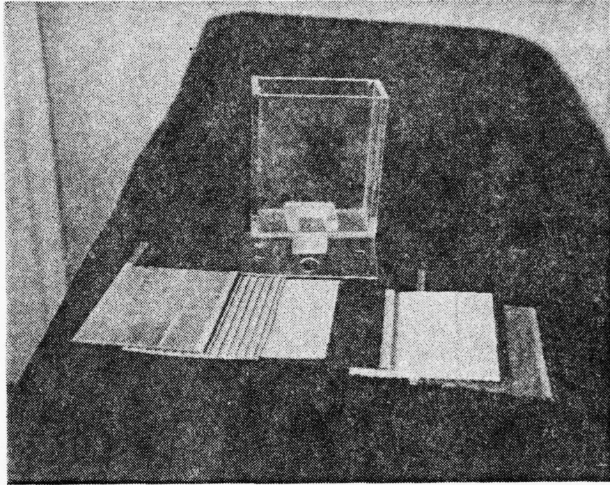
Figure 18. Typical element construction of the test cells.
