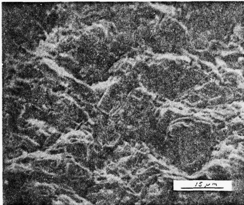
Figure 99. Lead-sulfate at the center of the active material. This layer has now begun its transformation into PbO_2 . Lead-calcium PbCA#1, 50 cycles, 1300X.
