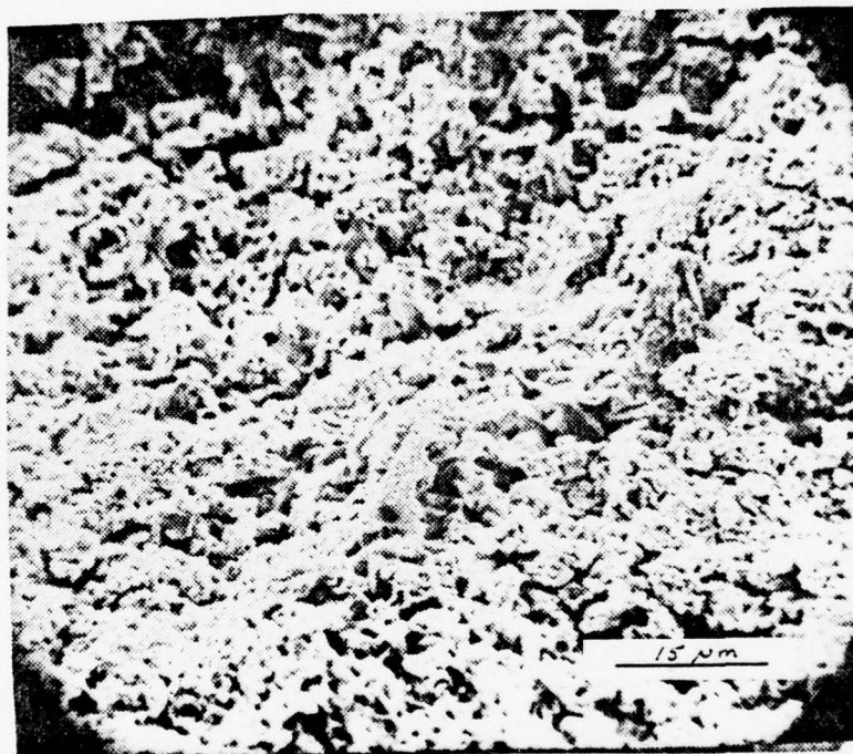
Figure 88. Active material which was bonded to the grid at the top and bottom. Lead-calcium PbCA#1, 20 cycles, 1300X.
