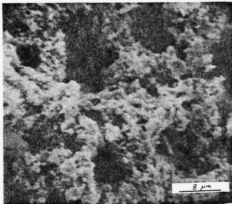
Figure 66. Surface of the coraloid structure. Lead-antimony PbSb#2, 50 cycles, 2500X.
