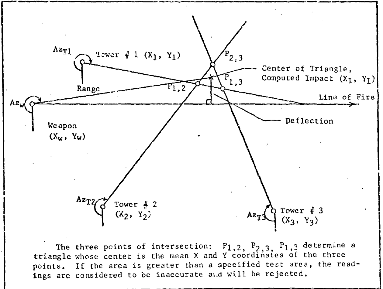
Figure 6. Three-Tower Arrangement for Determining Location of Single-Round Impact.
