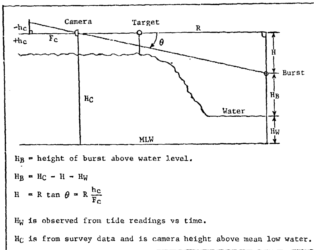
Figure 11. Measurements for Determining Relationship Between Burst Height Above Water and Above Mean Low Water.
