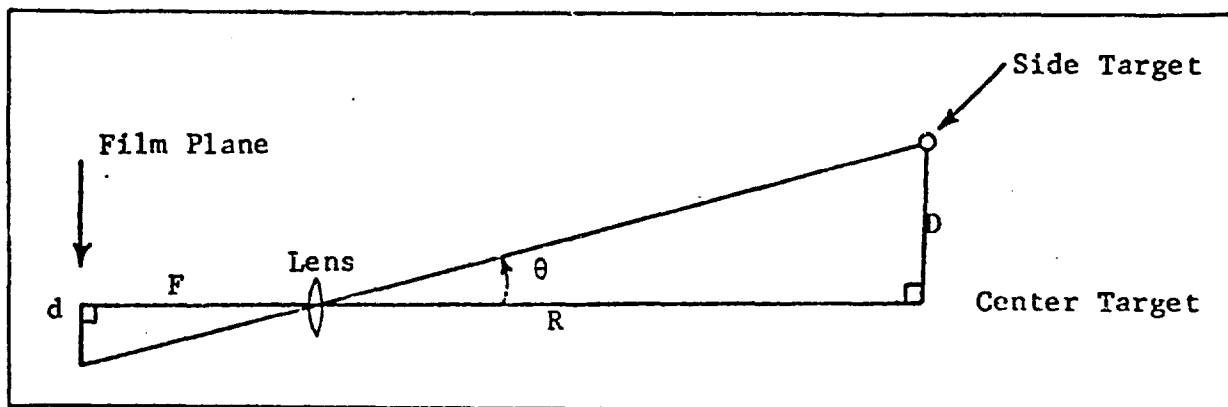
Figure 7. Method for Calculating Focal Length of Lens.
