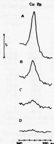
Figure 4. ESCA spectra of Cu 2p_{3/2} region for glassy carbons dipped in 10^{-4} M \text{Cu}(\text{NO}_3)_2 in acetone and rinsed with acetone. S = 3.41 kcounts/s. Smoothed spectra
