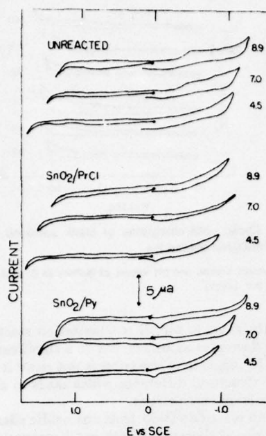
Figure 2. Cyclic voltammograms of blank solutions on unreacted \text{SnO}_2 , \text{SiO}_2/\text{PrCl} , and \text{SnO}_2/\text{Py} electrodes
