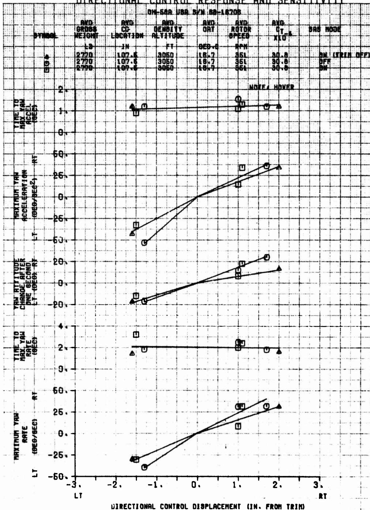
FIGURE 15 DIRECTIONAL CONTROL RESPONSE AND SENSITIVITY
