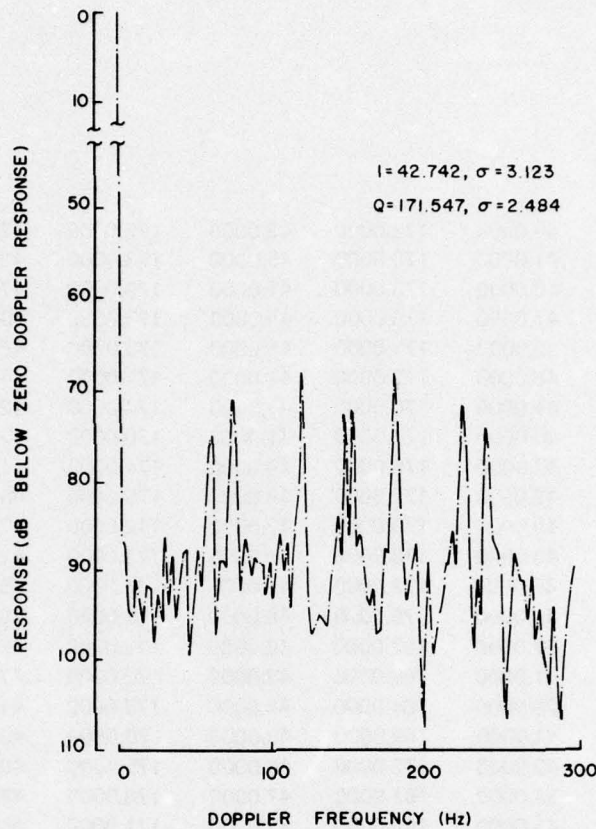
Fig. 13 — Spectral response of module 37m (transmit, 1326 MHz), computed and plotted by the computer program using the input data of Fig. 12.
