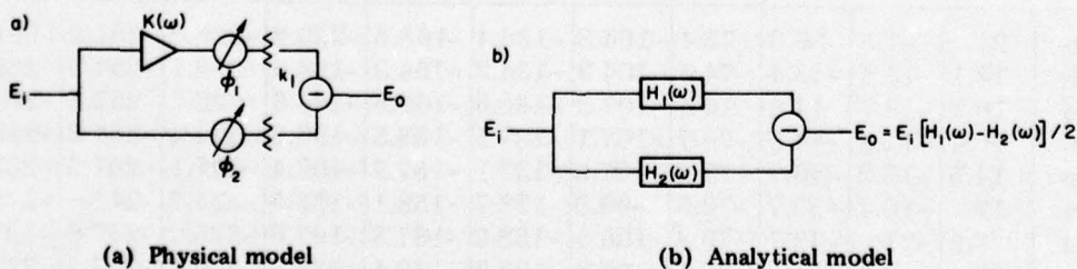
Fig. 10 — Simplified version of either Fig. 3 or Fig. 7
