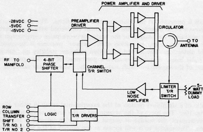
Fig. 9 - Transmit/receiver module tested
