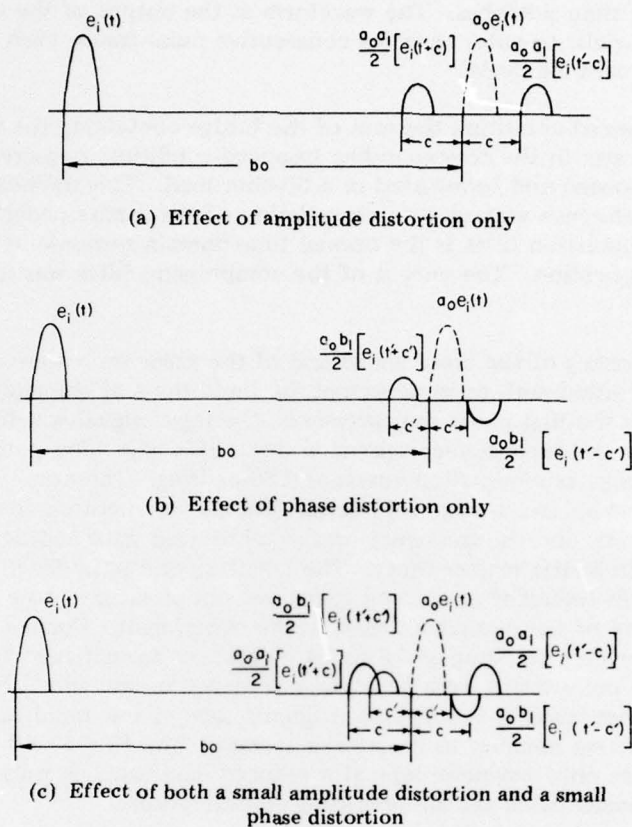
Fig. 11 — Effect of phase and amplitude distortions on the waveform at the output of the compression filter. (Because balancing of the bridge in this experiment suppresses the undistorted signal at the output of the compression line, the undistorted signal is dashed.)
