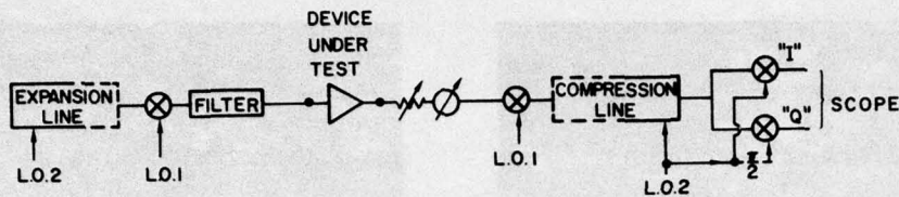
Fig. 1 — First version of the initial test setup developed at NRL
