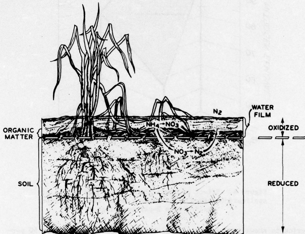
Figure 5. A schematic of conditions that would allow both aerobic and anaerobic processes to occur in an overland flow system
