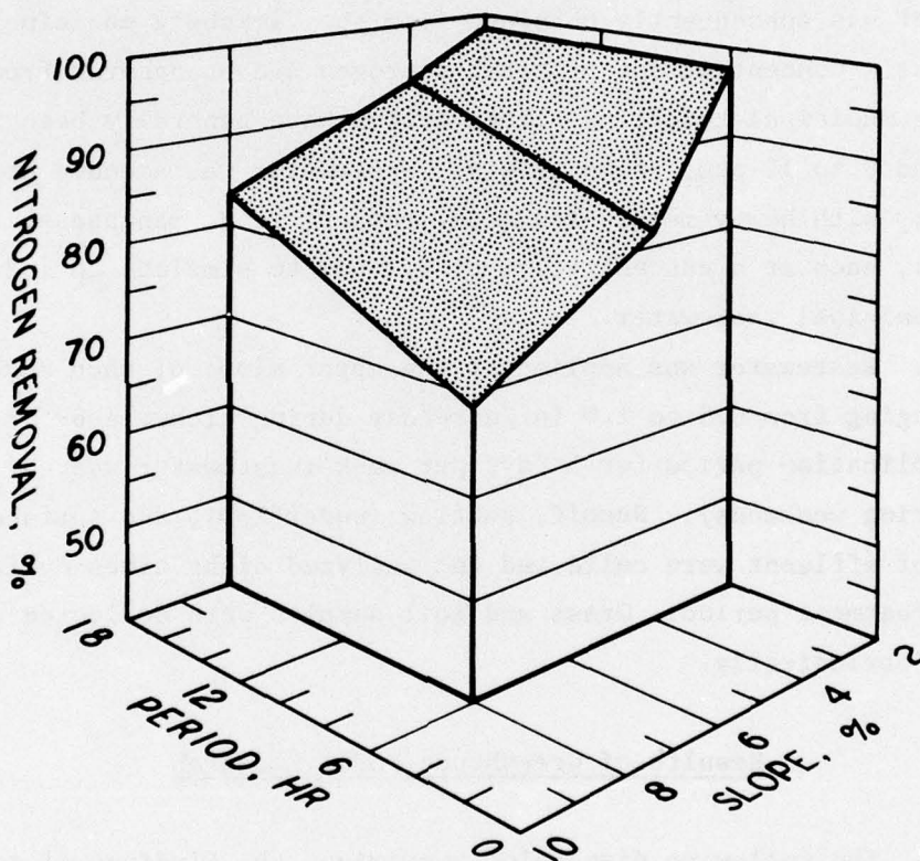
Figure 3. Effect of length of application period and slope on the efficiency of nitrogen removal from wastewater applied at a volume of 0.5 in./acre
