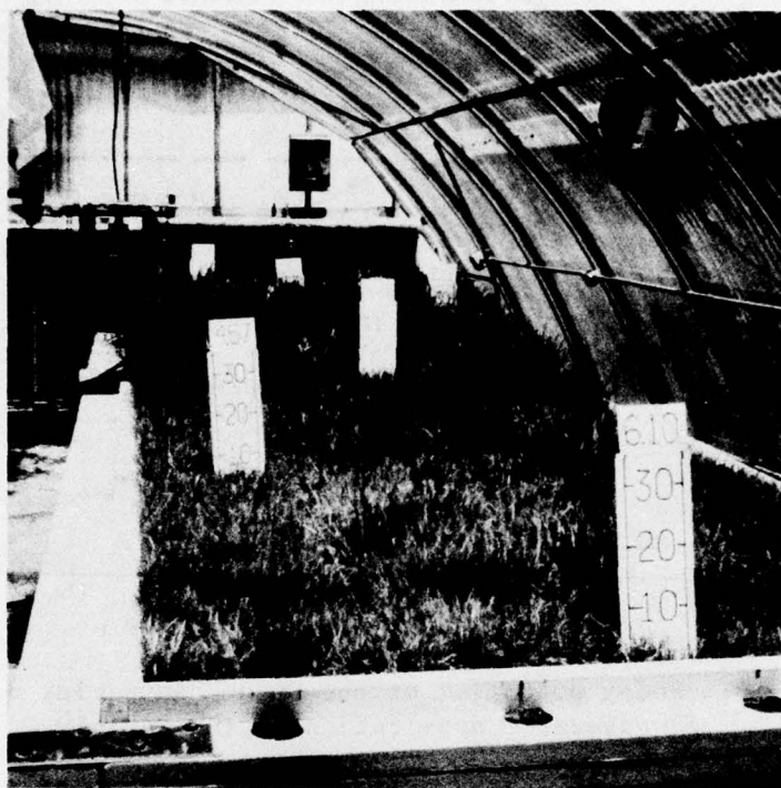
Figure 7. Wastewater model 43 days after start of treatment. Grass height reached 20 to 40 cm (7.87 to 15.74 in.) in upper 10 ft (3.05 m); practically no increase in height and zero nitrogen content in surface water beyond 15 ft (4.57 m) 10
