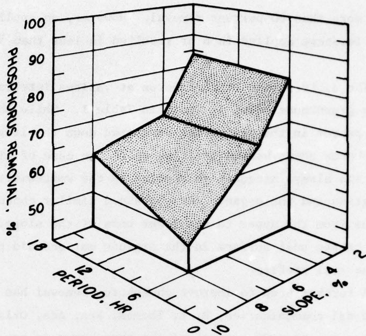
Figure 8. Effect of length of application period and slope on phosphorus removal from wastewater applied at a volume of 0.5 in./acre
