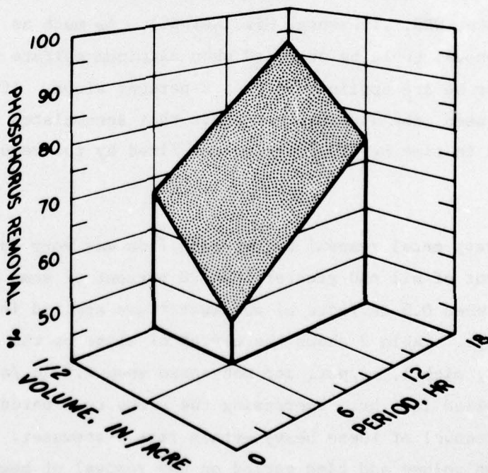
Figure 9. Effect of application volume and length of application period on phosphorus removal from wastewater applied to a 2-percent slope
