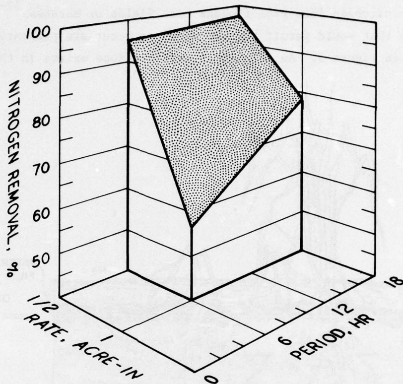
Figure 4. Effect of application volume and length of application period on nitrogen removal from wastewater applied to a 2-percent slope
