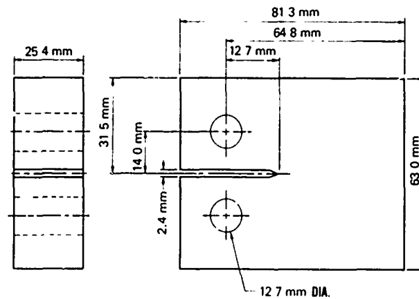
Fig. 2—Compact tension cyclic crack-growth specimen
