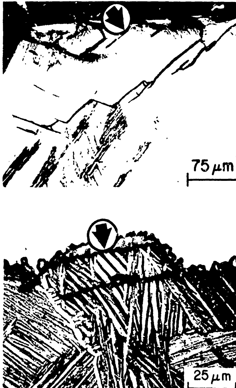
Fig. 5—Metallographic crack path section for the BA: (a) \Delta K = 17.4 MPa \cdot m 1/2 ; (b) \Delta K = 18.5 MPa \cdot m 1/2 . Arrow indicates trace of fracture surface (Cu, Ni-plated).
