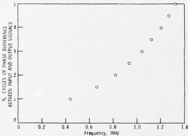
Figure 11. Cycles of phase difference versus frequency in 3-D carbon-phenolic specimen
