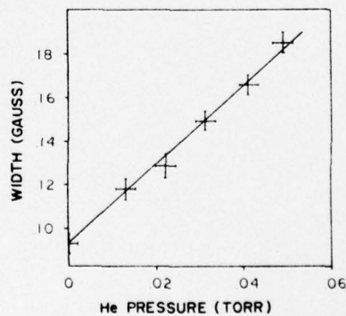
FIG. 4. Width vs helium pressure plot for the 4f^{14}6s6p^3P_1^0 levels.
