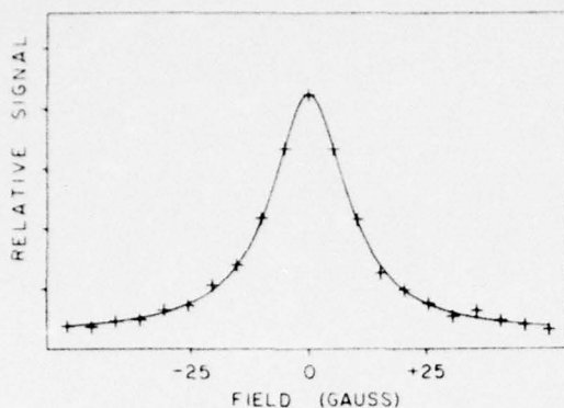
FIG. 2. Yb II Hanle signal fit with Lorentzian. The solid line is the computer fit.
