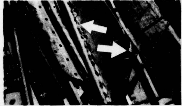
Figure 5-7. E2A Aircraft Lifting Sling Exfoliation
