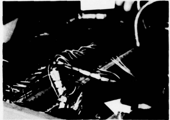
Figure 5-23. Electrical Compartment Corrosion of Terminal Strap Support Bracket
