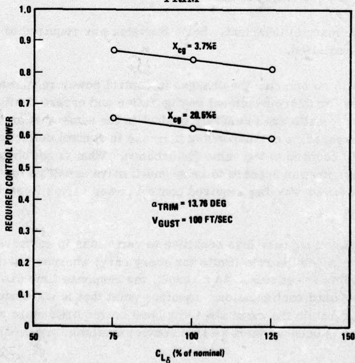
Figure 2-15. Canard Configuration, Required Control Power as a Function of Control Surface Effectiveness, \alpha_{TRIM} = 13.76 Degrees
