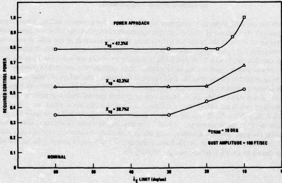
Figure 2-20. Conventional Configuration, Variation in Control Surface Rate Limit
