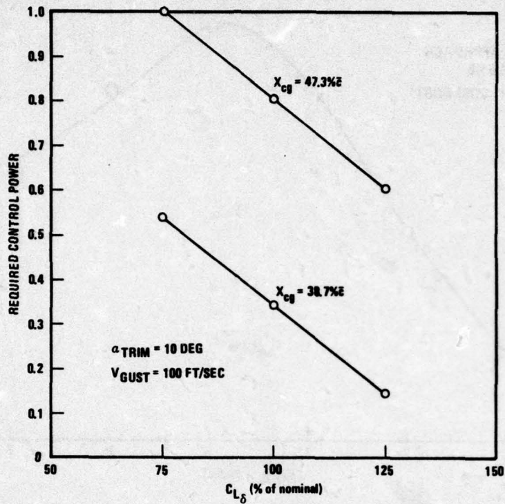
Figure 2-14. Canard Configuration, Required Control Power as a Function of Control Surface Effectiveness, \alpha_{TRIM} = 10 Degrees
