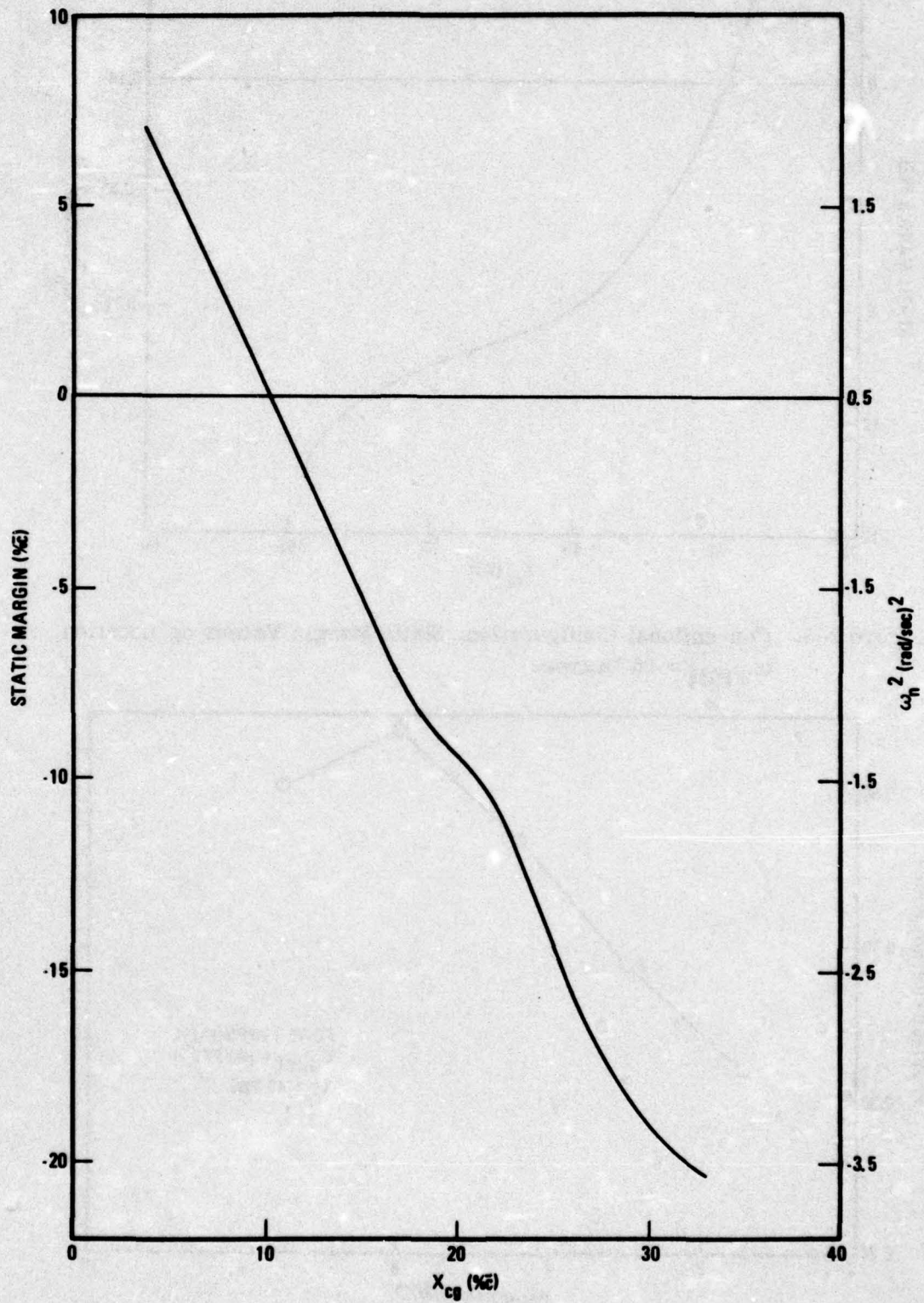
Figure 2-7. Canard Configuration, Static Margin Versus cg Location, Power Approach, \alpha_{\text{TRIM}} = 13.76 Degrees
