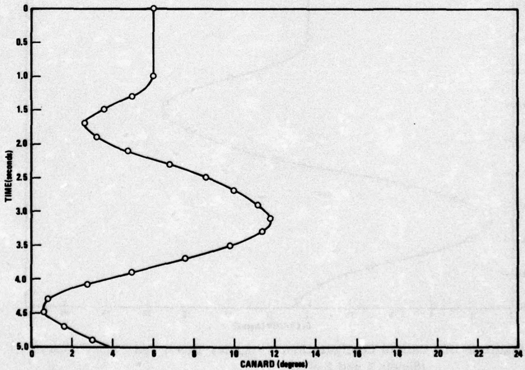
Figure 2-12. Canard Configuration, Computer-Generated Time History (Sheets 3 and 4 of 4)
