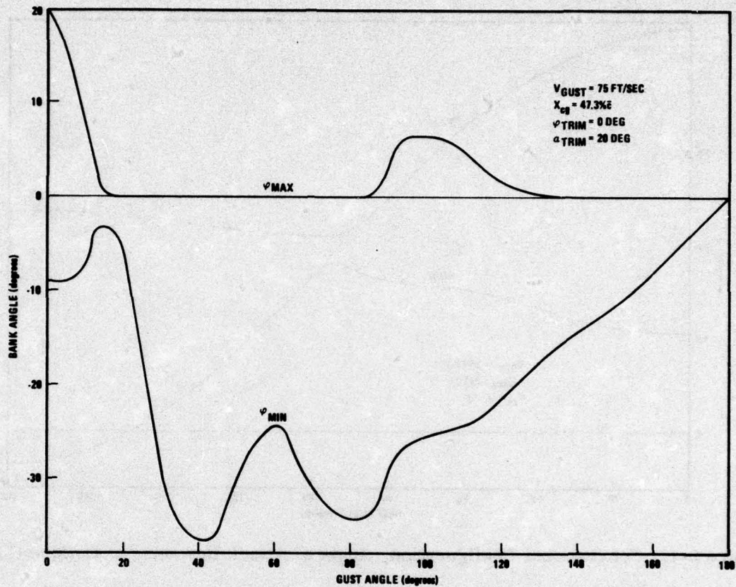
Figure 3-3. Conventional Configuration, Bank Angle Response to Oblique Gusts
