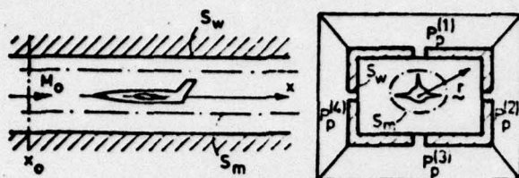
Fig. 2. Slotted test section.
