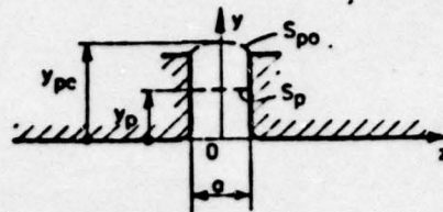
Fig. 5. Slot geometry.
