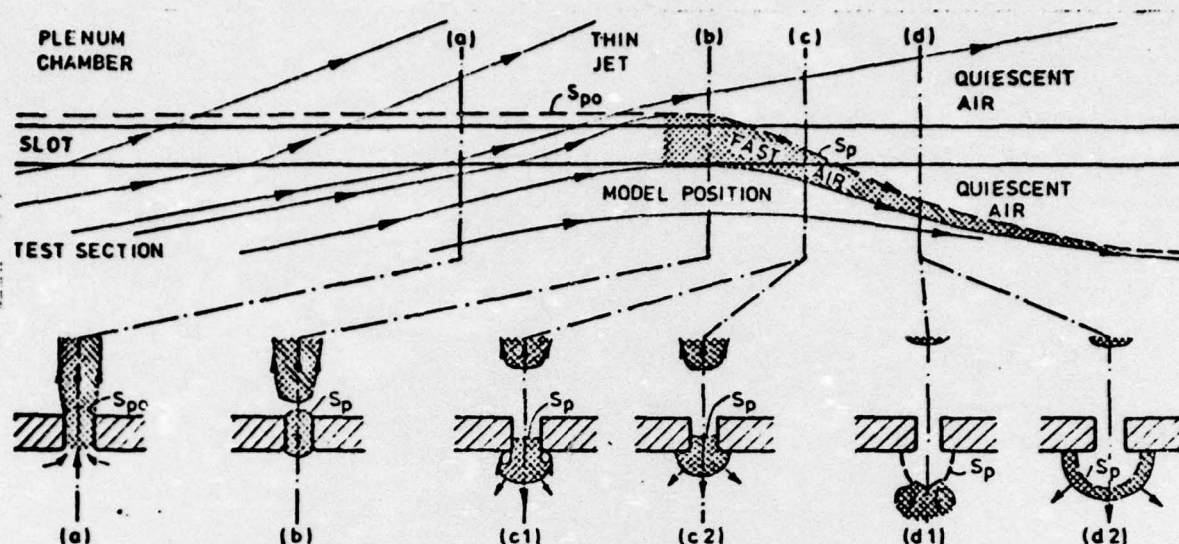
Fig. 1. Possible inviscid flow patterns (not to scale).
