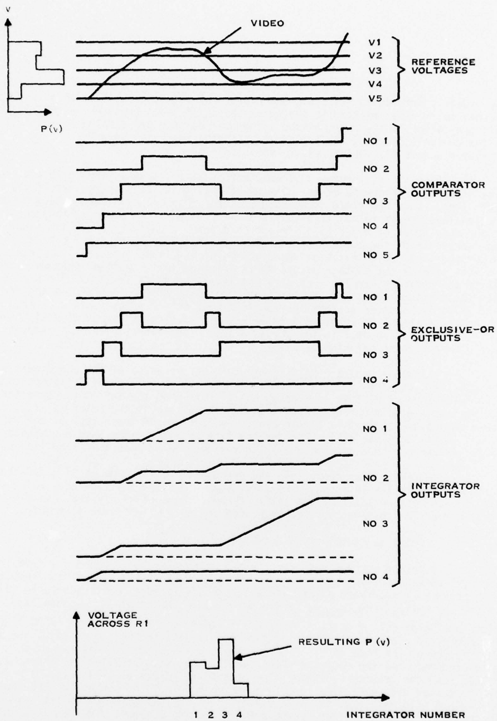
Figure 5. Typical Waveforms Dynamic Range Enhancement Scheme 1
