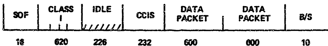
(b) OPTIMUM PACKET SIZE OF 600 BITS, BER = 10^{-4} , CONTINUOUS ARQ -- TYPE II
