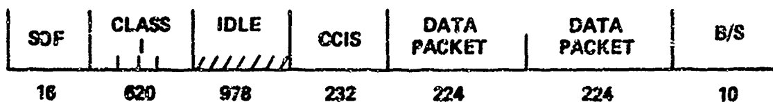
(a) OPTIMUM PACKET SIZE OF 224 BITS, BER = 10^{-3} , CONTINUOUS ARQ -- TYPE II
