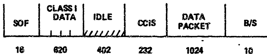
(c) SUB-OPTIMUM PACKET SIZE OF 1024 BITS, BER = 10^{-4} , CONTINUOUS ARQ -- TYPE II
