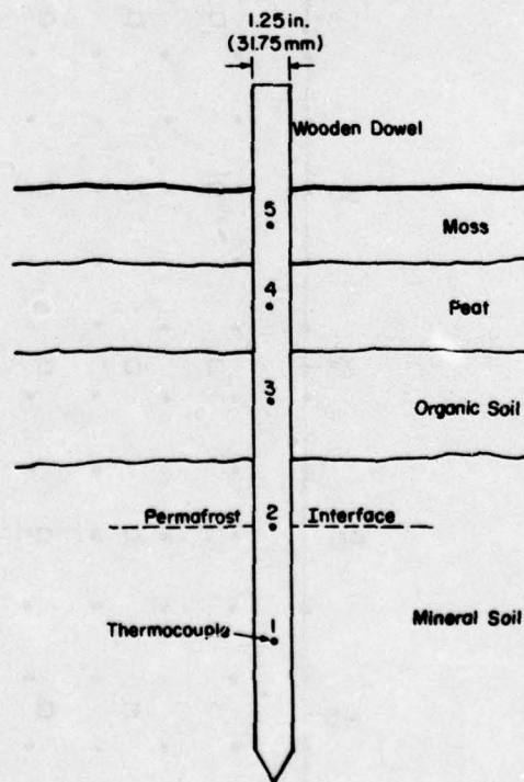
Figure 4. Thermocouple levels.
