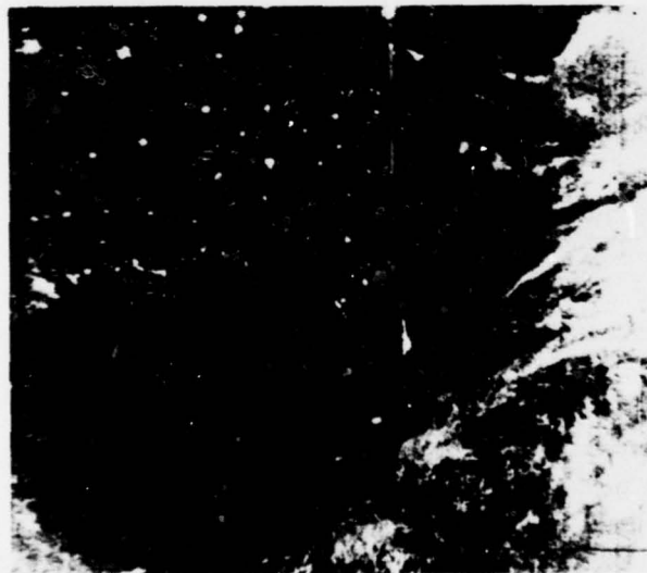
Figure 4. DMSP Satellite Photograph Recorded on 23 May 1973 During Partial Moonlit Conditions Showing Clouds. The photo shows the continental outline of the United States East Coast and Gulf Coast. Squall line activity can be identified by lightning streaks at top center of the photograph
