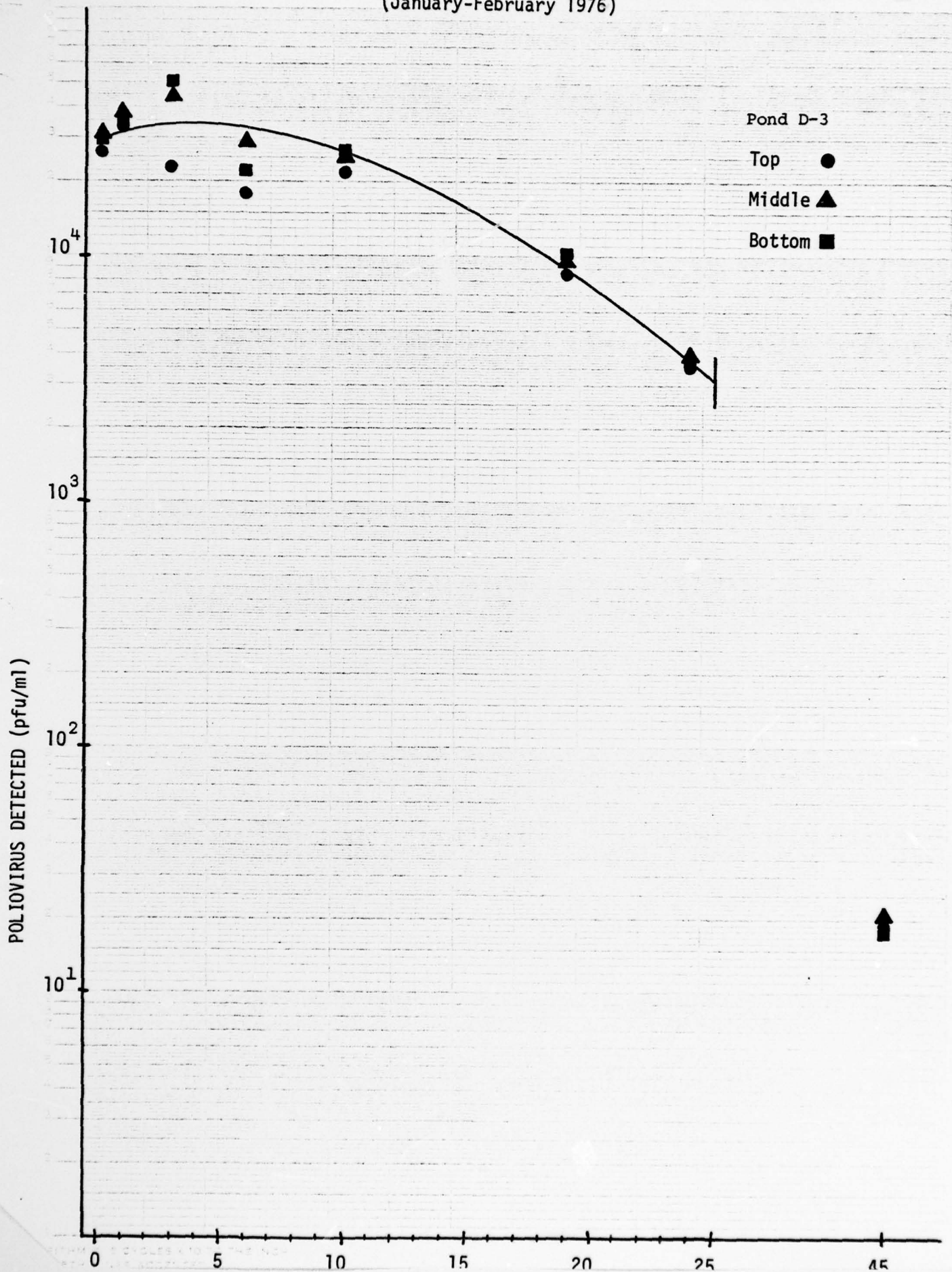
FIGURE 11. POLIOVIRUS SURVIVAL IN 90-INCH DEEP FINAL EFFLUENT POND (January-February 1976) - 19 -
