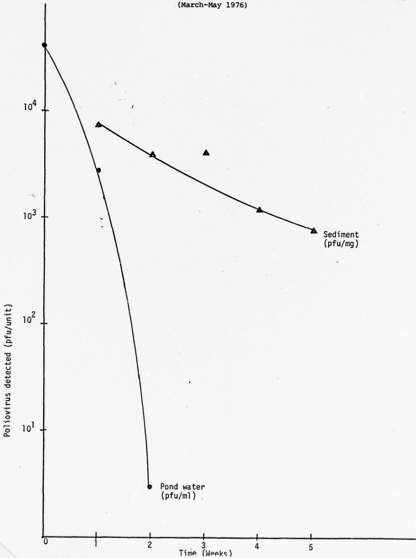
FIGURE 13. POLIOVIRUS SURVIVAL IN 30-INCH DEEP FINAL EFFLUENT POND (March-May 1976)
