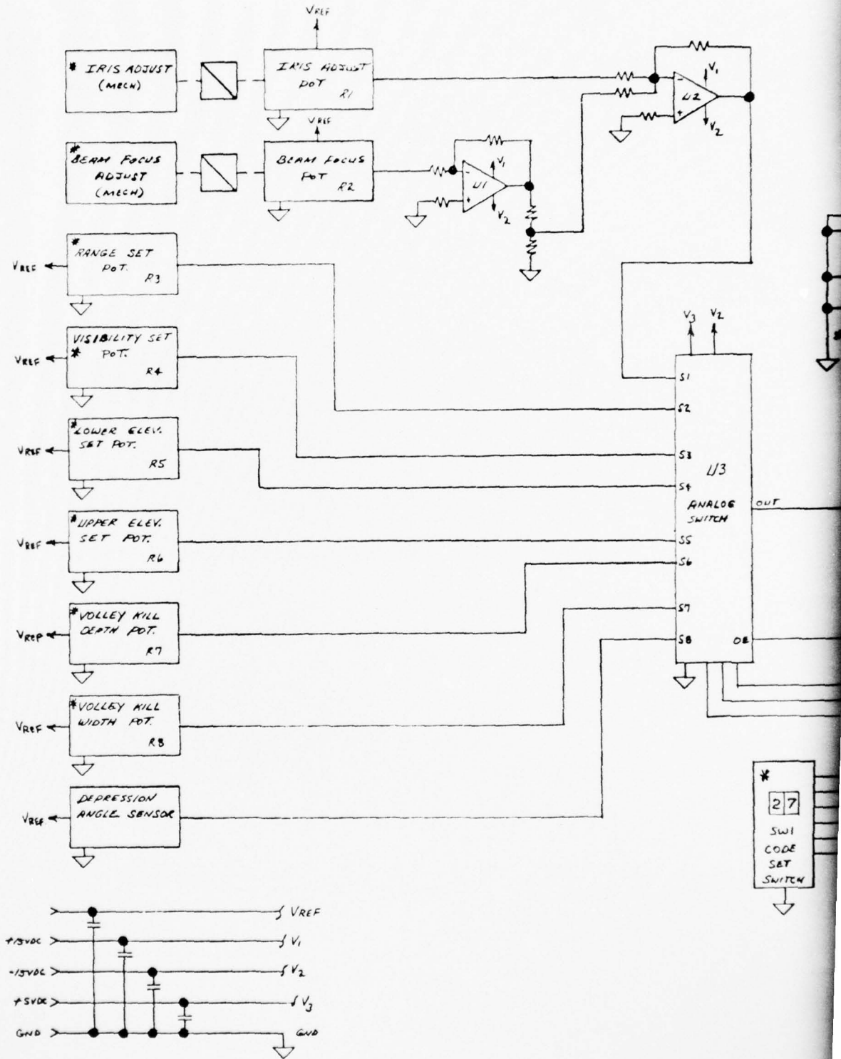
Figure C-9. Controls and Input Interf (Indirect/Area Fire Simulator System)
