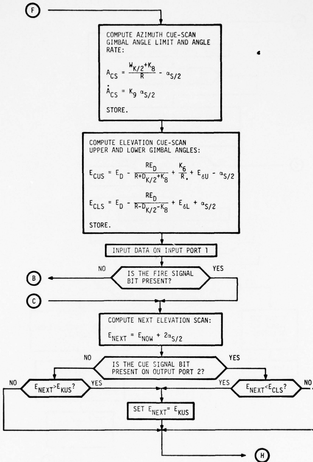
Figure C-12. Program Flow to be Implemented (Cont'd)
