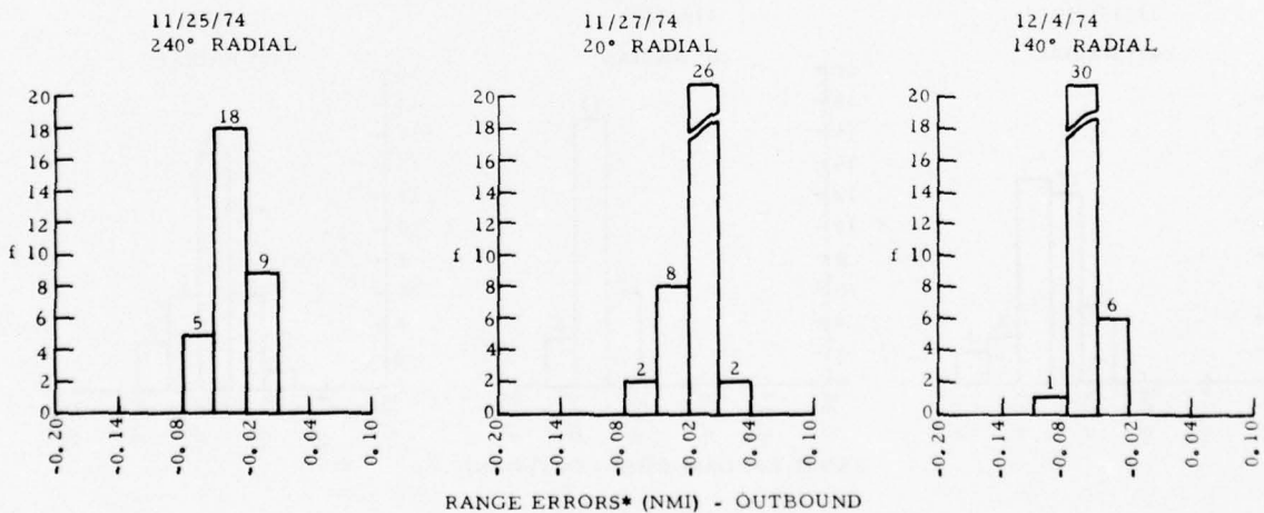
RANGE ERRORS * (NMI) - OUTBOUND
