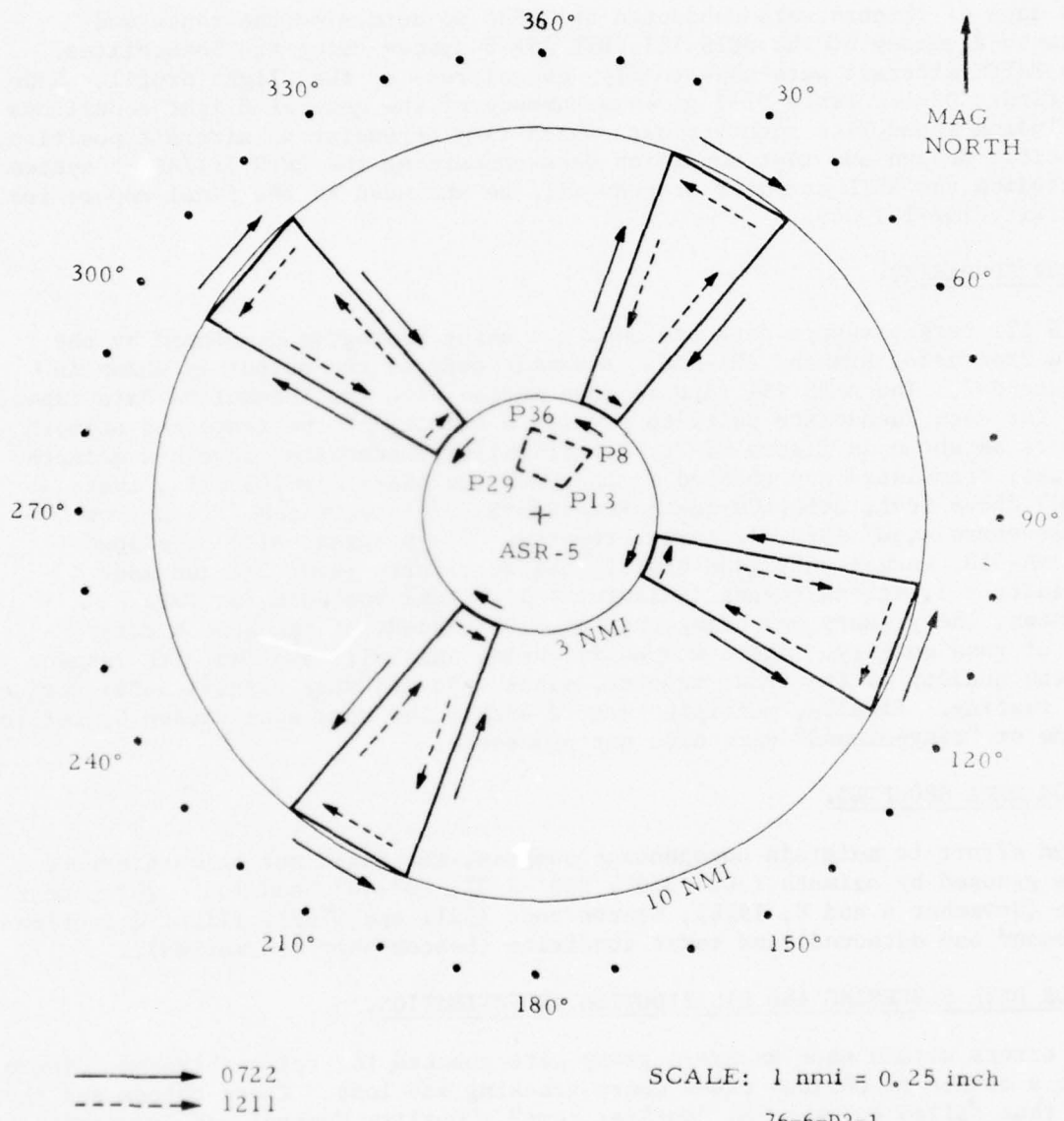
FIGURE D2-1. FLIGHT PROFILES (THEODOLITE)
