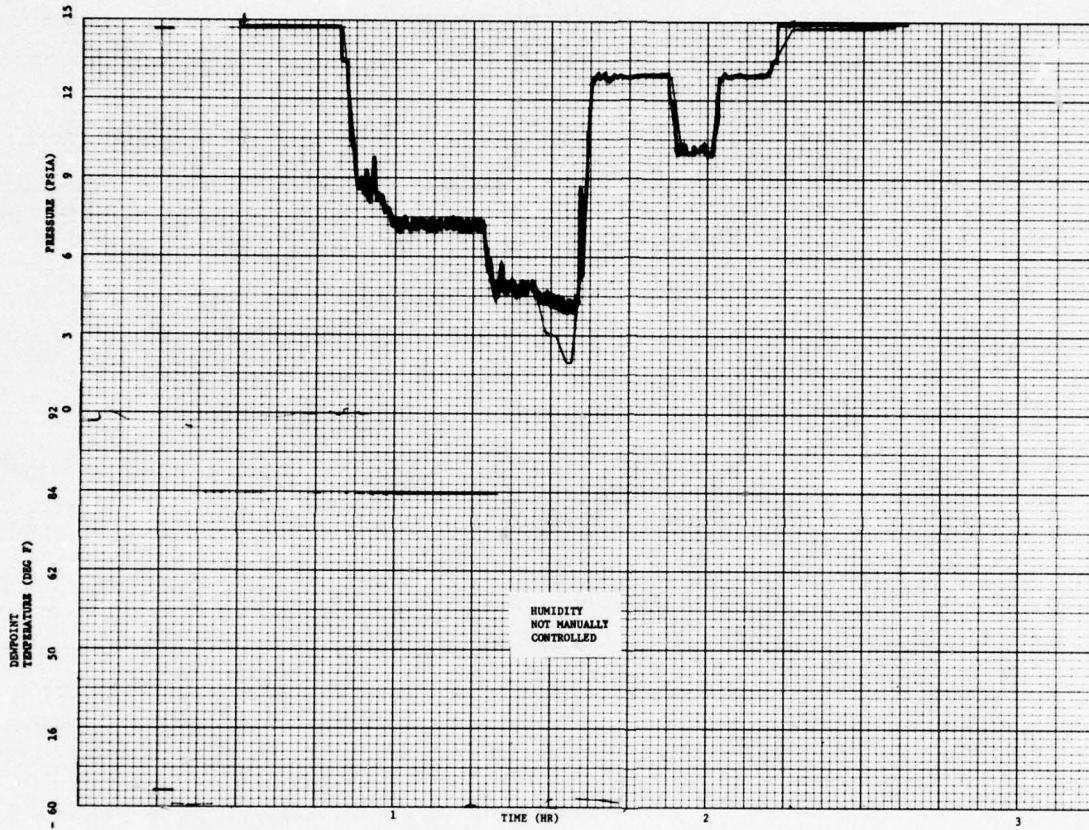
Figure 12. Manual Control of a Pressure (Altitude) Profile
