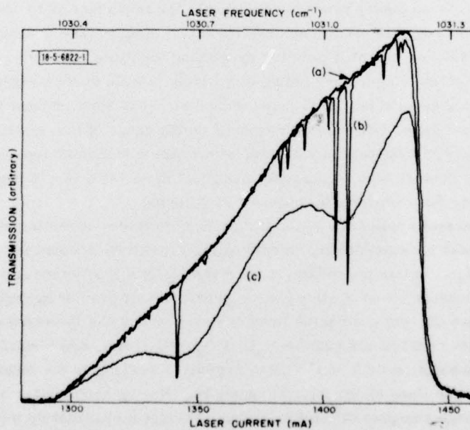
Fig. II-2. Laser spectroscopy of C_2H_4 using diode laser operating CW at 77^\circ K (liquid-nitrogen-cooled). Trace (a) is for the evacuated cell, (b) for 1 Torr C_2H_4 , and (c) for 13,200 ppm C_2H_4 in air at atmospheric pressure. Cell length = 30 cm.
