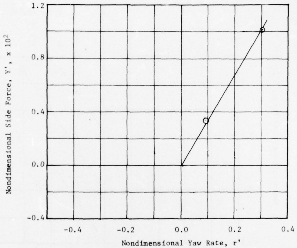
Figure 167 - Variation of Nondimensional Side Force with Nondimensional Yaw Rate for a Drift Angle of 0 Degrees at a Full Scale Speed of 10 Knots for the Spade Rudder at Deep Draft
