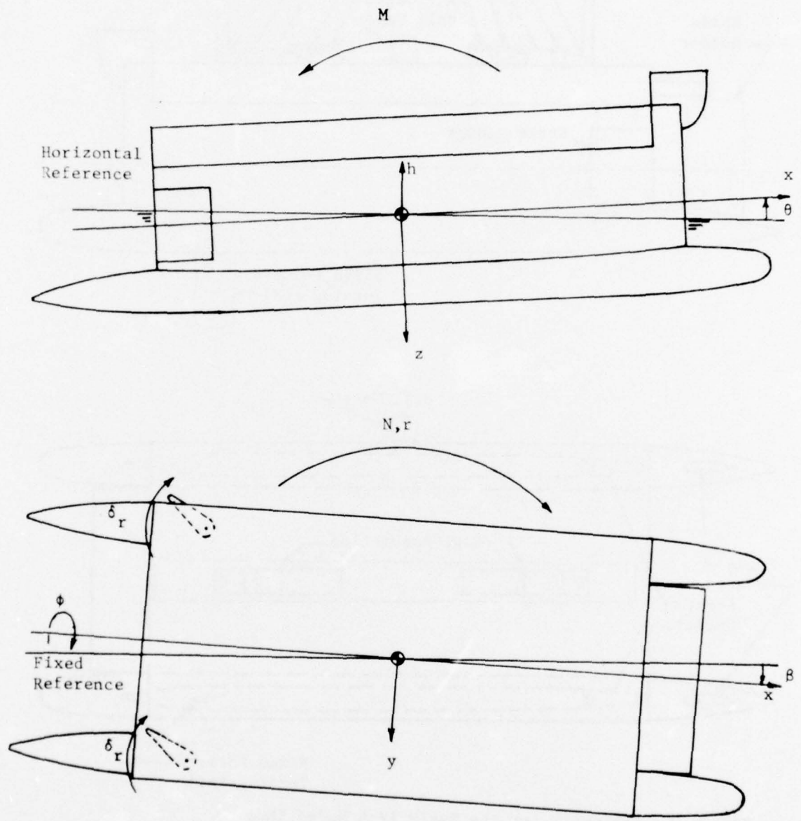
Figure 1 - Schematic Indicating Coordinate Systems and Positive Directions of Measured Values
