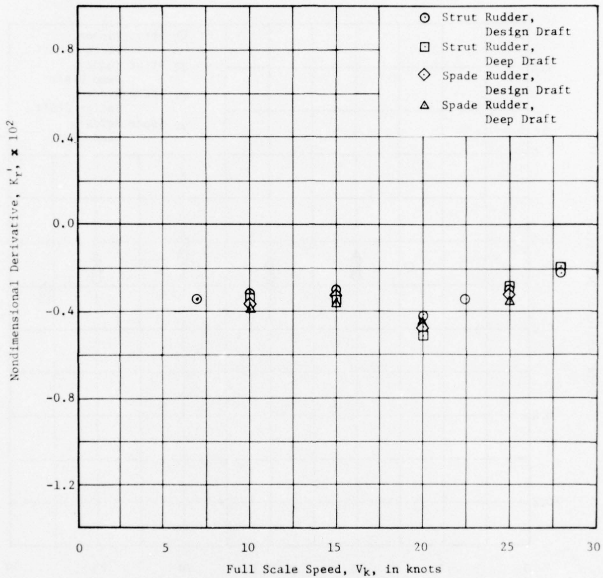
Figure 17 - Variation of Nondimensional Derivative, K_R^i , with Full Scale Speed for a Series of Rudder and Draft Configurations
