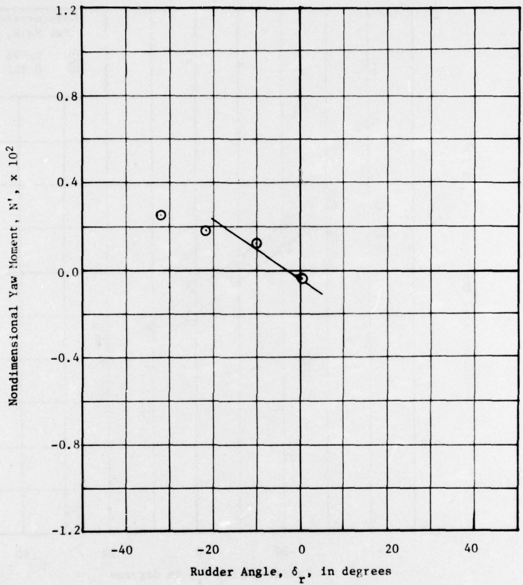
Figure 135 - Variation of Nondimensional Yaw Moment with Rudder Angle for a Nondimensional Yaw Rate of 0.093 at a Full Scale Speed of 5 Knots for the Spade Rudder at Design Draft
