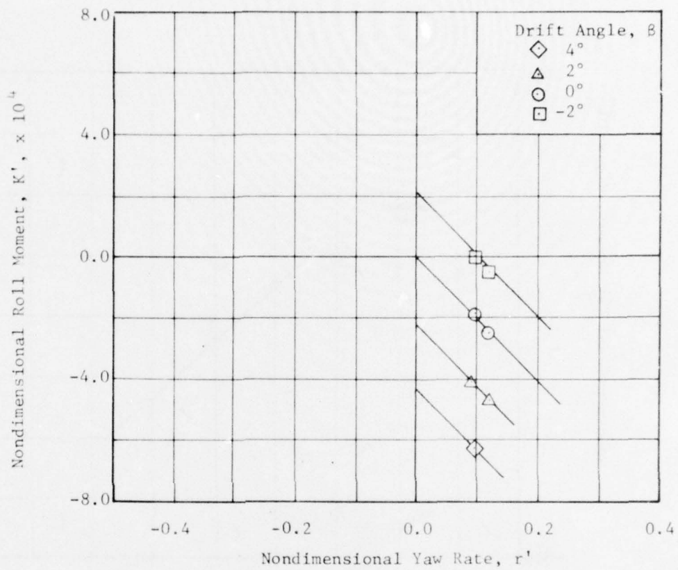
Figure 100 - Variation of Nondimensional Roll Moment with Nondimensional Yaw Rate for a Series of Drift Angles at a Full Scale Speed of 28 Knots for the Strut Rudder at Deep Draft
