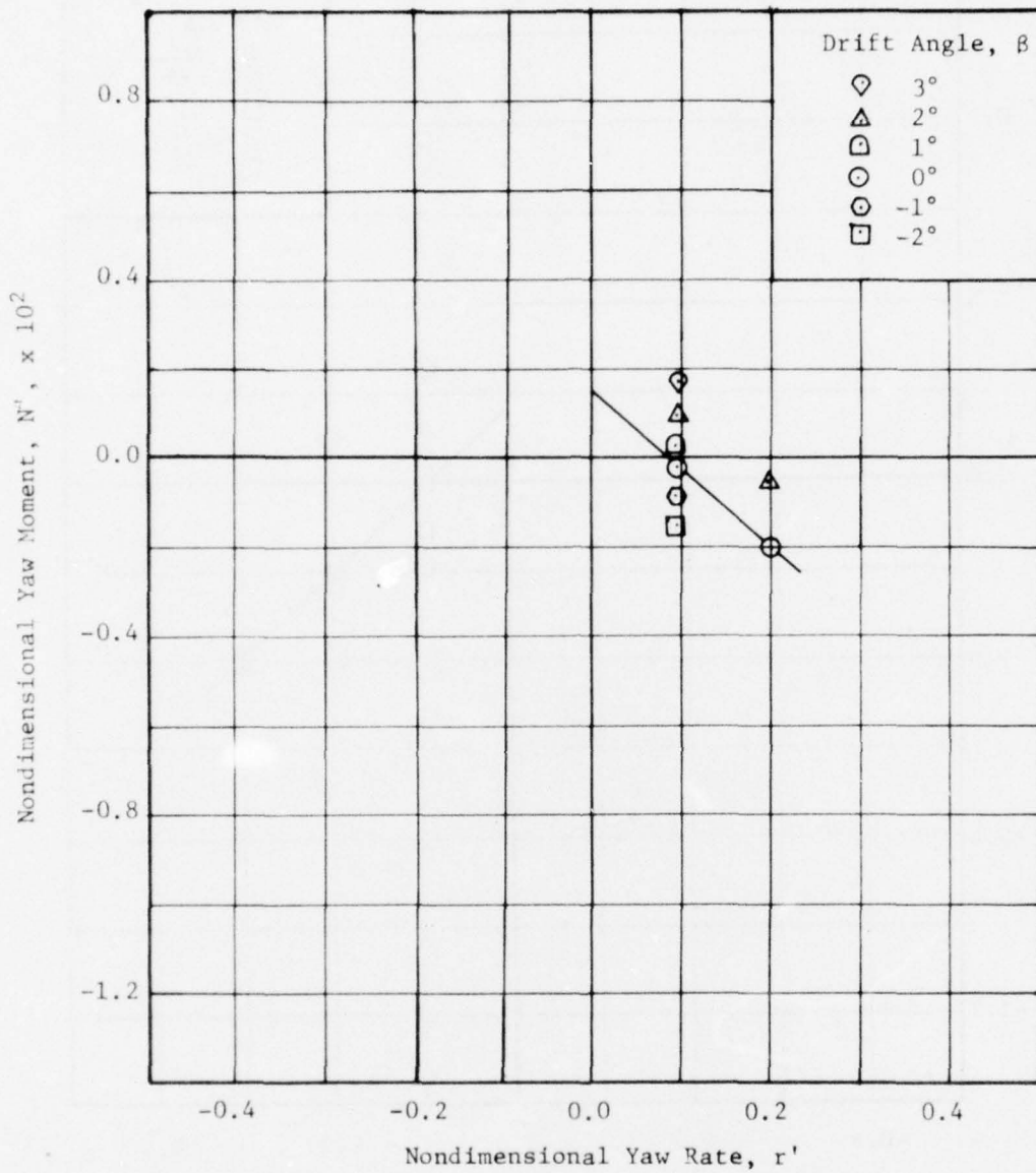
Figure 196 - Variation of Nondimensional Yaw Moment with Nondimensional Yaw Rate for a Series of Drift Angles at a Full Scale Speed of 28 Knots for the Fixed Forward Turning Foil
