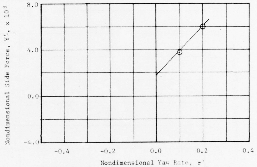
Figure 215 - Variation of Nondimensional Side Force with Nondimensional Yaw Rate for a Drift Angle of 0 Degrees at a Full Scale Speed of 5 Knots for the Half-Size Fixed Forward Turning Foil
