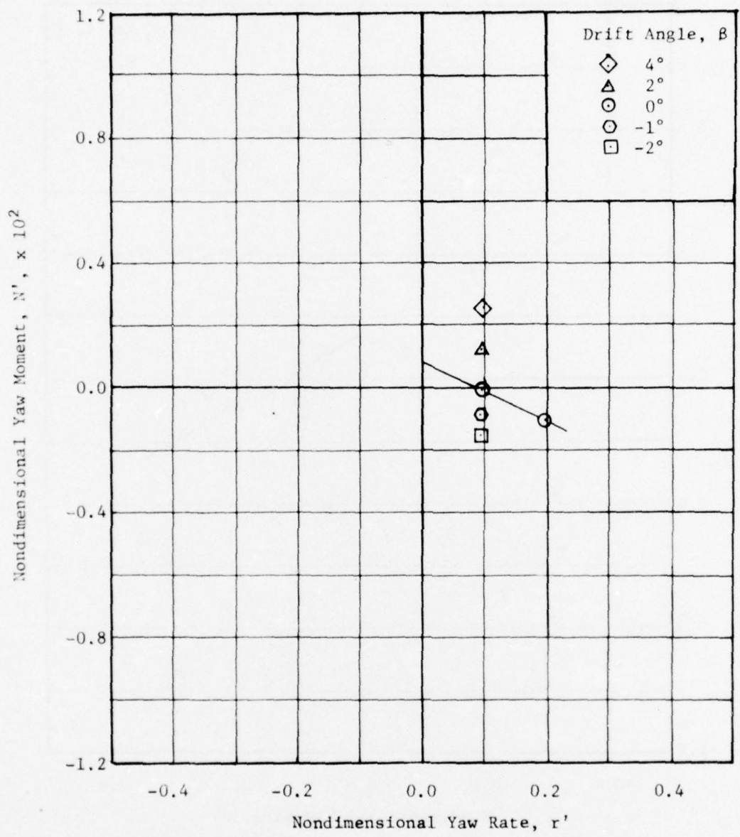
Figure 192 - Variation of Nondimensional Yaw Moment with Nondimensional Yaw Rate for a Series of Drift Angles at a Full Scale Speed of 10 Knots for the Fixed Forward Turning Foil
