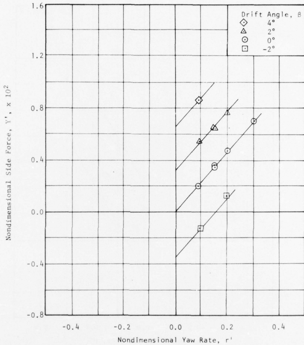
Figure 127 - Variation of Nondimensional Side Force with Nondimensional Yaw Rate for a Series of Drift Angles at a Full Scale Speed of 15 Knots for the Spade Rudder at Design Draft
