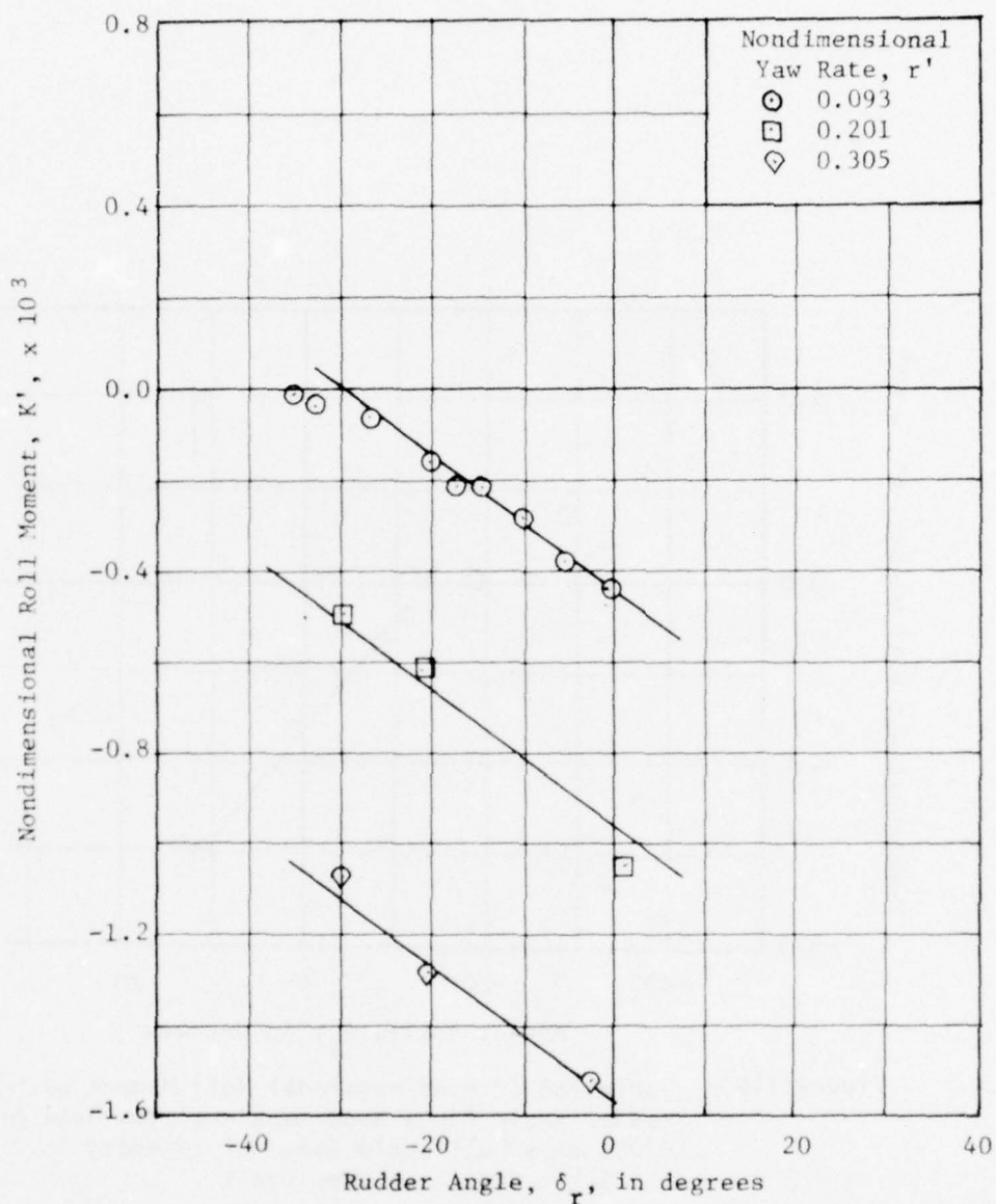
Figure 111 - Variation of Nondimensional Roll Moment with Rudder Angle for a Series of Nondimensional Yaw Rates at a Full Scale Speed of 20 Knots for the Strut Rudder at Deep Draft
