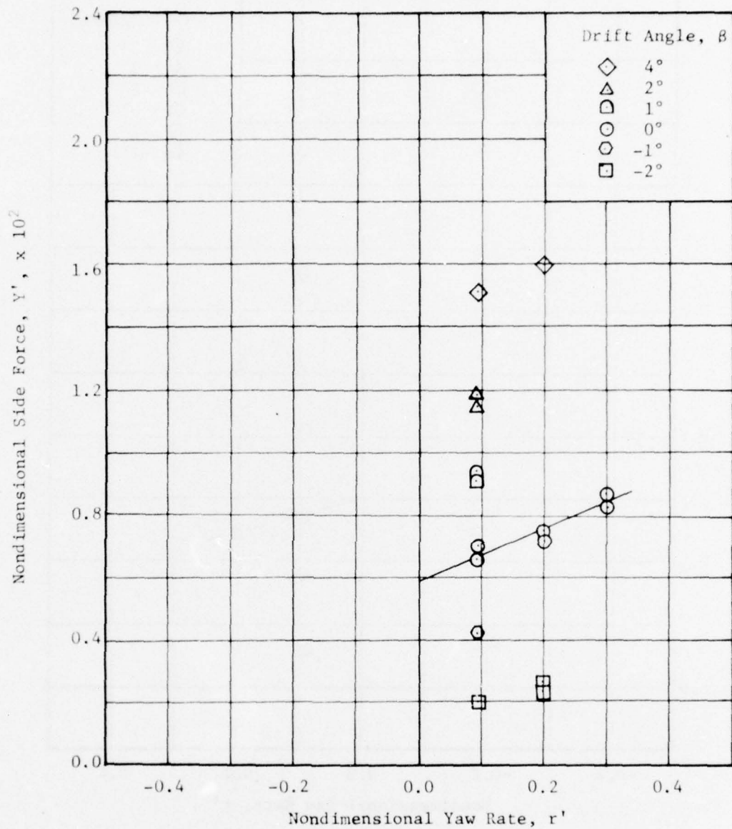
Figure 201 - Variation of Nondimensional Side Force with Nondimensional Yaw Rate for a Series of Drift Angles at a Full Scale Speed of 25 Knots for the Fixed Forward Turning Foil
