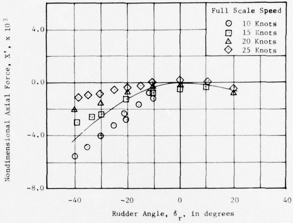
Figure 83 - Variation of Nondimensional Axial Force with Rudder Angle for a Series of Full Scale Speeds at a Nondimensional Yaw Rate of 0.093 for the Strut Rudder at Design Draft
