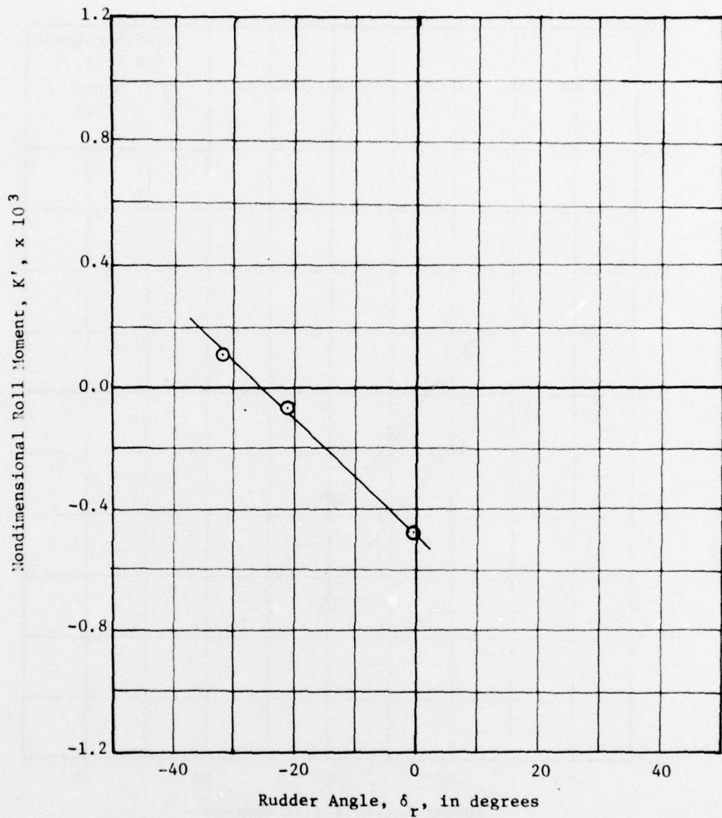
Figure 147 - Variation of Nondimensional Roll Moment with Rudder Angle for a Nondimensional Yaw rate of 0.093 at a Full Scale Speed of 5 Knots for the Spade Rudder at Design Draft
