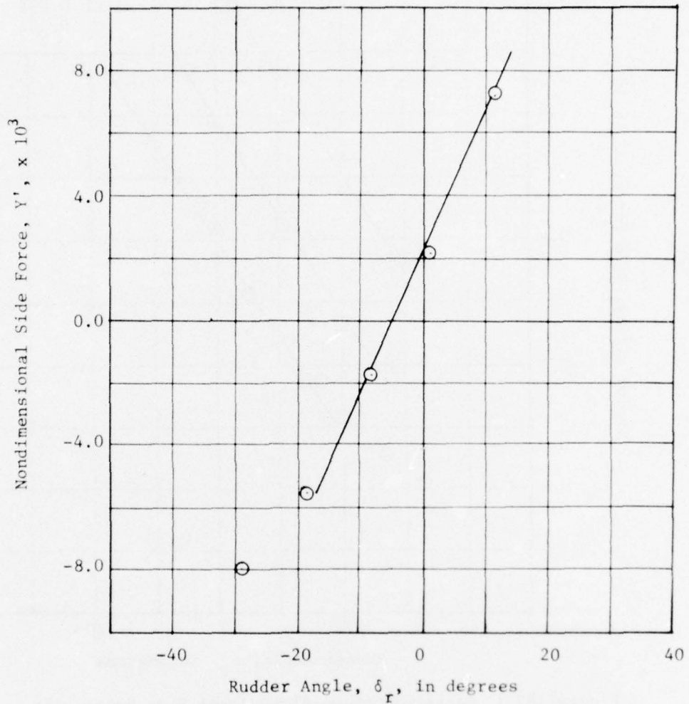
Figure 106 - Variation of Nondimensional Side Force with Rudder Angle for a Nondimensional Yaw Rate of 0.093 at a Full Scale Speed of 15 Knots for the Strut Rudder at Deep Draft
