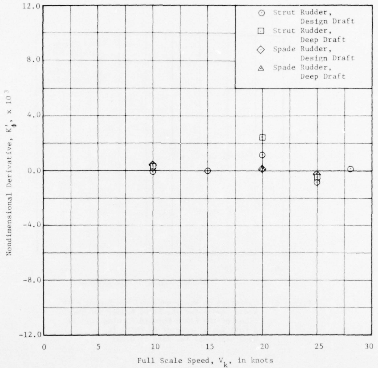
Figure 26 - Variation of Nondimensional Derivative, K'_\phi , with Full Scale Speed for a Series of Rudder and Draft Configurations
