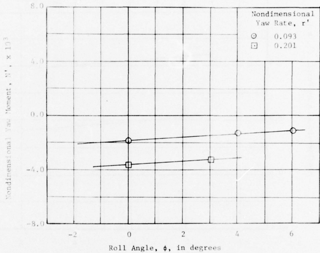
Figure 185 - Variation of Nondimensional Yaw Moment with Roll Angle for Two Nondimensional Yaw Rates at a Full Scale Speed of 25 Knots for the Spade Rudder at Deep Draft
